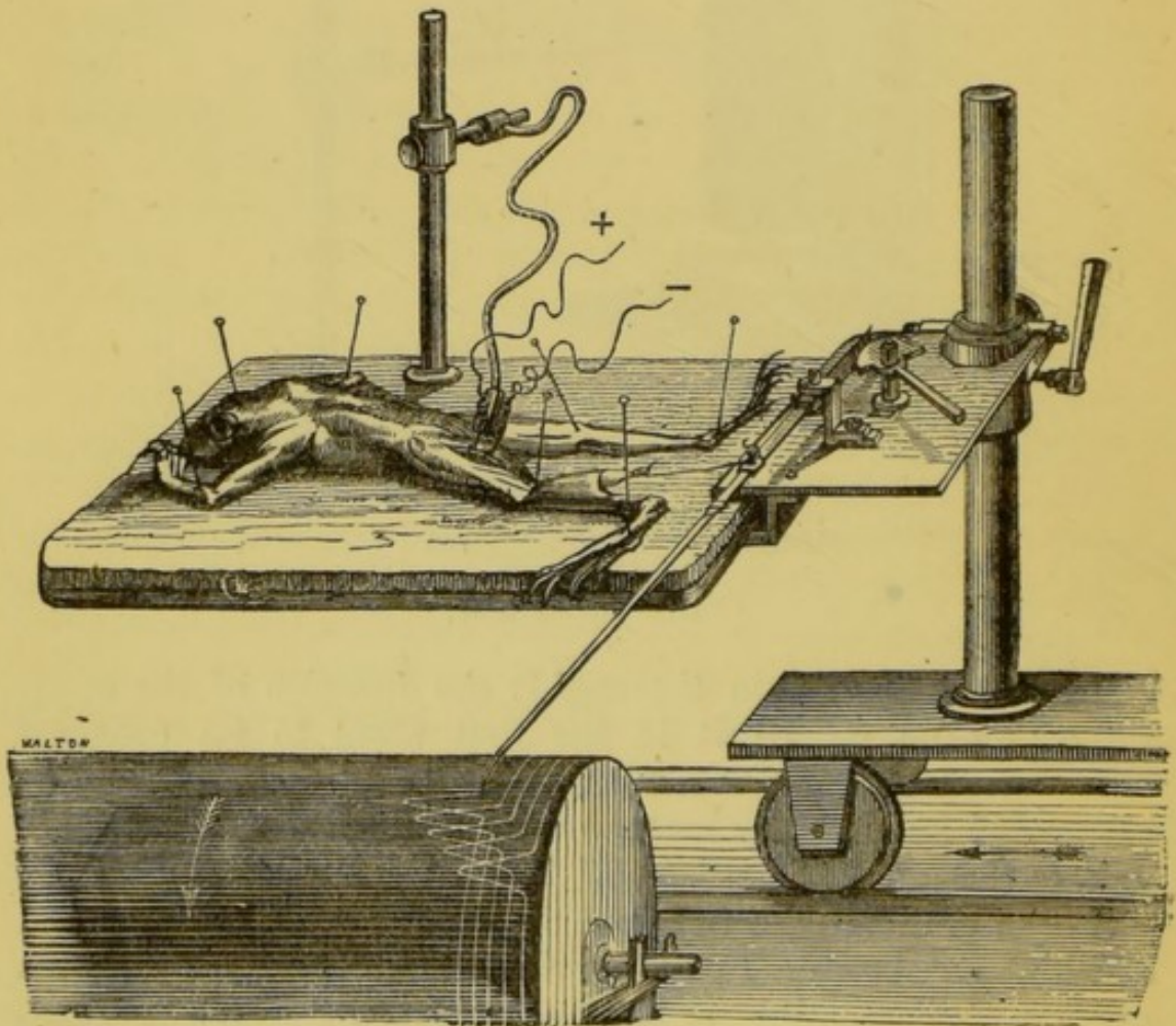
FIG. 3.—Marey's Myograph.
