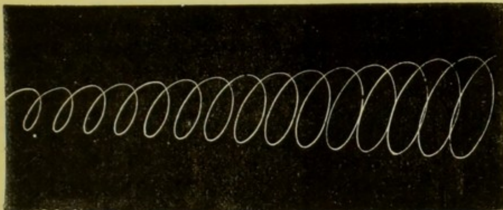
FIG. 101.—Ellipse formed by a Wheatstone's rod tuned in unison, and tracing on a revolving cylinder.
