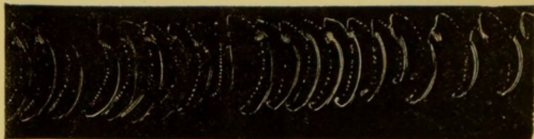
FIG. 77.—Tracing obtained with the wing of a bee, oscillating in a plane which is sensibly tangential to the generatrix of the registering cylinders.
