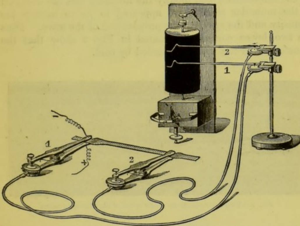
FIG. 7.—Disposition of a bundle of muscle between two pairs of myographical clips. Clip No. 1 holds the electric excitators of the muscle. A wave is represented at the moment when it has just crossed each of the clips.
