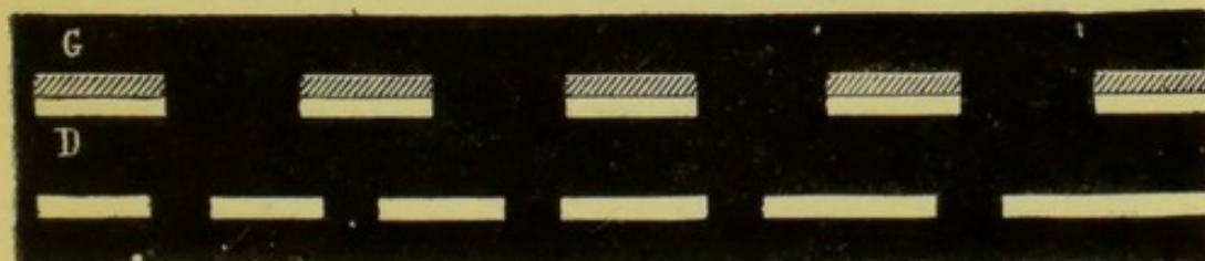
FIG. 37.—(Upper line), notation of a series of jumps on two feet. (Lower line), notation of hops on right foot. It is seen that there is constancy in the durations of suspension, notwithstanding the variability of the pressures.
