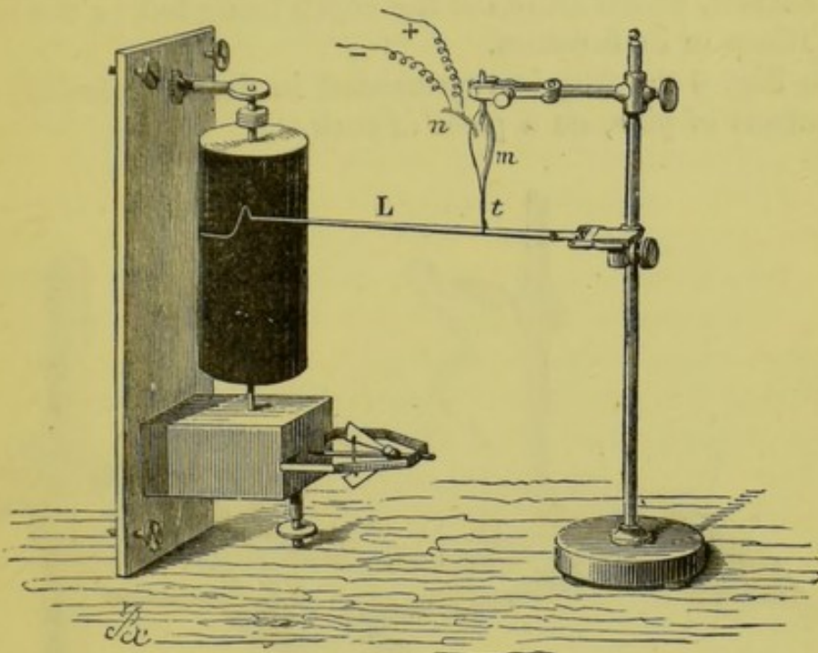
FIG. 2.—The Myograph.
