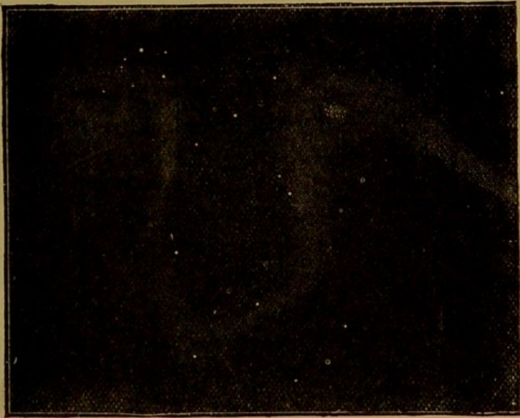
Fig. 9.—The Shield of Sobieski.
