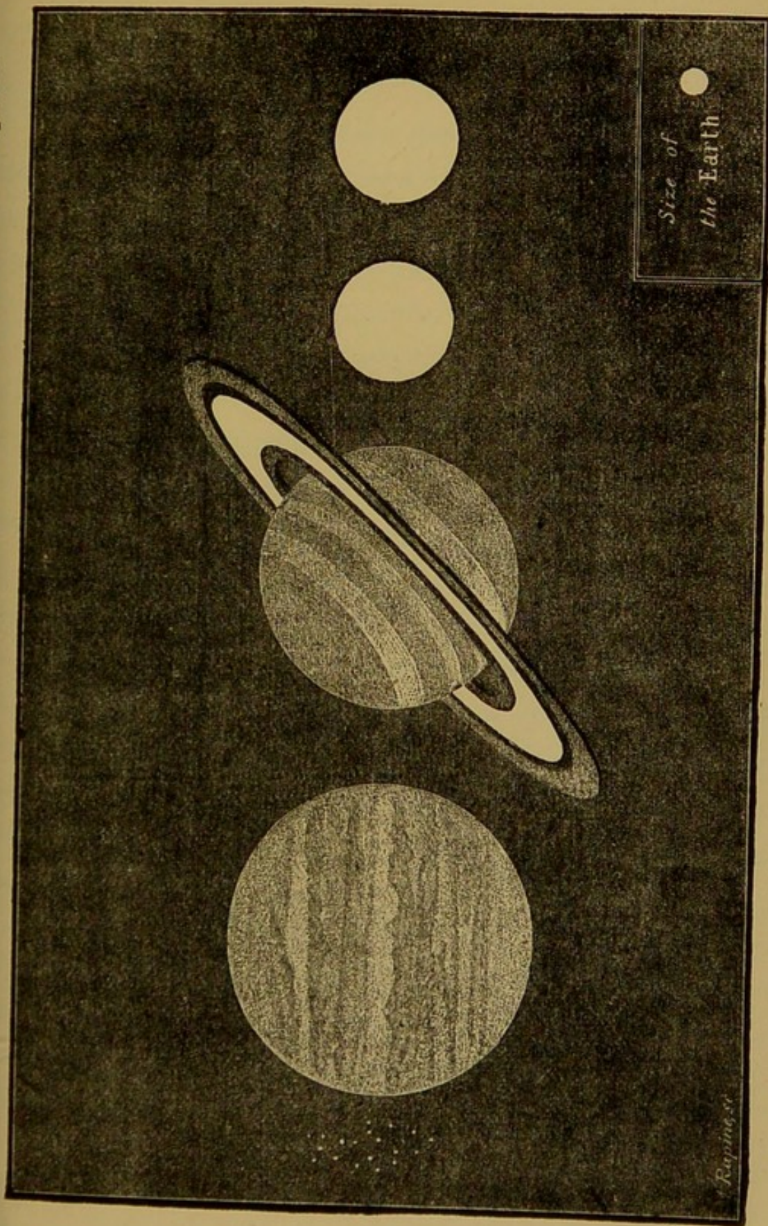
Fig. 5.—Size of the Planets Jupiter, Saturn, Uranus, and Neptune, compared with the Earth,
