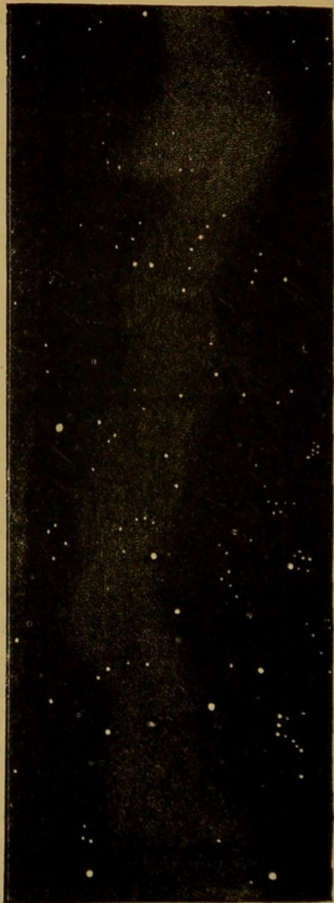
Fig. 10.—The Milky Way.
