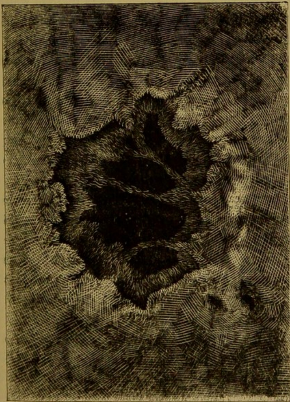
Fig. 3.—Another Solar Spot observed by Nasmyth.
