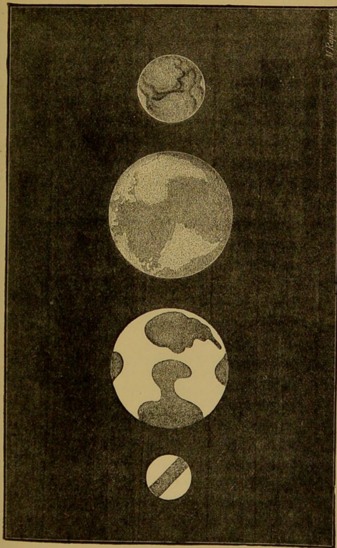
Fig. 4.—Comparative Size of the Planets Mercury, Venus, the Earth, and Mars.
