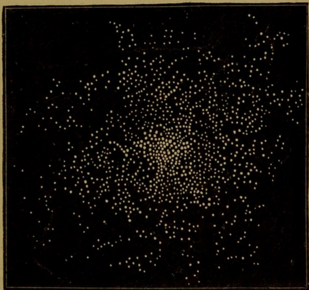
Fig. 8.—The Nebula of the Centaur.
