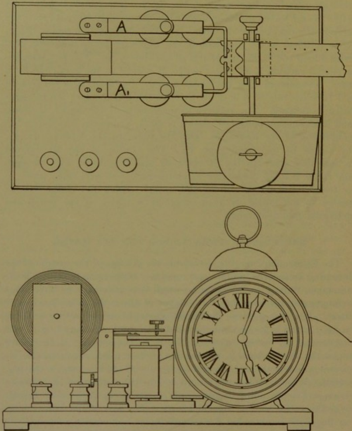
FIG. 11.—Recording apparatus for air meter.
