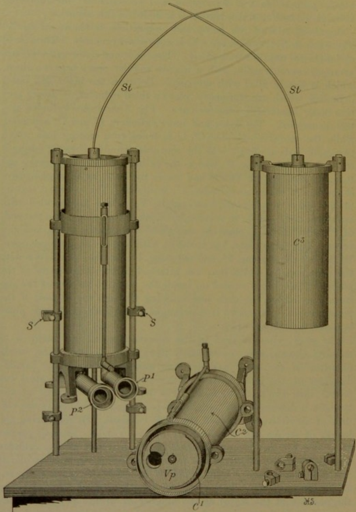
FIG. 8.— Pump cylinder system dismantled.
