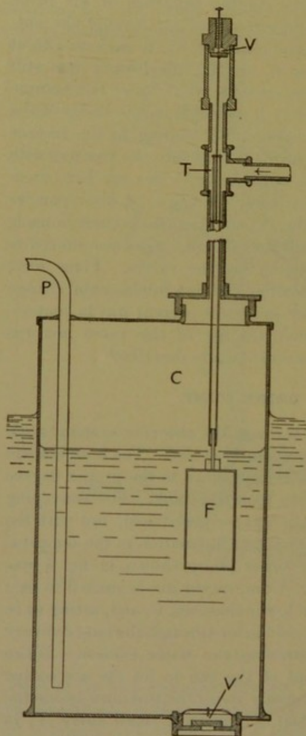
FIG. 4.—Automatic brine pump.
