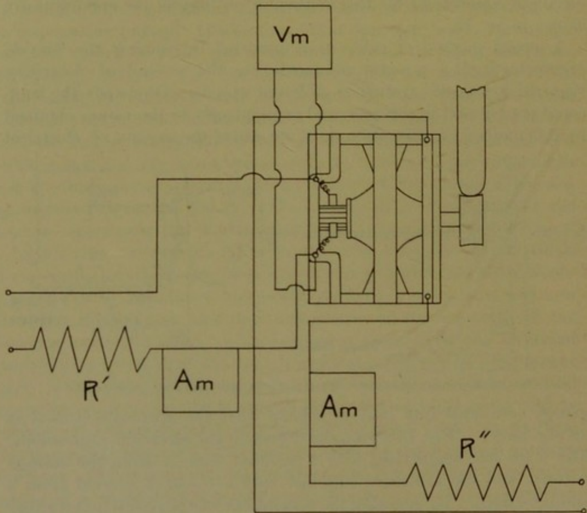
FIG. 14.—Electrical connections for second method of calibrating bicycle ergometer.
