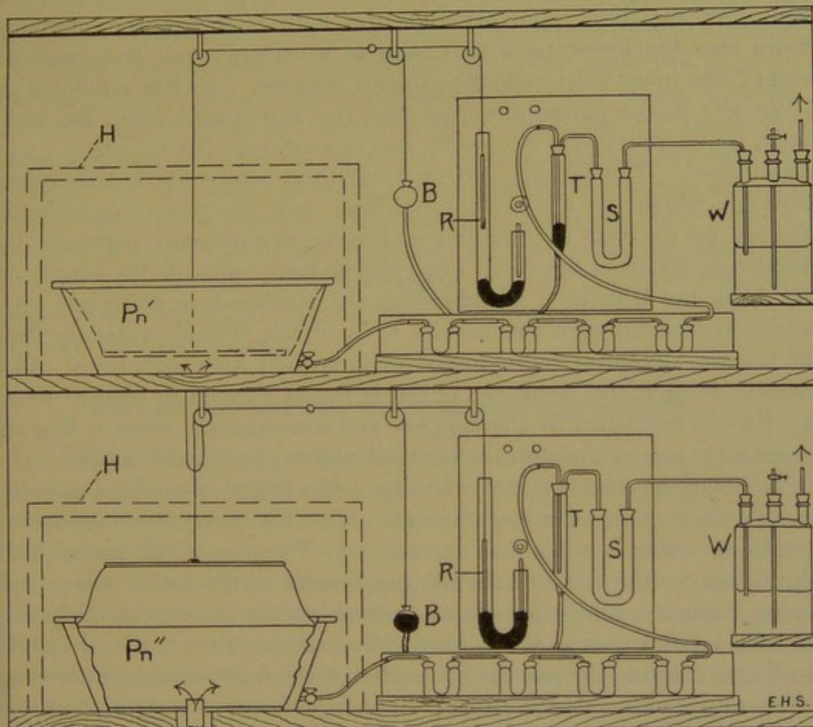
FIG. 10.—Device for collecting and analyzing air sample.
