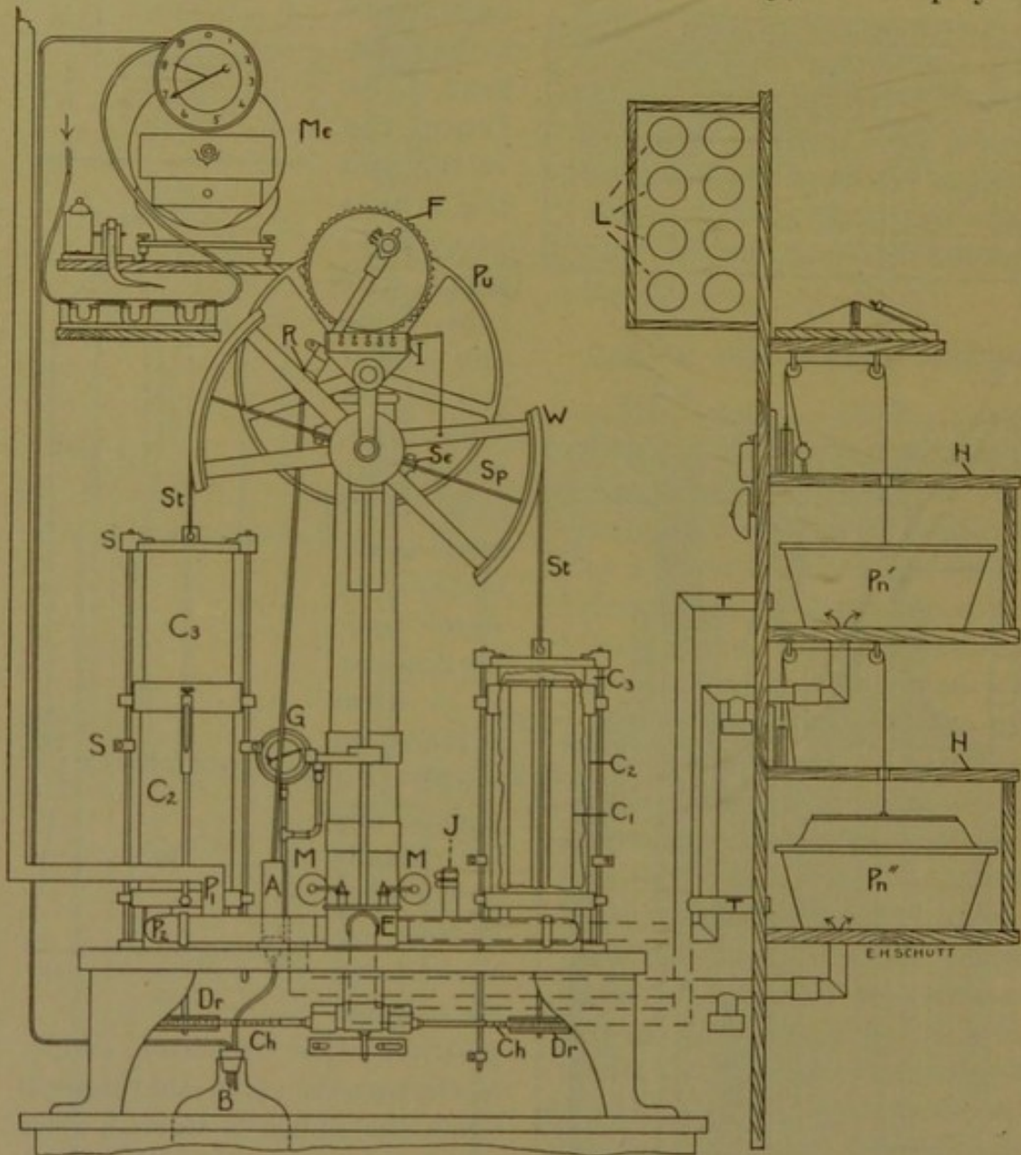
FIG. 7.—Blakeslee meter pump.
