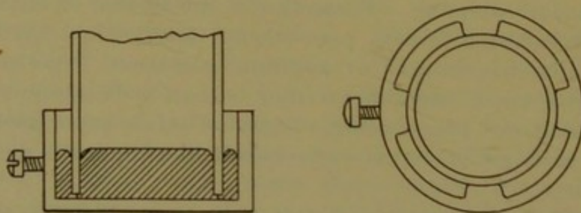
FIG. 9.—Safety trap for air pipes.
