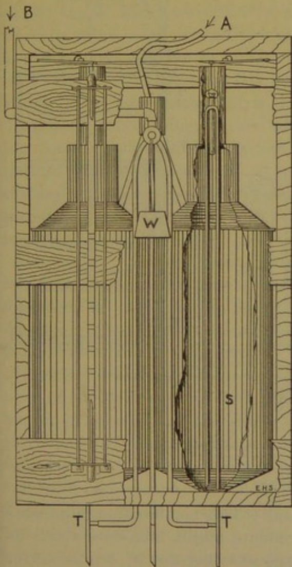
Fig. 6.—Water meter.
