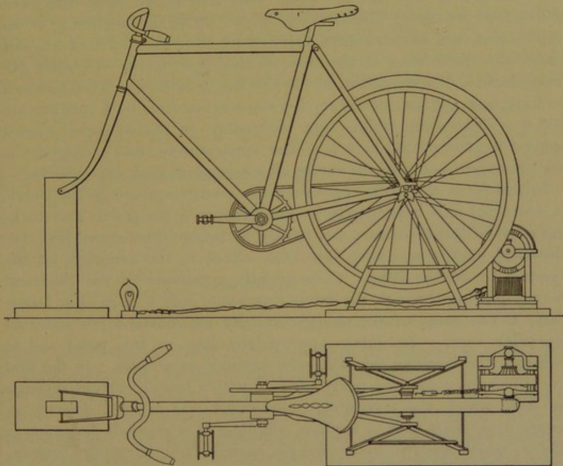
FIG. 12.—Bicycle dynamo or ergometer.
