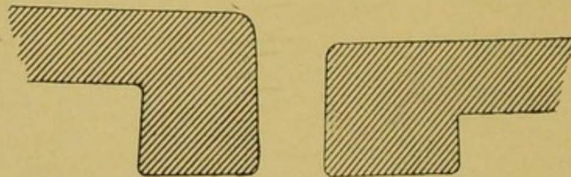
Fig. 40.—Two calkins—the low square one preferable.
