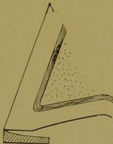
Fig. 52.—Section of a "saucer" shoe.
