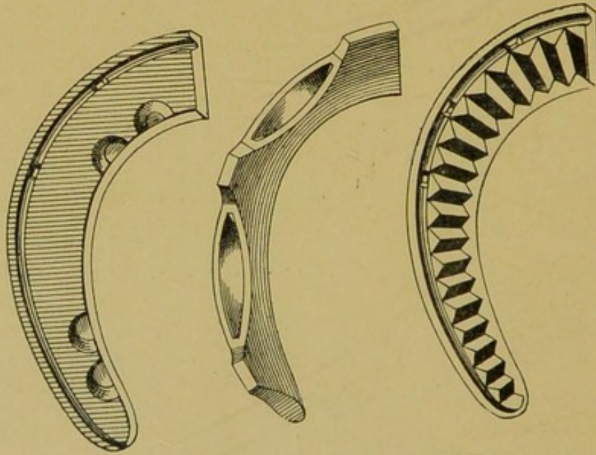
Fig. 38.—Ground-surfaces, notches, projections, ridges.
