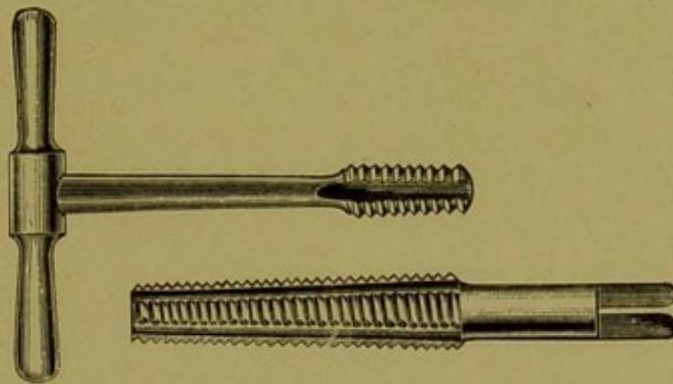
Fig. 72.—Steel Taps for screwing shoes.
