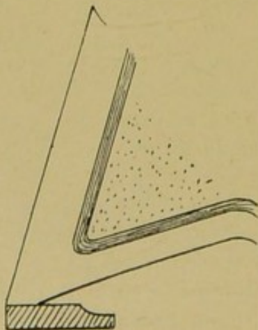
Fig. 55.—Bearing-surface of foot too narrow.
