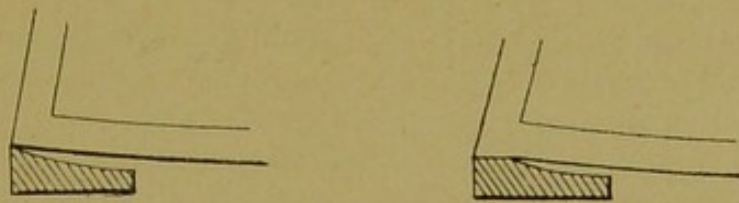
Improper bearing surface. Fig. 80. A level bearing surface.
