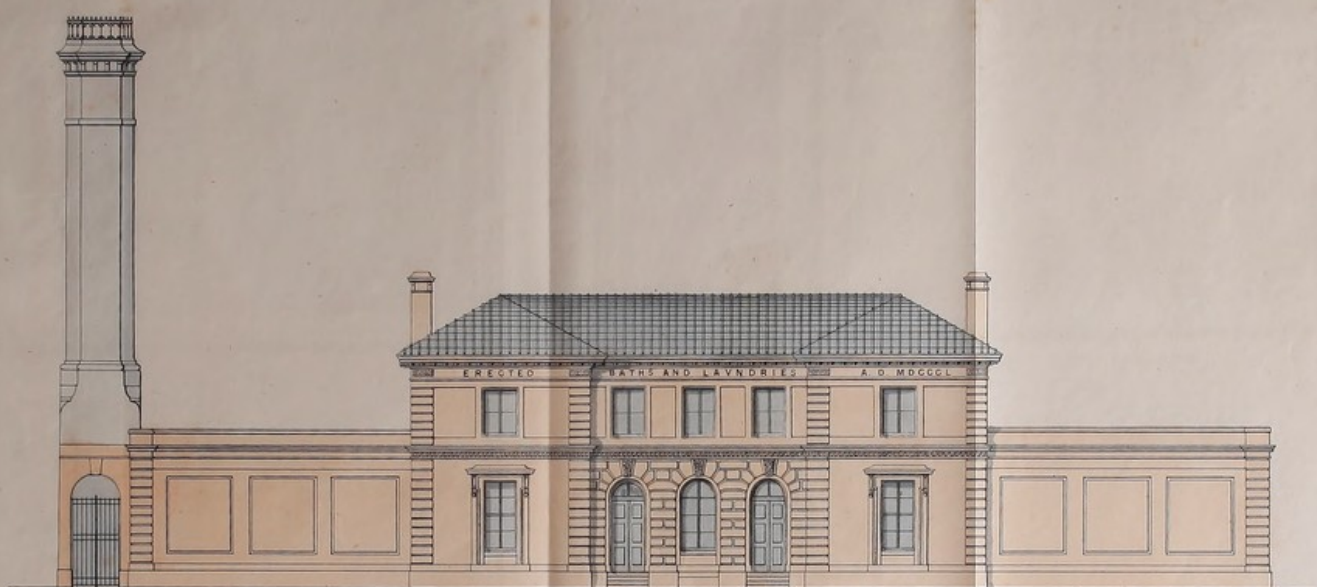
ELEVATION OF AN ESTABLISHMENT ADAPTED TO PLAN N° 1.
