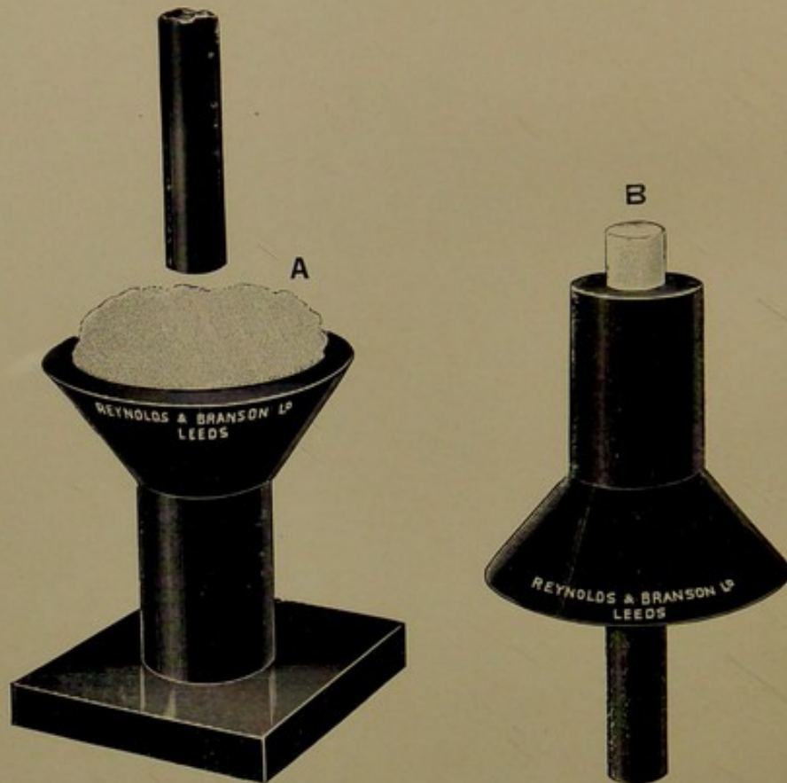
FUNNEL-SHAPED MOULD.
