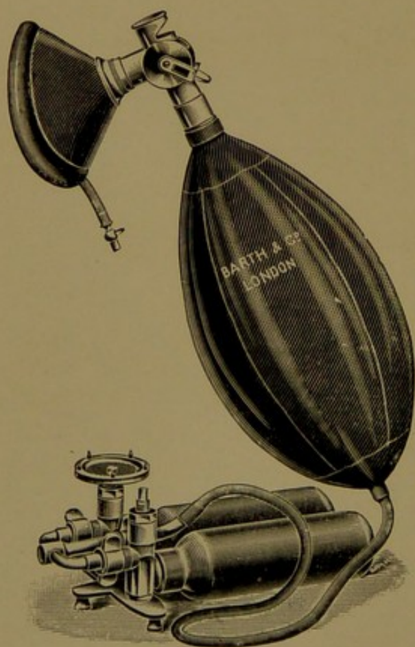
FIG. 4.—BARTH'S NITROUS OXIDE APPARATUS.
