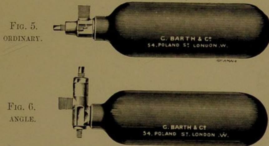
NITROUS OXIDE CYLINDERS.
