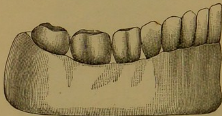
FIG. 30.—From a model of a lower maxilla, aged 40 years. The maxilla curves upward in front, thus raising its front teeth considerably above its lower bicuspid and molars. The result of this is that the upper front teeth are deeply indented and worn away, as regards the posterior surface of their fangs. They are, moreover, much loosened and so pushed forward as to lie in an almost horizontal position. A gold plate capping the lower molars is now worn and thus, the bite being raised, the upper front teeth are preserved.
