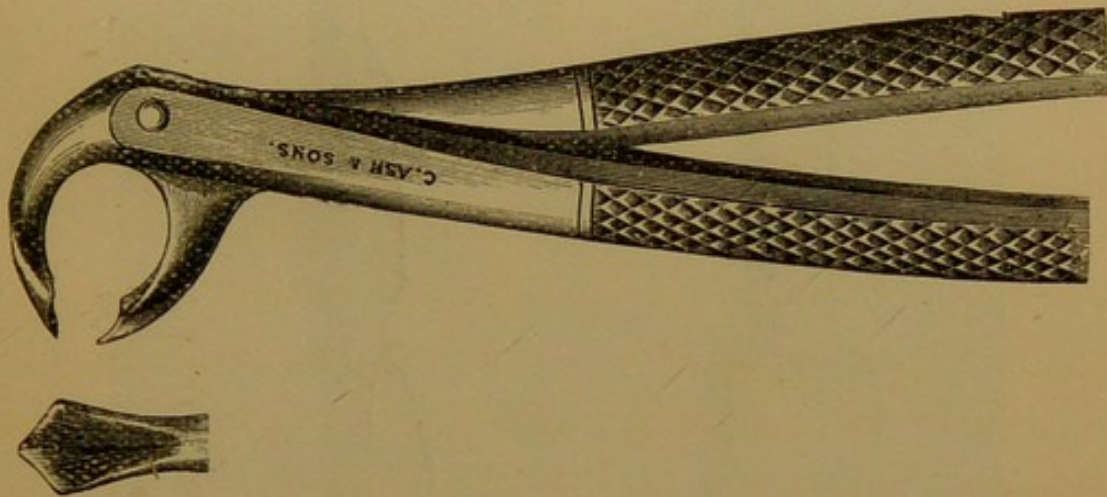
FIG. 83.—Lower molar forceps for either side of the mouth. The width of the blades is also shown.
