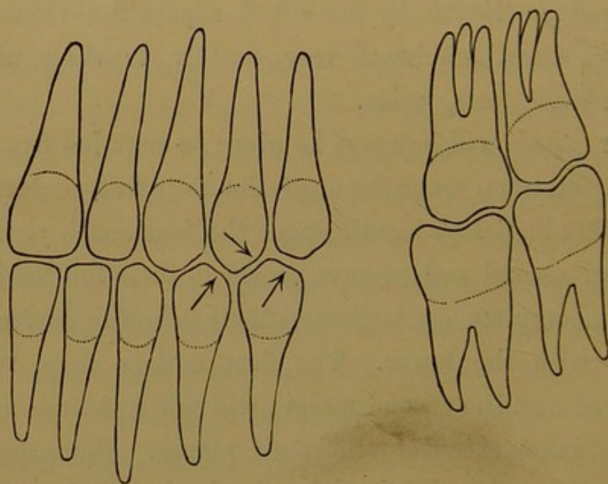
FIG. 17.—The arrows show the direction in which the four bicuspid will frequently move after symmetrical extraction of four 1st molars. (From Smale and Colyer's Diseases and Injuries of the Teeth . Longmans & Co.)
