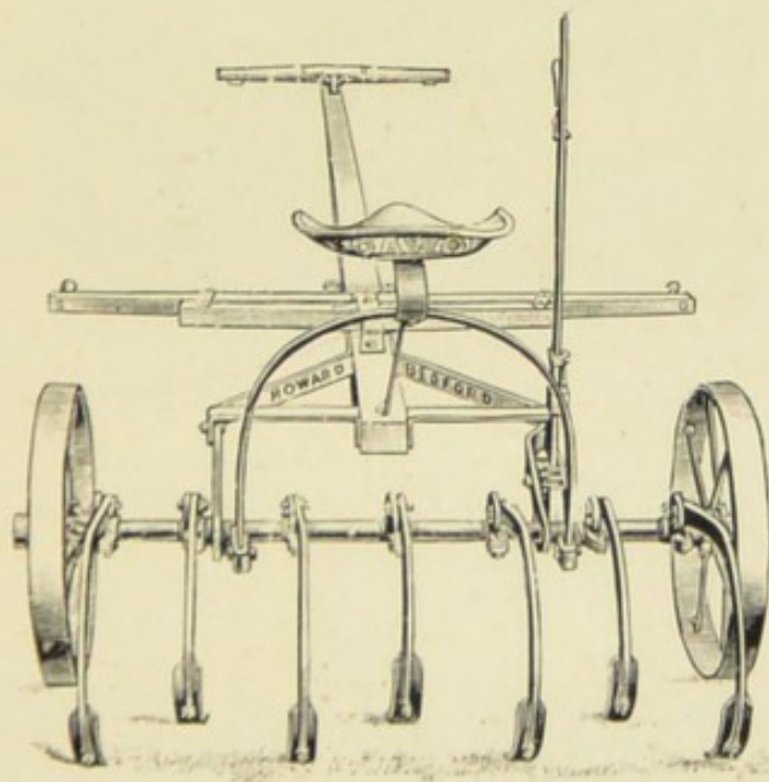
FIG. 66.—HOWARD'S CULTIVATOR, NO. 7.
