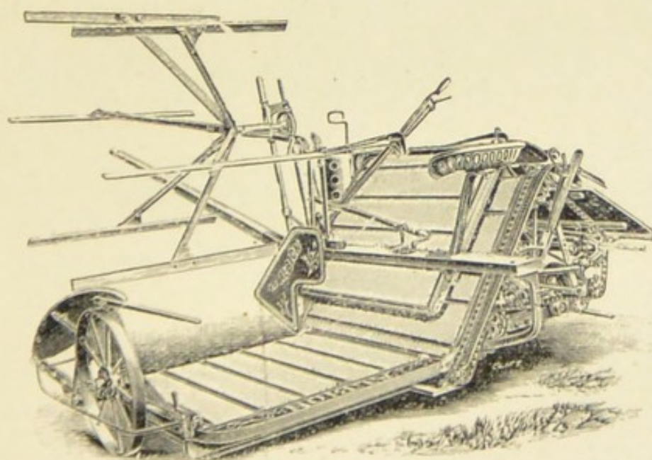
FIG. 73.—HARRISON, MACGREGOR & Co.'s SHEAF-BINDING MACHINE, "THE ALBION."
