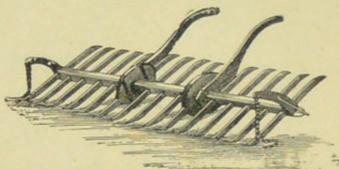
FIG. 68.—HAY GATHERER.
