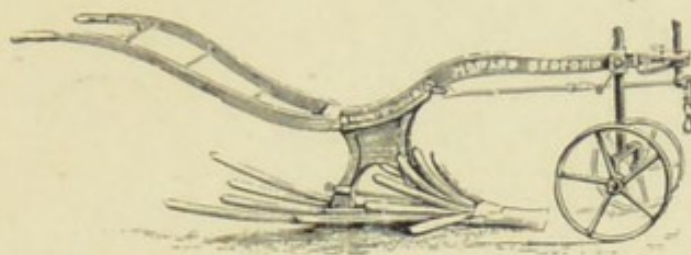
FIG. 64.—HOWARD'S POTATO-DIGGING PLOUGH.
