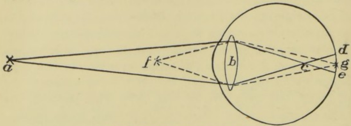
Diagram of the eye in near sight.
