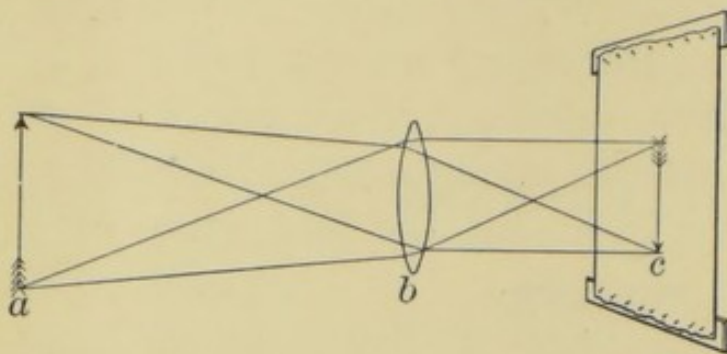
Diagram of the formation of an image with a lens.
