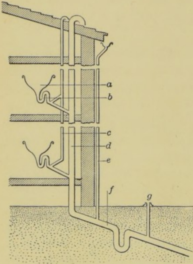
Diagram of the plumbing of a house.
