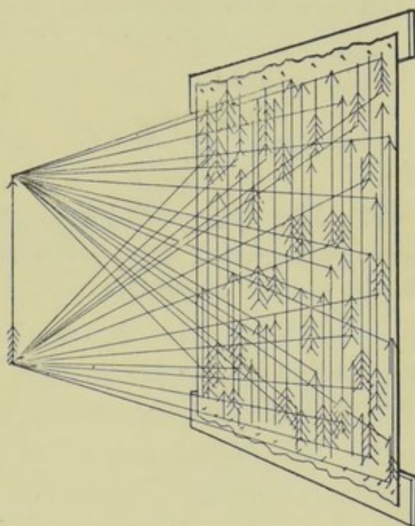
Diagram of light passing from an object.
