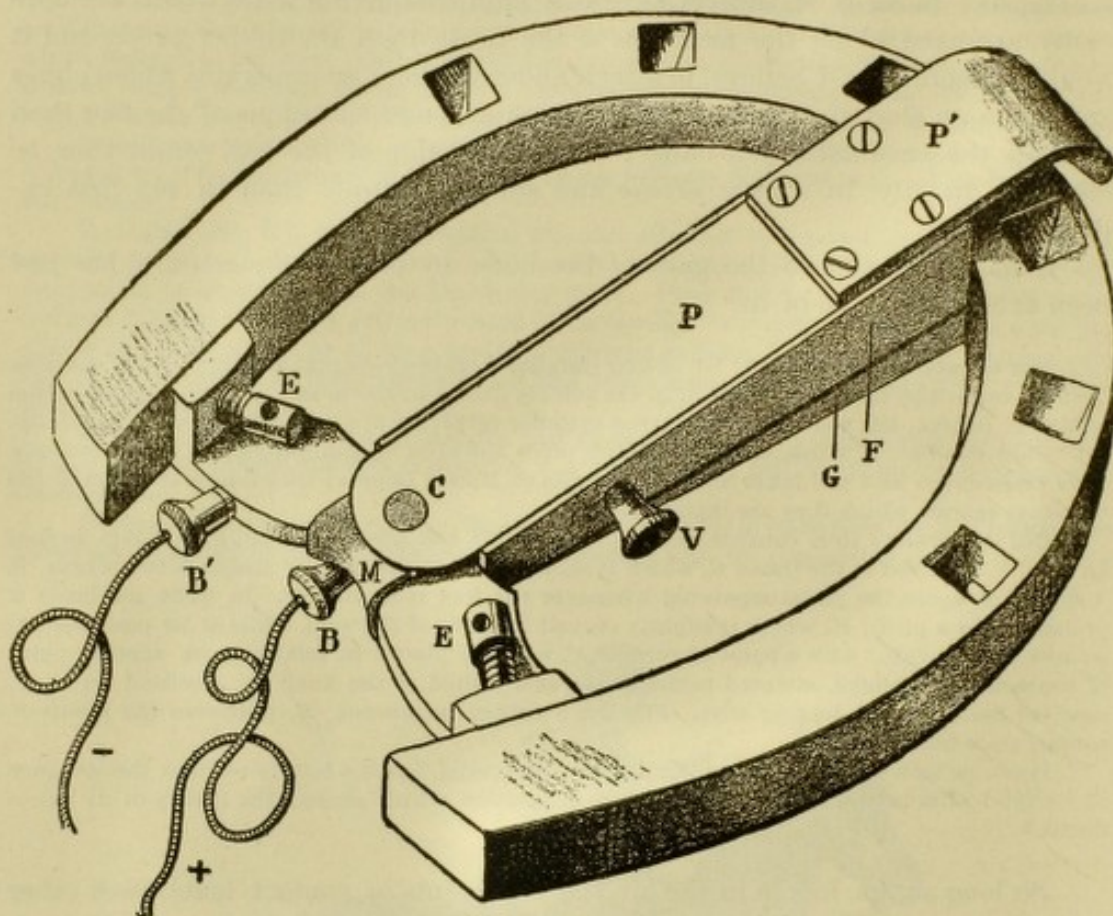
FIG. 178.— Chaussure exploratrice for registering the gaits by electricity.
