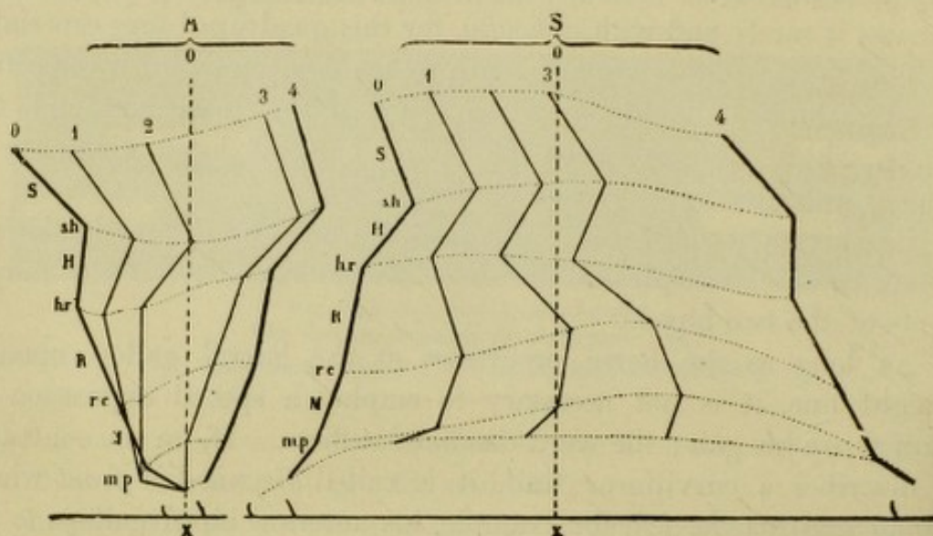
FIG. 238.—Kinematic analysis of the play of the anterior member in the gallop . (From Messrs. Marey and Pagès.)
