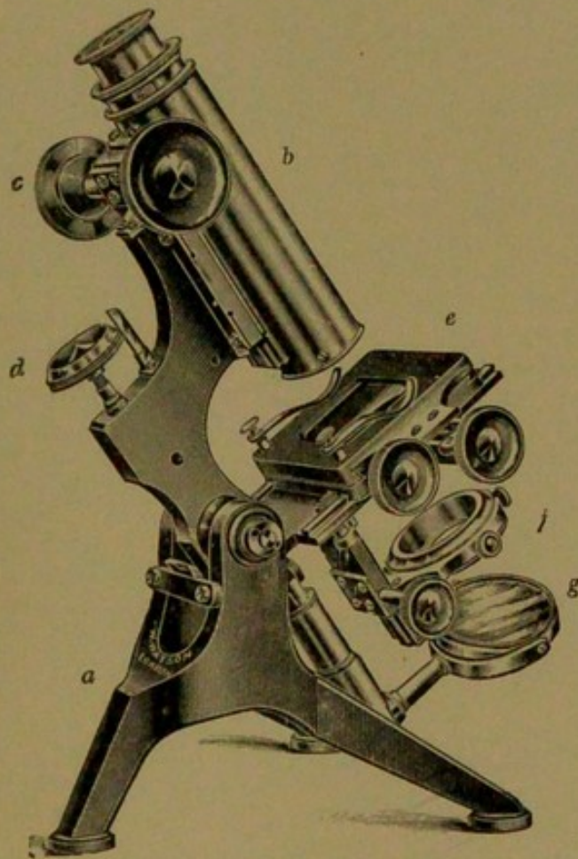
FIG. 40.—Microscope stand.
