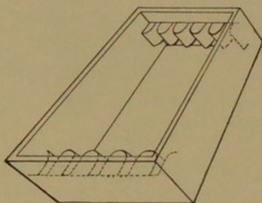
FIG. 76.—Staining pot.
