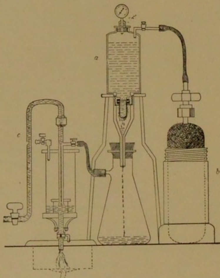
FIG. 38.—Pakes' filtering reservoir—pressure and aspiration.
