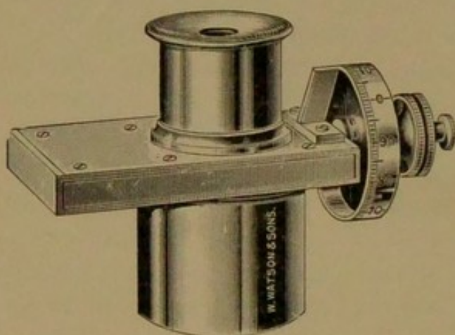
FIG. 58.—Ramsden's Filar micrometer.
