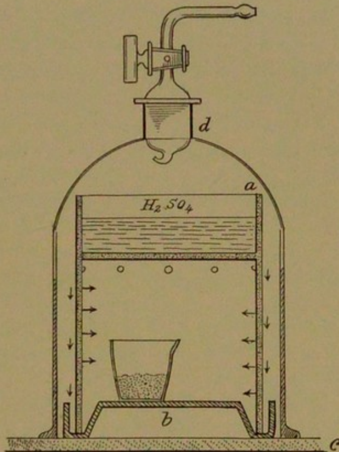
FIG. 157.—Mueller's desiccator.
