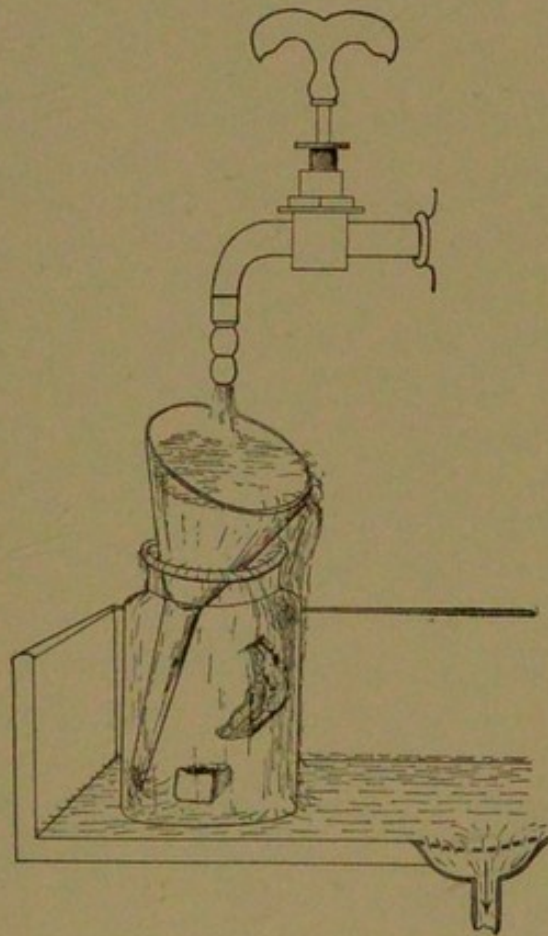
FIG. 71.—Washing tissues.
