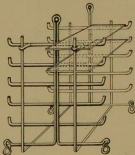
FIG. 75.—Section rack.
