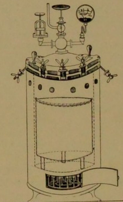
FIG. 30.—Chamberland's Autoclave.
