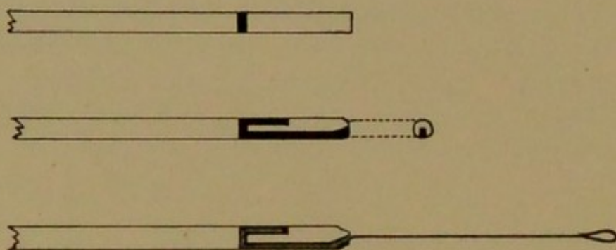
FIG. 64.—Platinum rod in aluminium handle—method of mounting.
