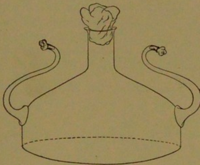
FIG. 33.—Ruffer's flask.
