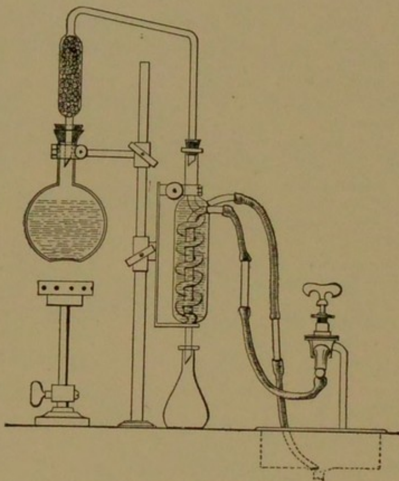
FIG. 152.—Arrangement of distillation apparatus for acids, etc.
