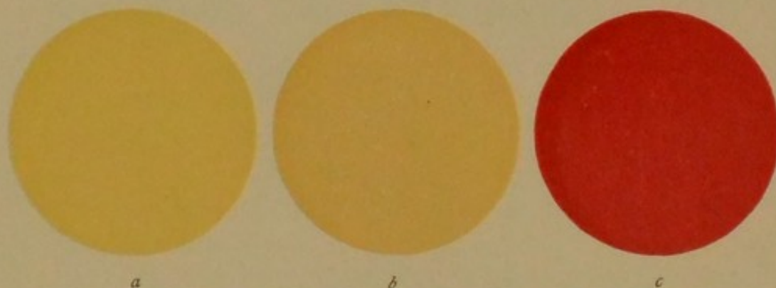
FIG. 98.—a, Sample of filtered meat extract or nutrient gelatine to which phenolphthalein has been added. The medium is acid, as evidenced by the unaltered colour of the sample. b, The same neutralised by the addition of \frac{n}{10} NaOH. The production of this faint rose-pink colour indicates that the "end-point," or neutral point to phenolphthalein, has been reached. If such a sample is cooled down to say 30° or 20° C., the colour will be found to become more distinct and decidedly deeper and brighter, resembling that shown in c. c, Also if, after the end-point is reached, a further 0.5 c.c. or 1.0 c.c. \frac{n}{10} NaOH be added to the sample, the marked alkalinity is evidenced by the deep colour here shown.
