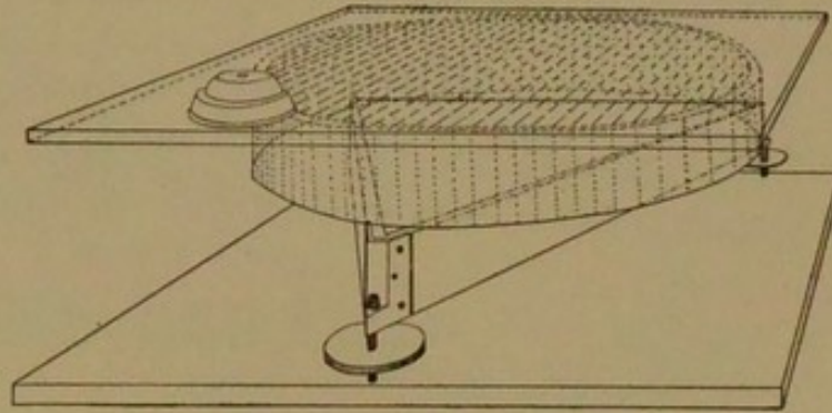
FIG. 122.—Plate-leveiling stand.
