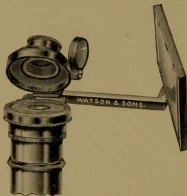
FIG. 55.—Camera lucida, Abbé pattern.
