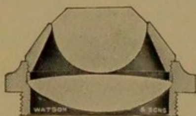
FIG. 47.—Optical part of Abbé illuminator.
