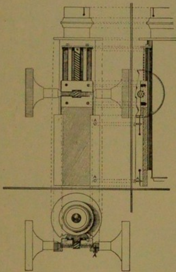
FIG. 42.—Coarse adjustment.
