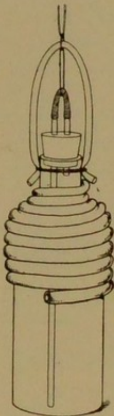
FIG. 204.— Thresh's deep water sampling bottle.
