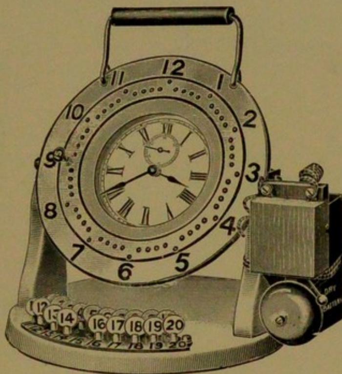
FIG. 31.—Electric signal timing clock.
