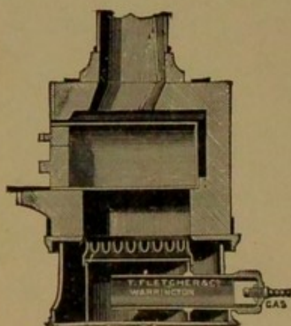
FIG. 25.—Muffle furnace.
