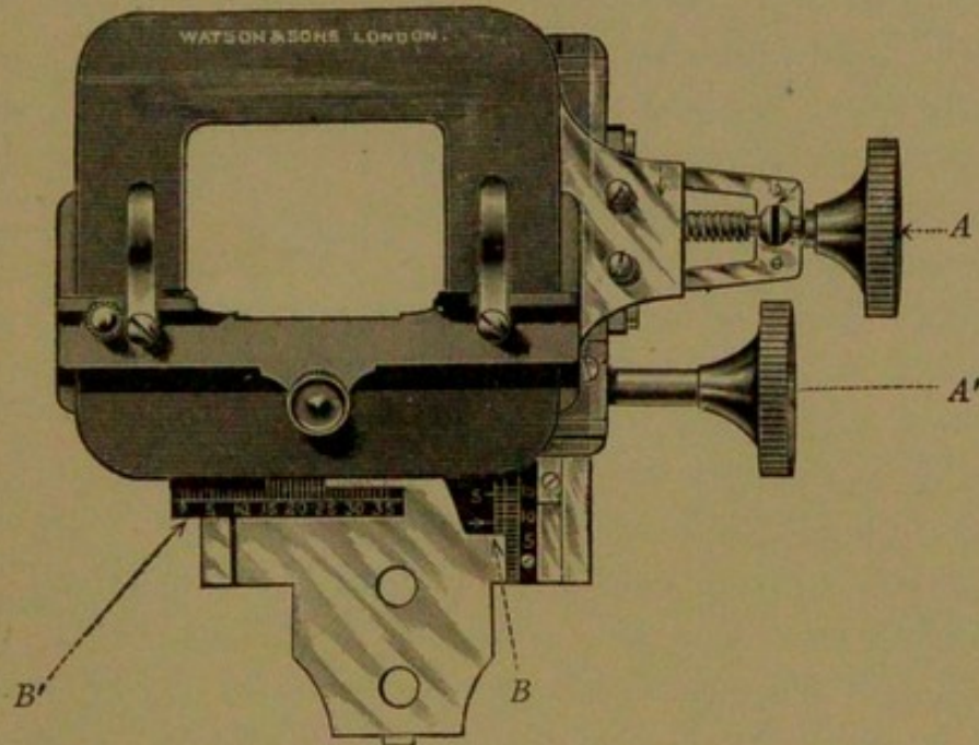
FIG. 45.—Mechanical stage.
