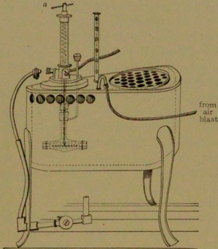
FIG. 155.—Hearson's water-bath.
