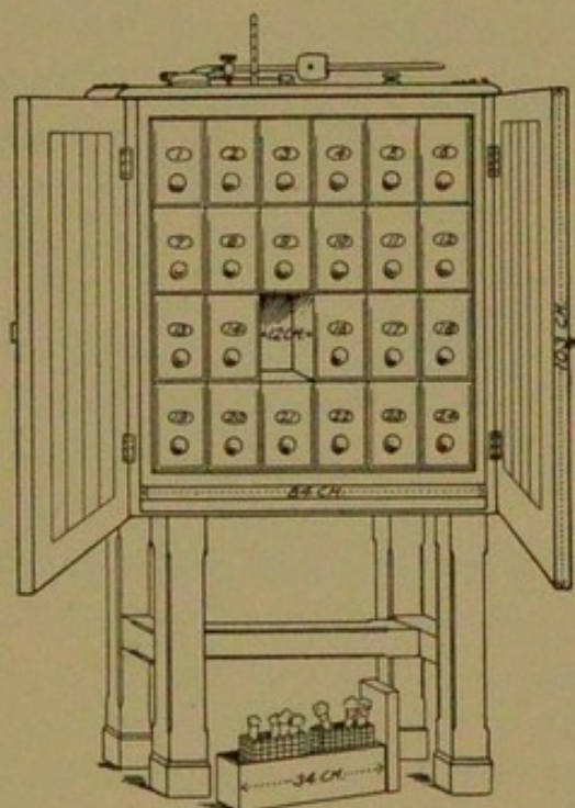
FIG. 114.—Cellular incubator.
