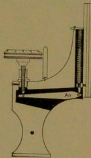
FIG. 43.—Fine adjustment.
