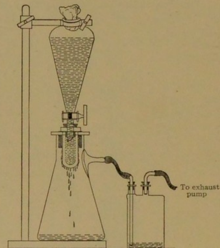
FIG. 37.—Apparatus arranged for filtering—aspiration.
