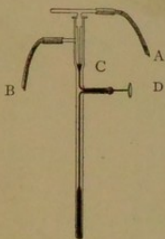
FIG. 115.—Reichert's thermo-regulator.
