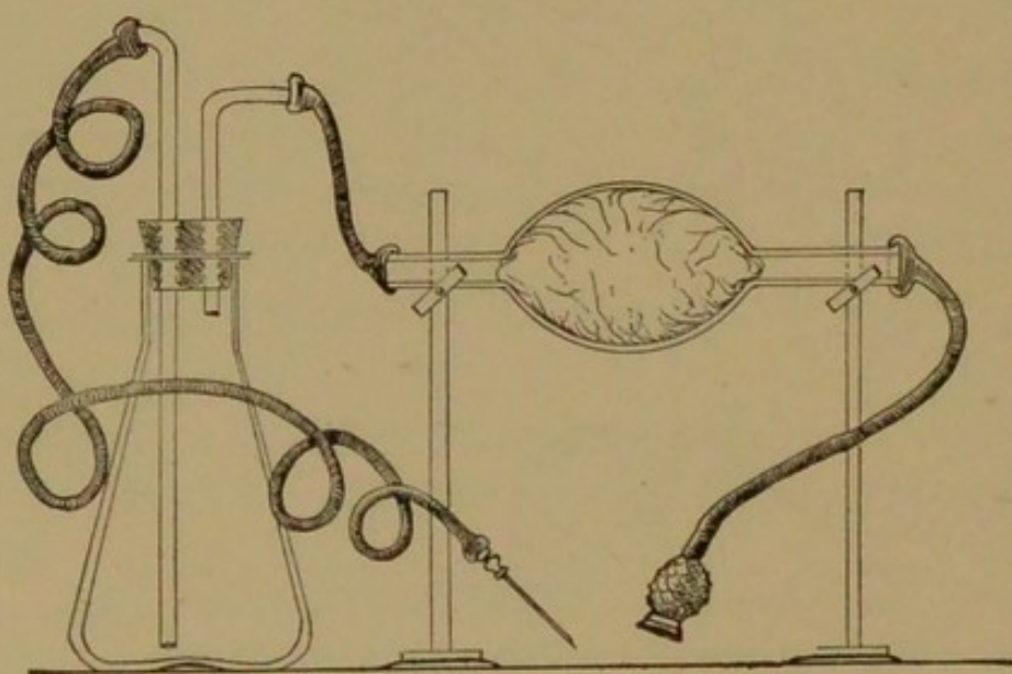
FIG. 174.—Arrangement of pressure injection apparatus.
