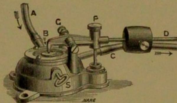
FIG. 116.—Capsule thermo-regulator.
