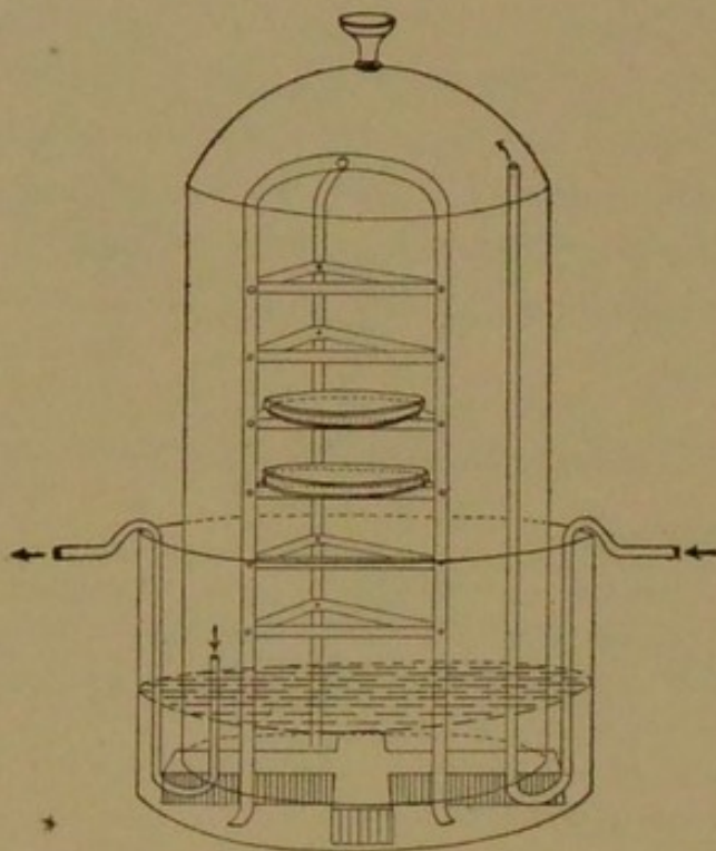
FIG. 134.—Botkin's apparatus.
