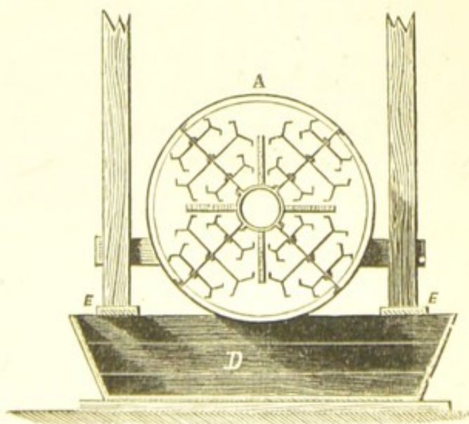
PLATE VII.—GUARDIOLA'S COFFEE DRYER.
