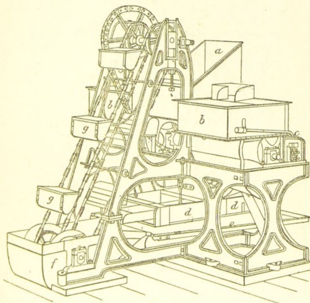
Gearless Pulper.
