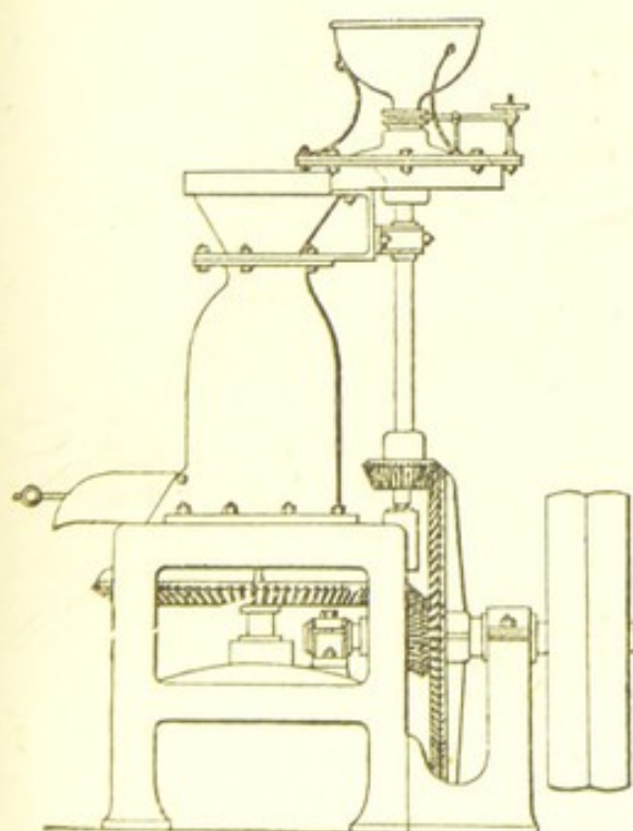
Peeling and Polishing Machine.
