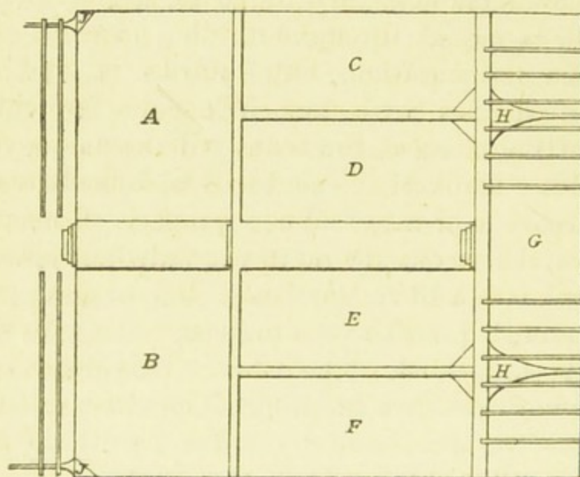
Fermenting Tanks.
