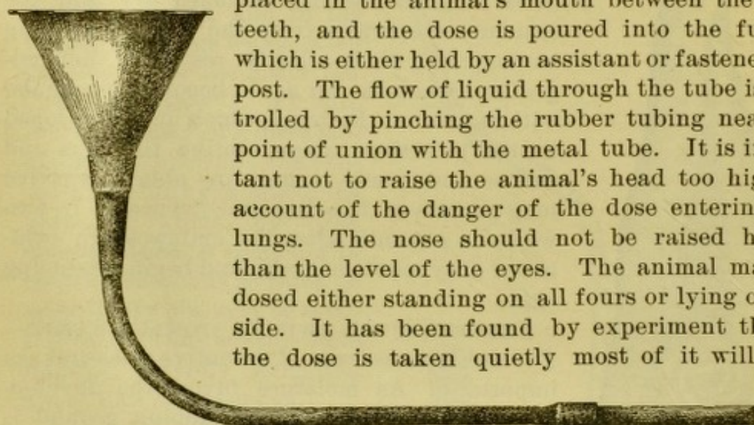
FIG. 18.—A drenching tube made from an ordinary tin funnel, a piece of rubber hose, and a piece of brass pipe.
