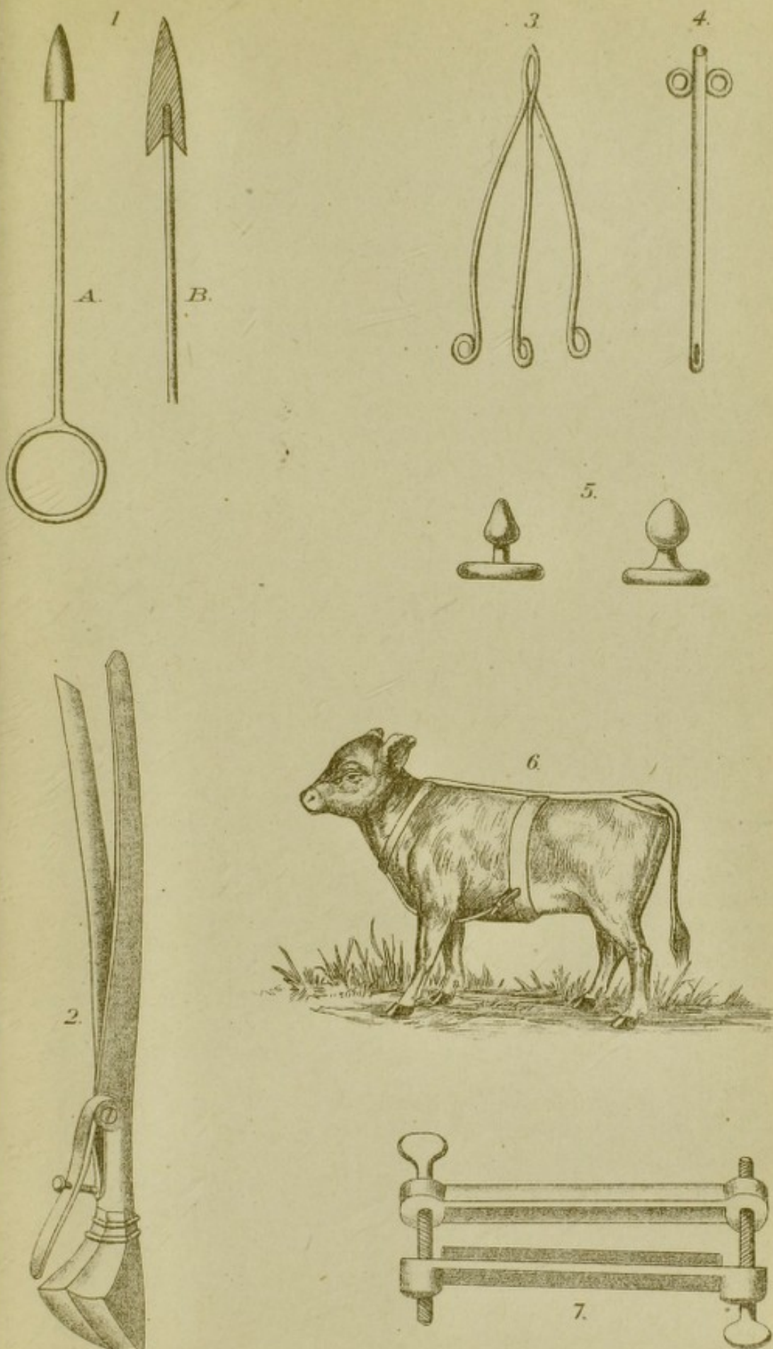
INSTRUMENTS USED IN DISEASES FOLLOWING PARTURITION.
