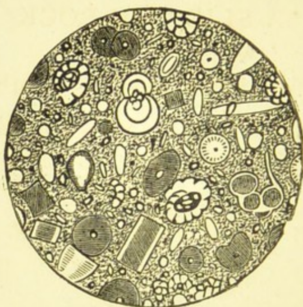
Section of Limestone.
