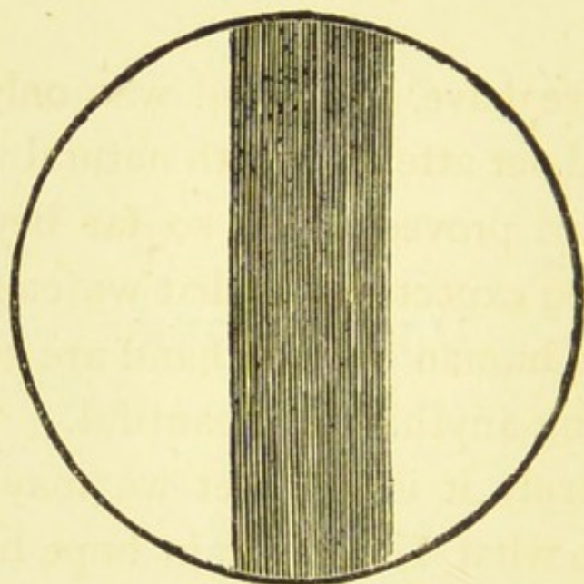
The Fifteenth Band of Nobert's Test Plate.
