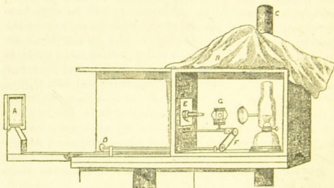
A—Frame for receiving sensitive plate and focusing screen, B—Black velvet curtain for shutting in the light. C—Chimney. D—Handle of focusing rod. E—Sliding plate for changing objectives. F—Endless band acting on fine adjustment of G—The object carrier.
