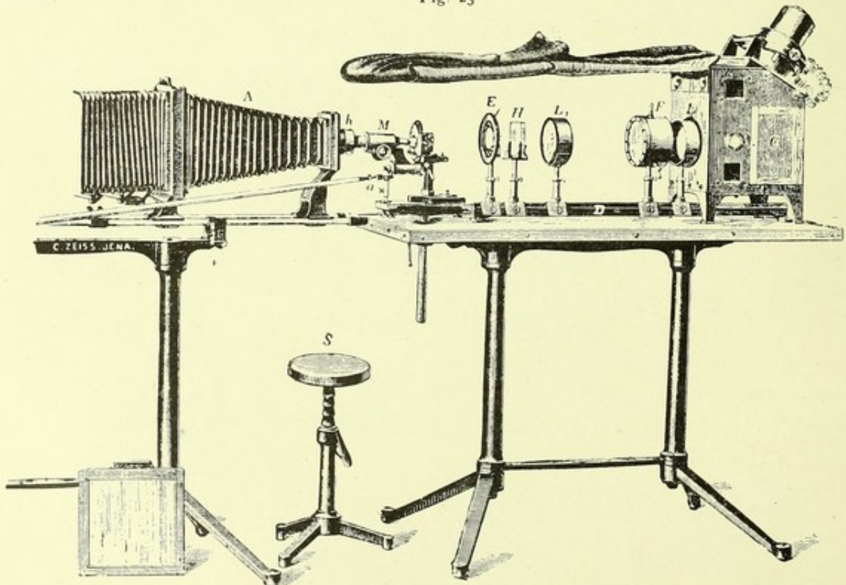
Large Photo-Micrographic and Projection Apparatus
