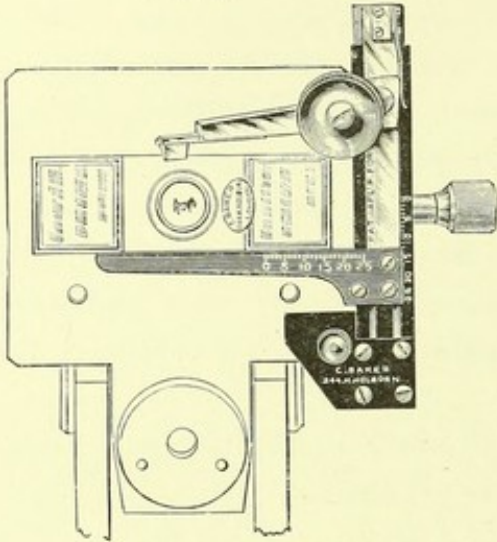
Baker's Removable Stage
