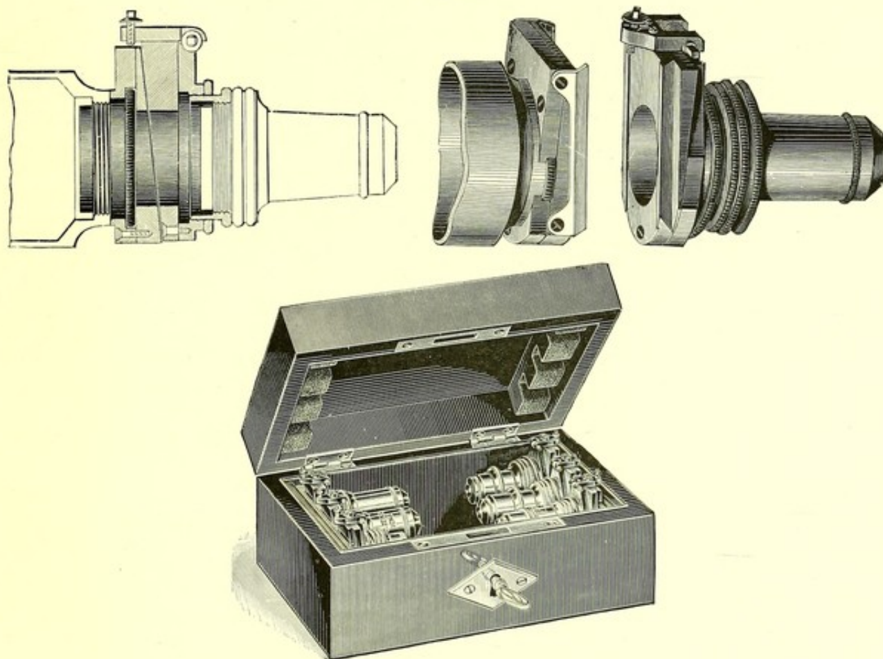
Zeiss Sliding Objective Changer
