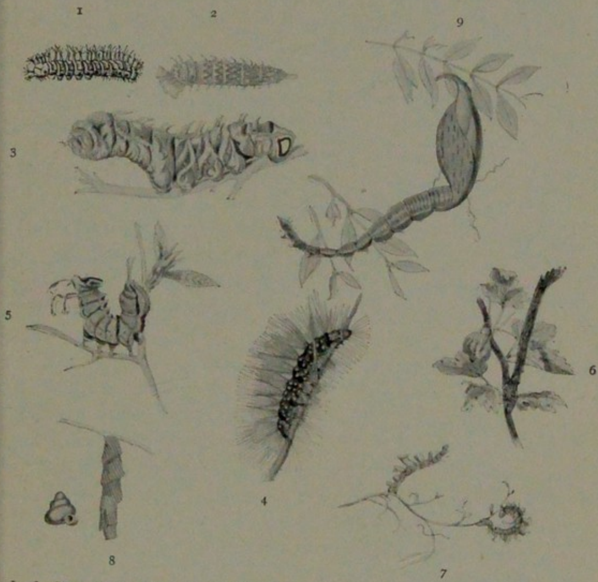
1.-3. STAGES IN THE LIFE-HISTORY OF THE ATLAS MOTH CATERPILLAR, SHOWING CHANGES IN THE FORM OF THE SPINY ARMATURE (after Poujade). 4. CATERPILLAR OF TIGER MOTH, SHOWING ARMATURE OF BRISTLES. 5. CATERPILLAR OF LOBSTER MOTH IN A THREATENING ATTITUDE. 6. CATERPILLAR OF FEATHERED THORN MOTH ( Himeria ), SHOWING STICK-LIKE ATTITUDE. 7. CATERPILLAR OF ESSEX EMERALD MOTH WITH LEAVES ATTACHED TO BODY FOR DISGUISE. 8. DWELLING-CASES OF CASE-WEAVER MOTHS ( Psychidæ ). 9. CATERPILLAR OF HAMMOCK-MOTH IN CASE MADE OF ITS OWN EXCREMENT.
