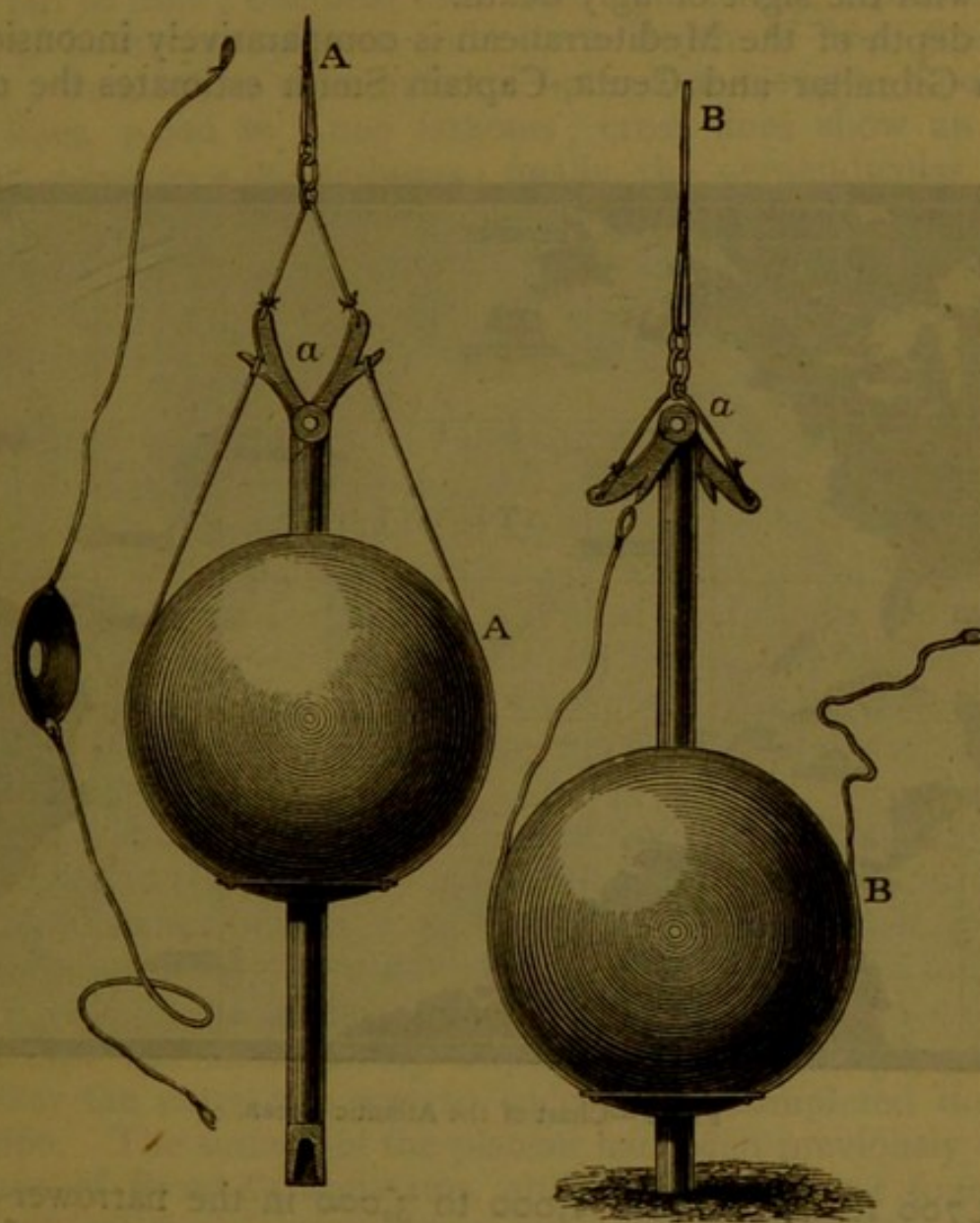
Fig. 1. — Brooke's Sounding Apparatus
