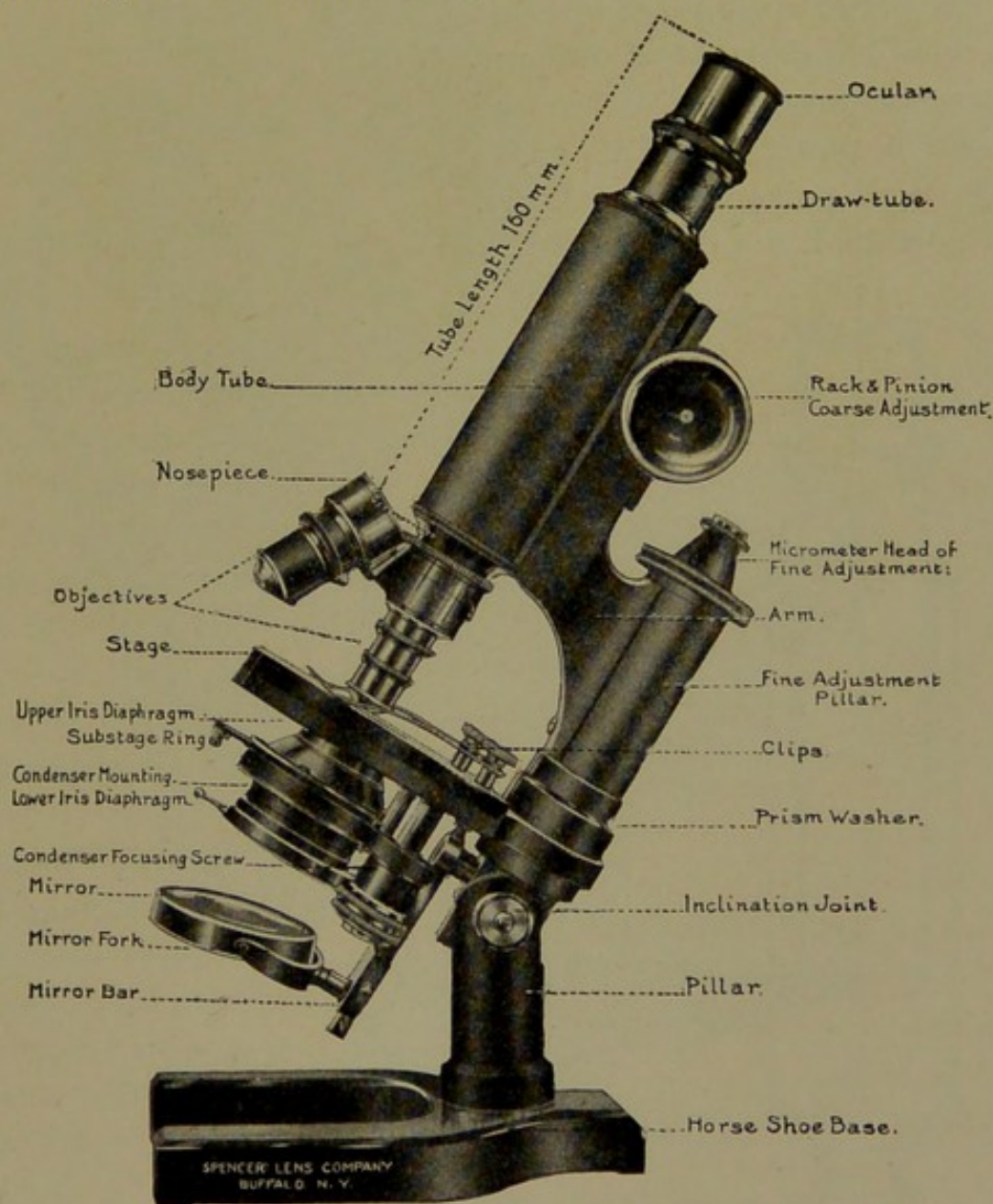
FIG. 51.—A Compound Microscope with Parts Named.
