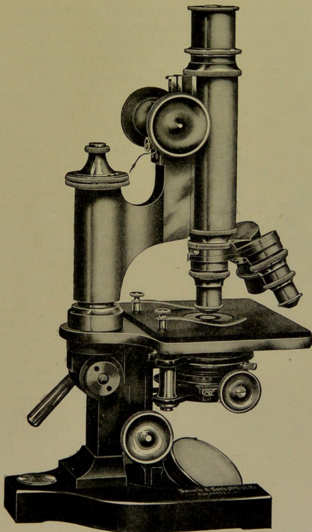
FIG. 57.—The Bausch and Lomb CA Stand.
