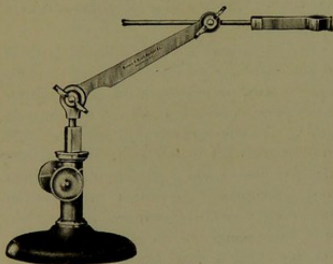
FIG. 65.—Stand for Dissecting Lens.
