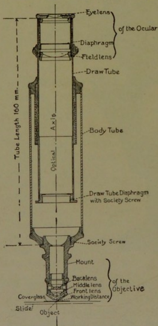
FIG. 52.—Sectional View of Microscope Tube including Ocular and Objective.
