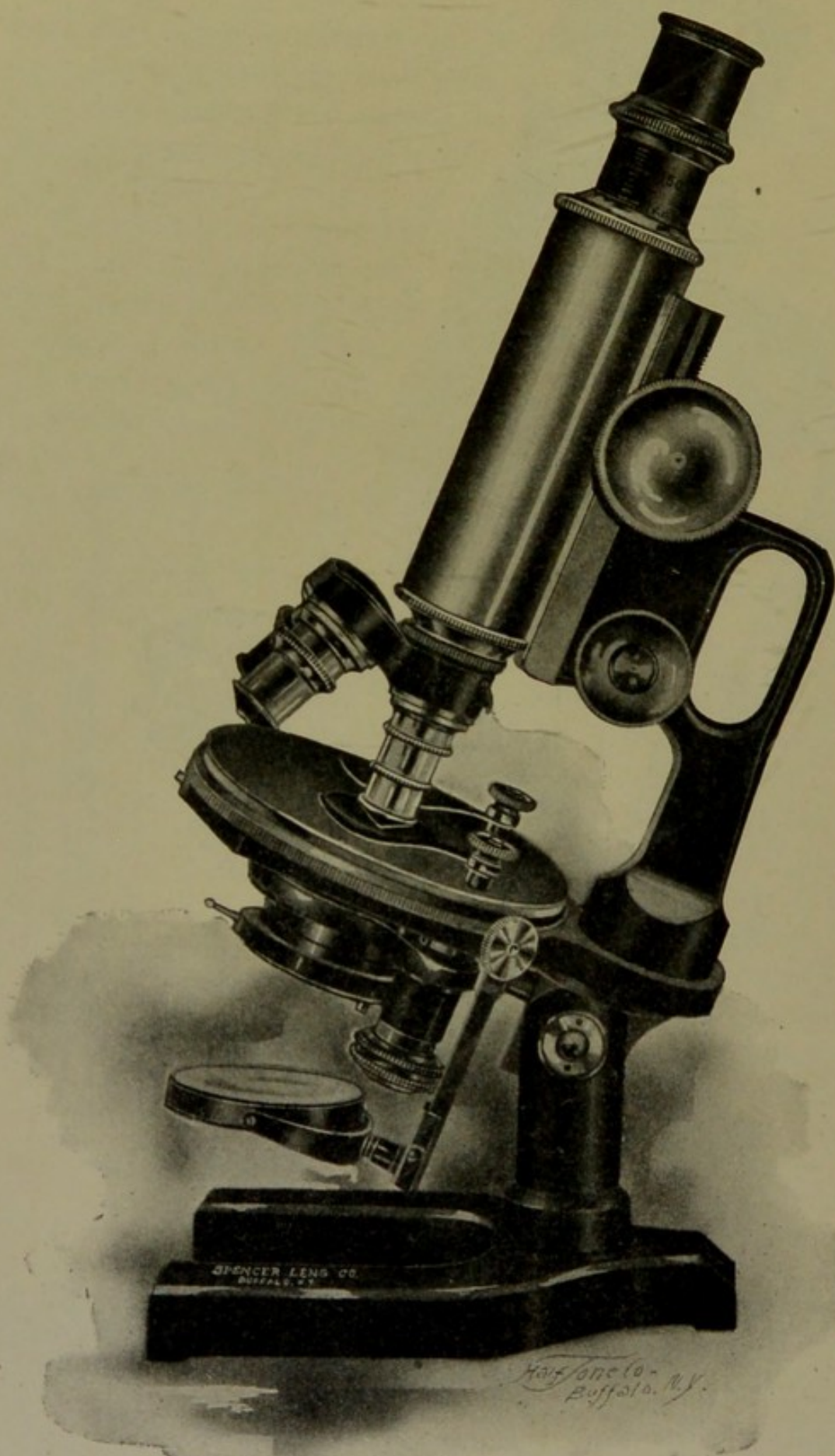
FIG. 56.—The Spencer No. 25 Stand.
