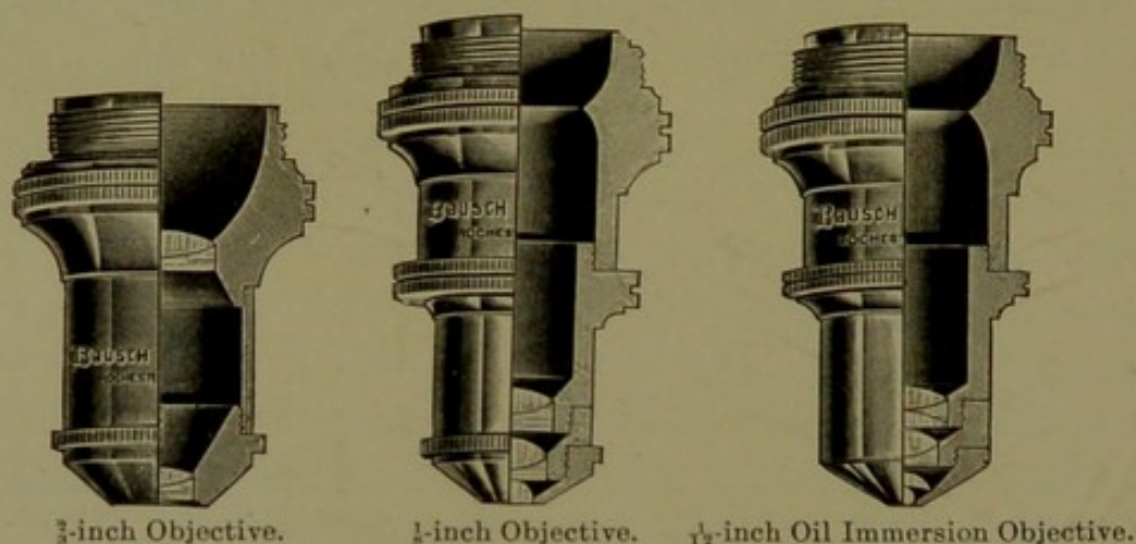
FIG. 49.—Lens Systems of Various Objectives.
