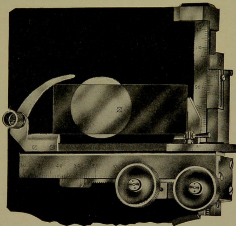
FIG. 68.—Attachable Mechanical Stage.
