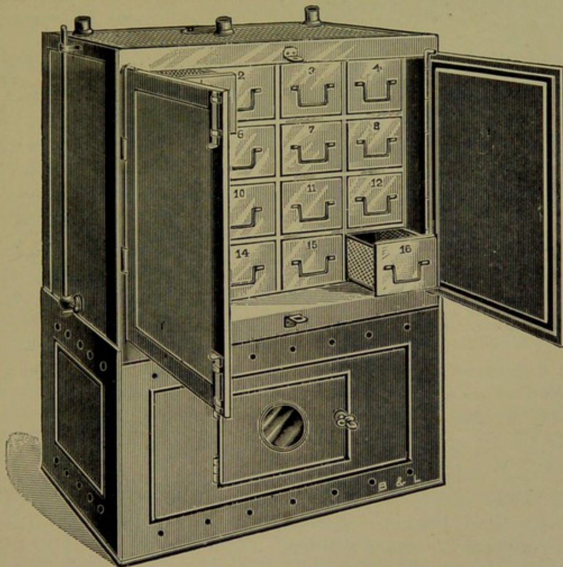
FIG. 24.—The Lillie Water-Bath.
