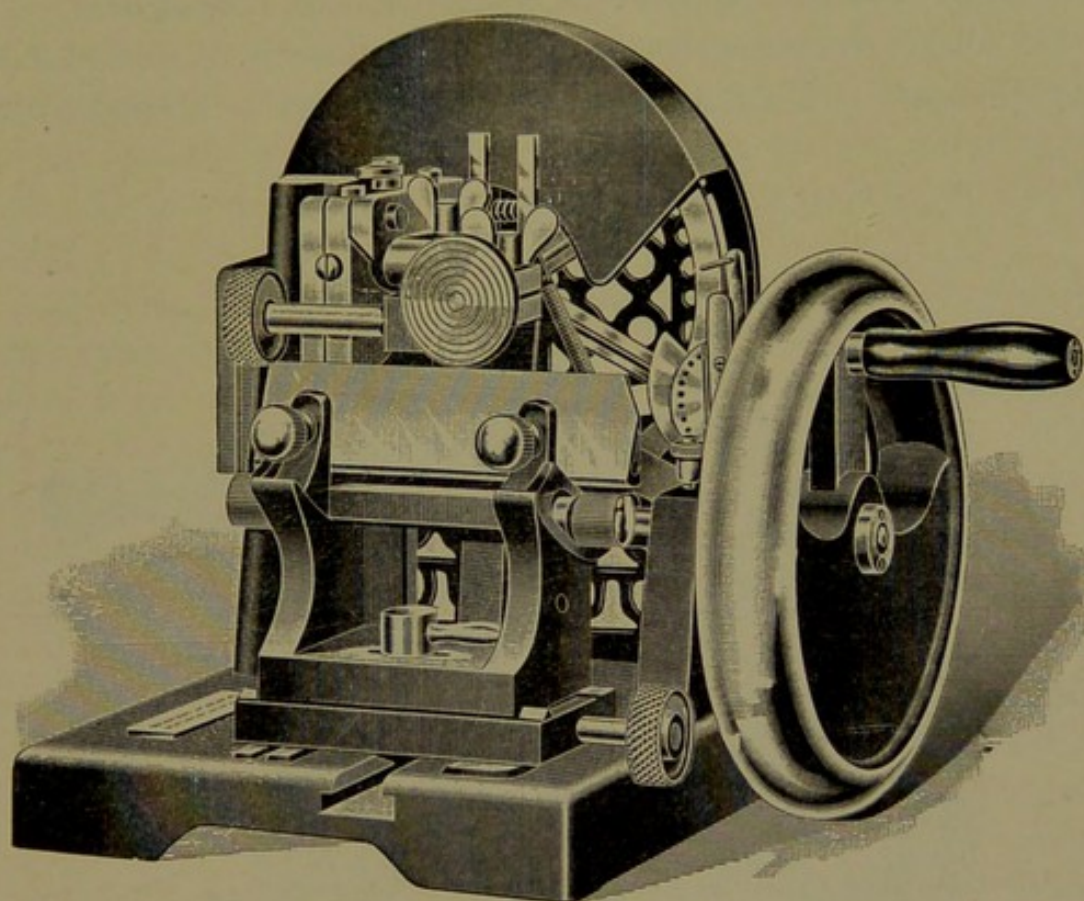
FIG. 28.—Minot Automatic Rotary Microtome.
