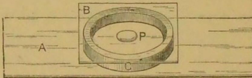
A, glass slide; B, cover-glass; C, glass ring forming the wall of the chamber; P, drop of nutritive liquid in which the micro-organisms grow. ( Klein. )
