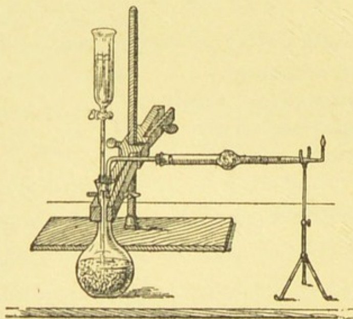
ANALYTICAL APPARATUS.
