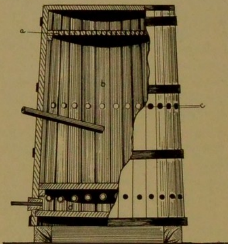
FIG. 165. Cask for the continuous, quick, or German method of making vinegar. The alcoholic solution trickles through the holes at a , and passes over the chips or shavings which fill the space b . Air enters through the openings at c . The vinegar collects in the lower portion ( d ). (Adapted from Dammer.)
