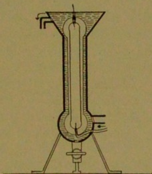
FIG. 119. Cooper-Hewitt mercury vapor lamp adapted for sterilization of water. The water enters at the bottom and leaves at the top, passing along the side of the lamp, and is thus exposed to the rays effectively. (Adapted from Bertarelli.)
