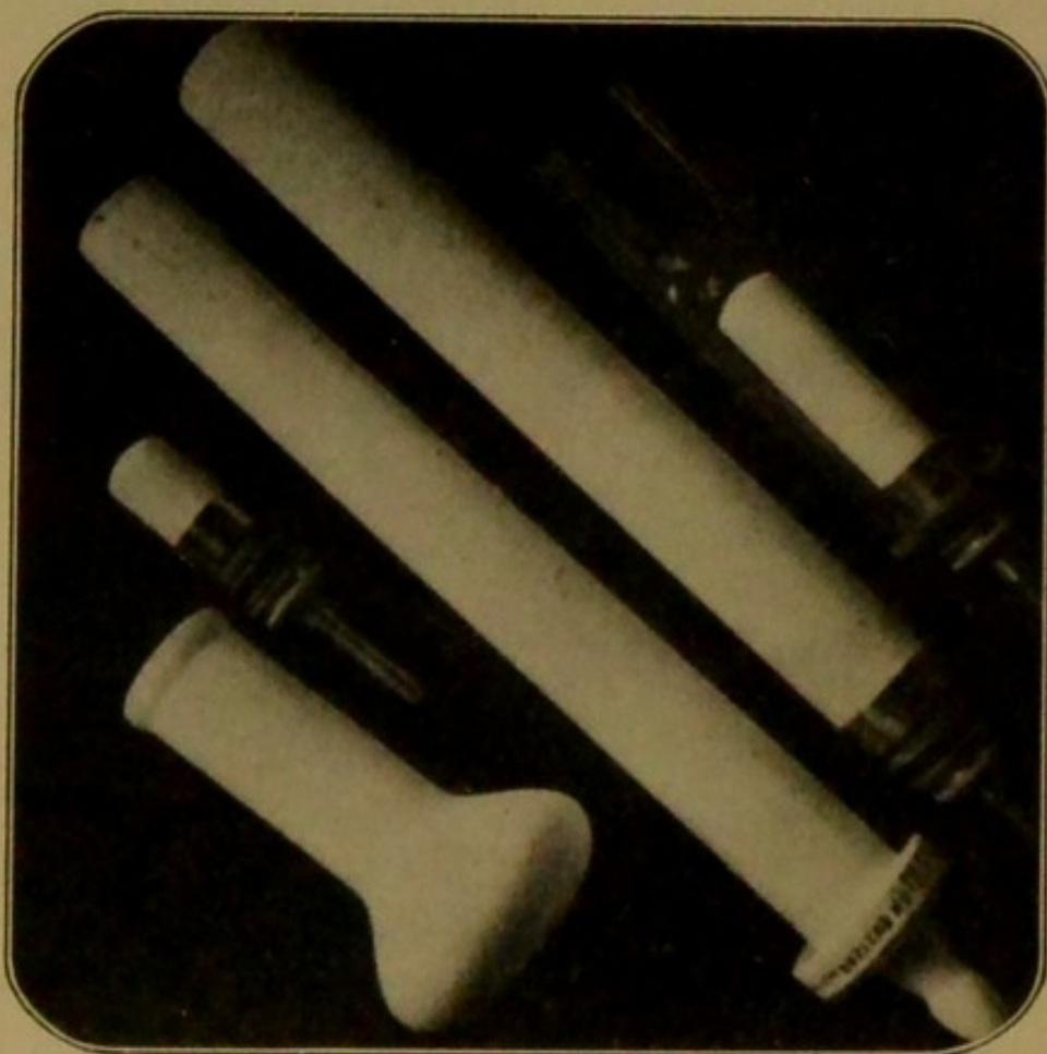
FIG. 90. Various types of porcelain filters for sterilization of liquids by filtration.
