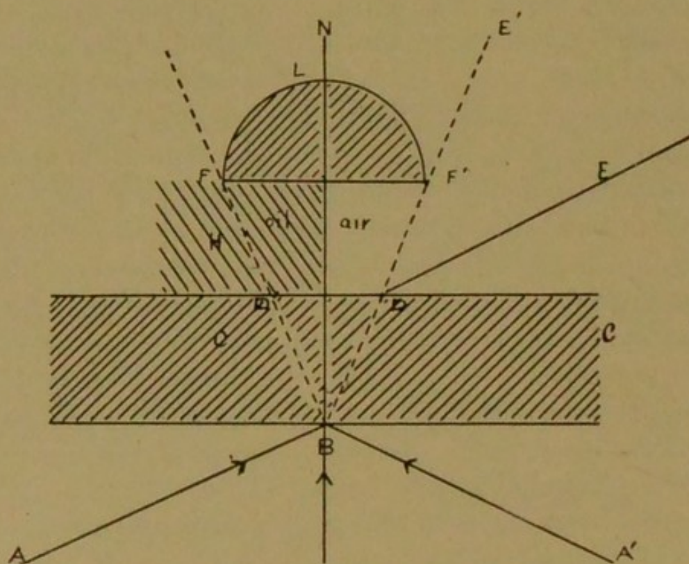
FIG. 114. Oil immersion lens, and object glass in diagrammatic longitudinal section. See text for lettering.
