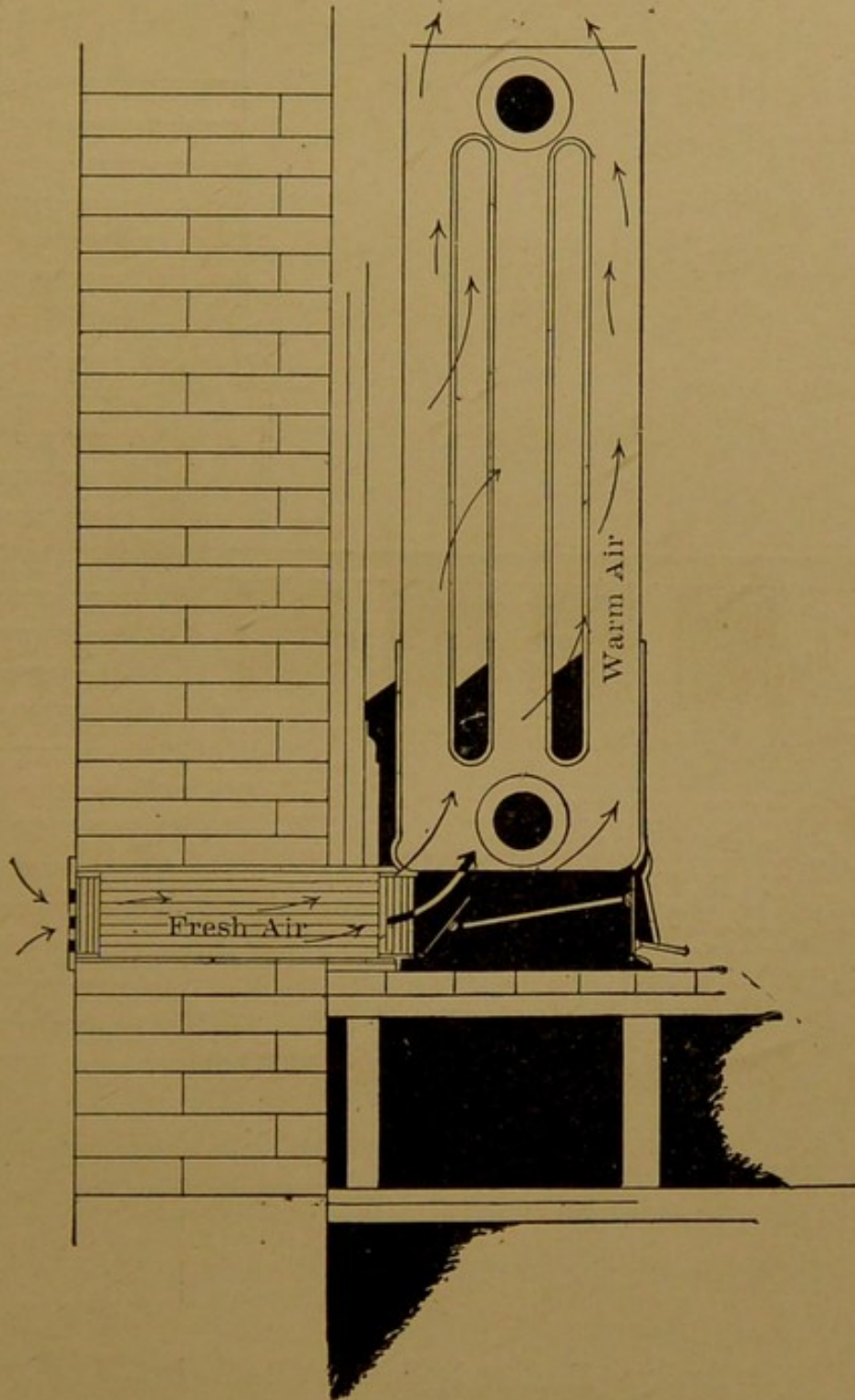
FIG. 6.—Heating by Direct-indirect Radiation.
