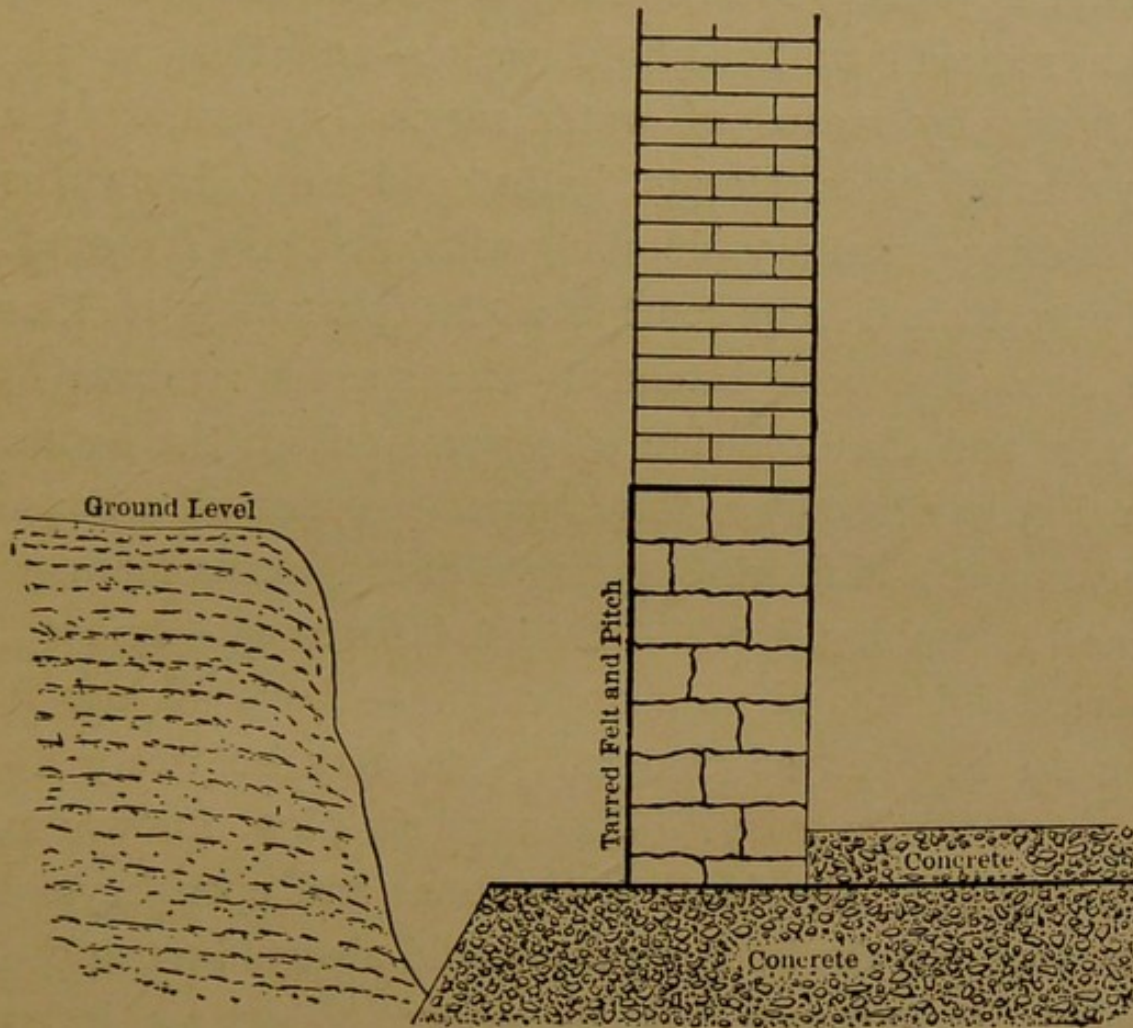
FIG. 1.—A Method of Constructing a Foundation.
