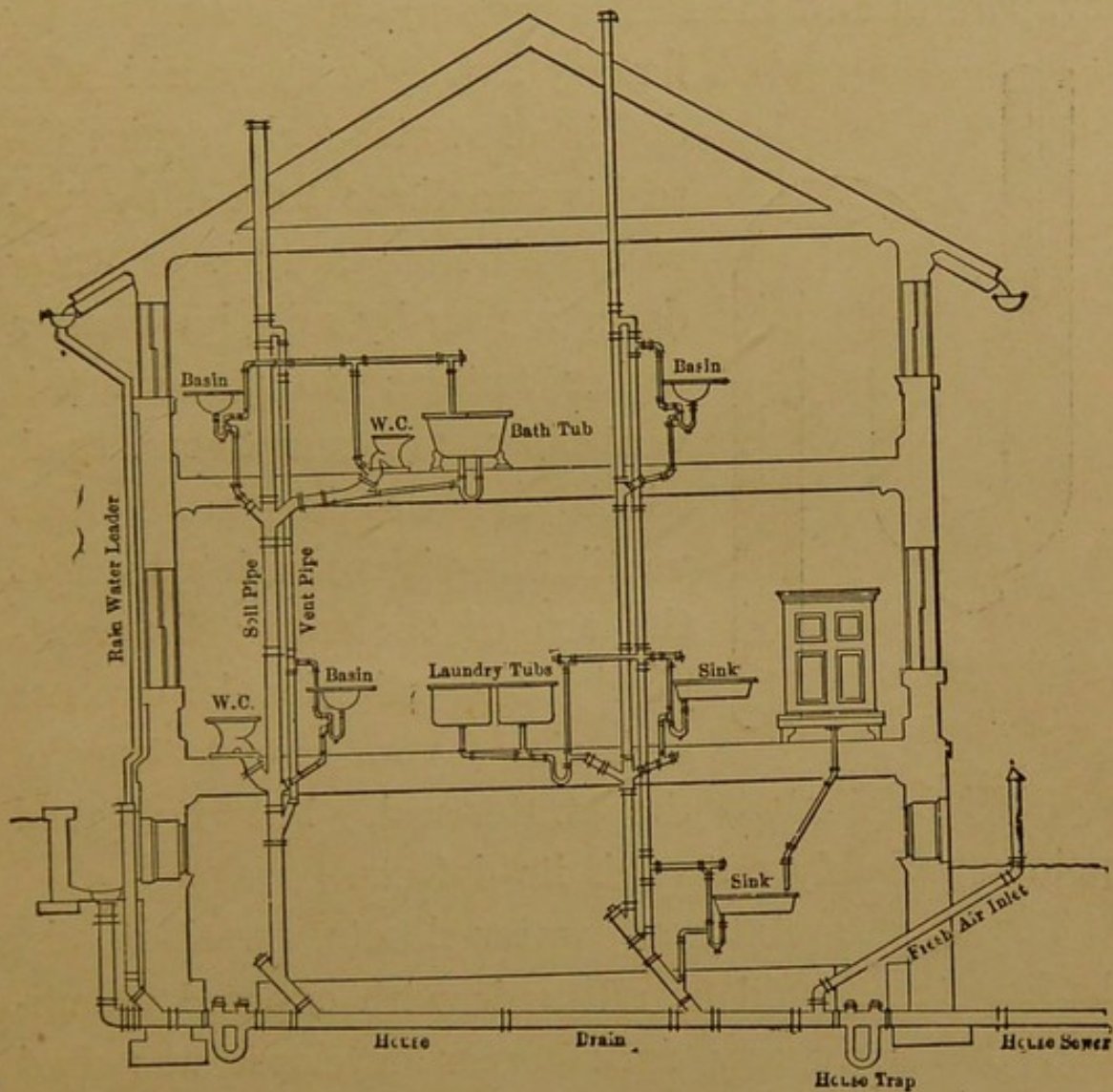
FIG. 2.—Section of a House, showing Plumbing System.
