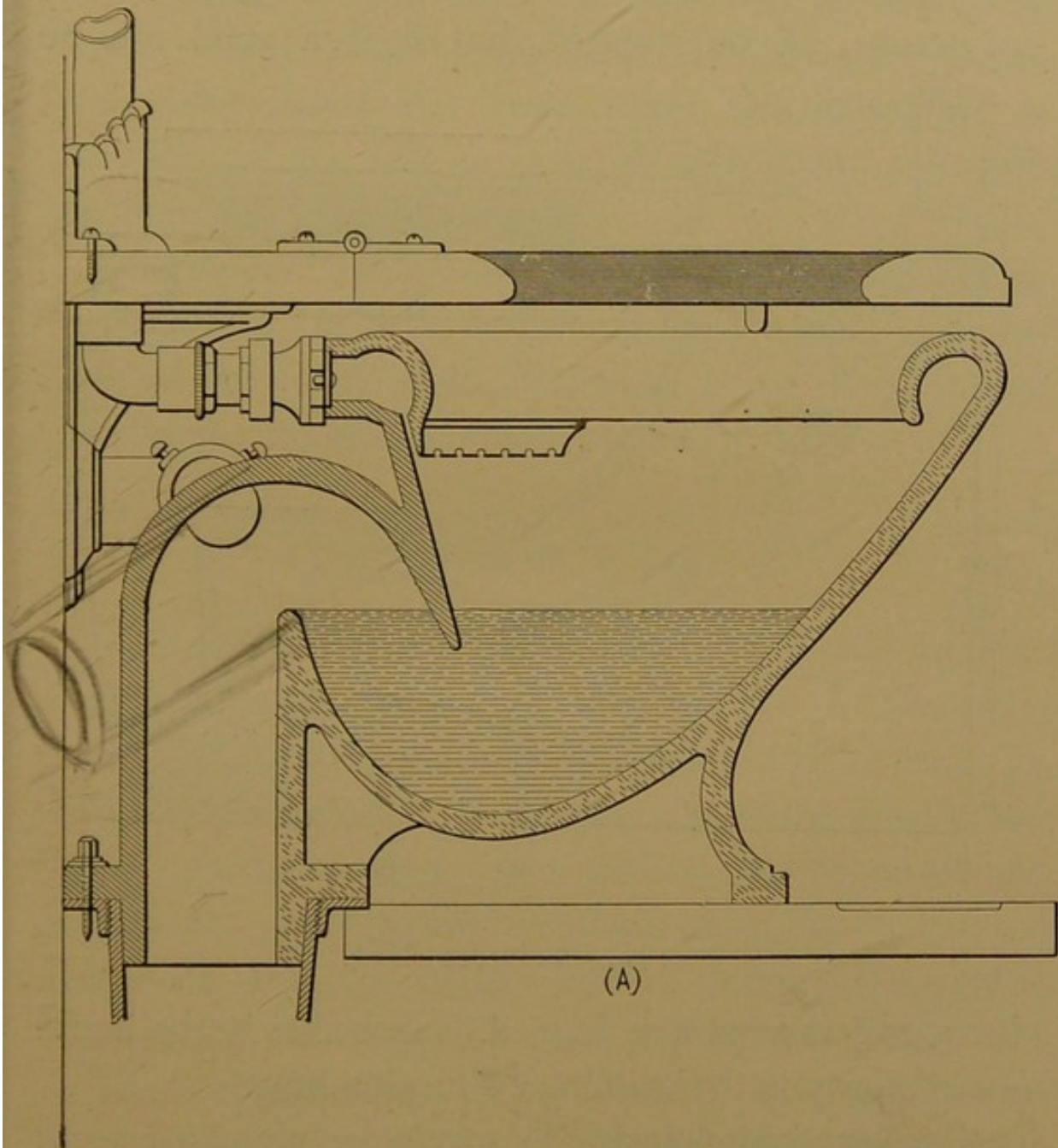
FIG. 5a.—Wash-down Closet.
