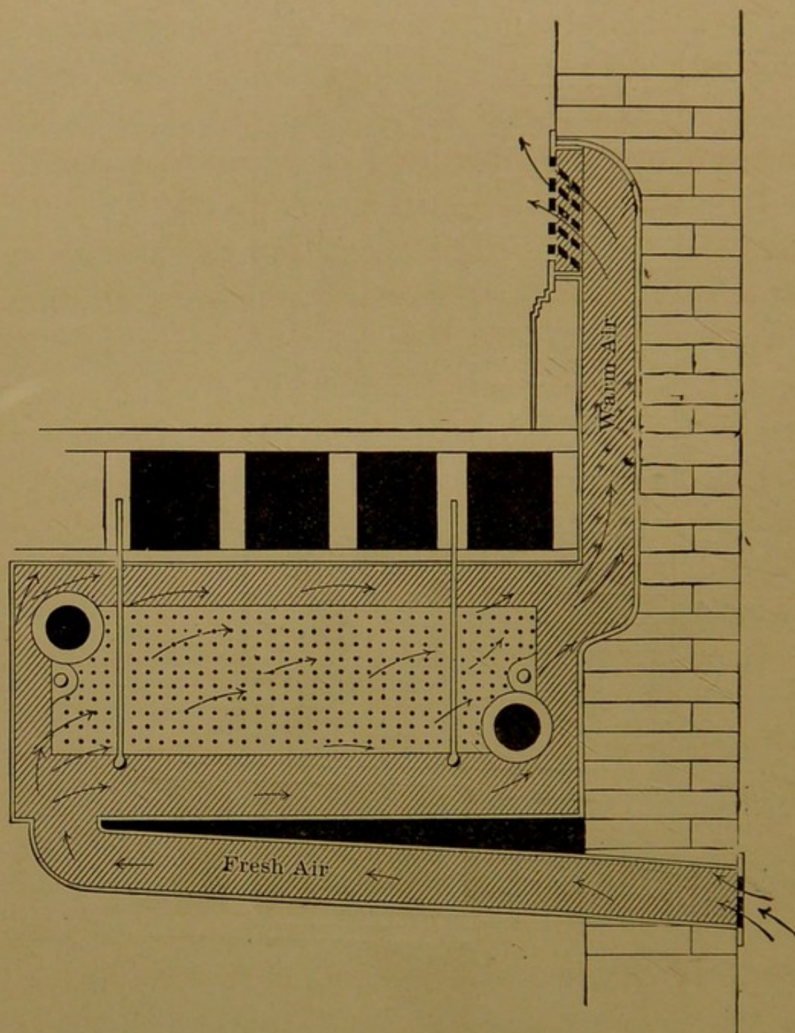
FIG. 7.—Heating by Indirect Radiation.
