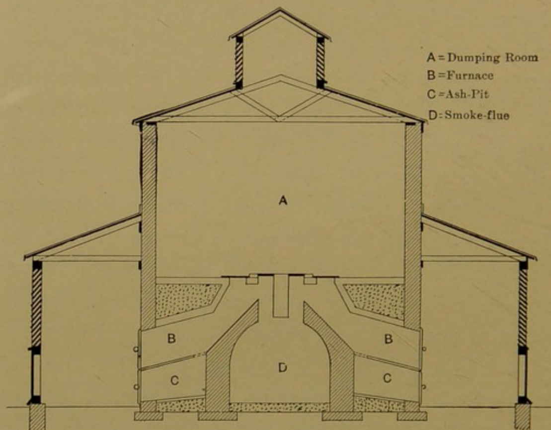
FIG. 20.—Section of Thackery Garbage-furnace.
