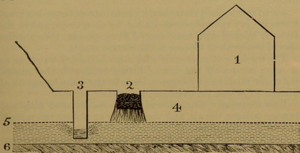
Fig. 25.—Pollution of shallow Well-water by Soakage from Cesspool.
