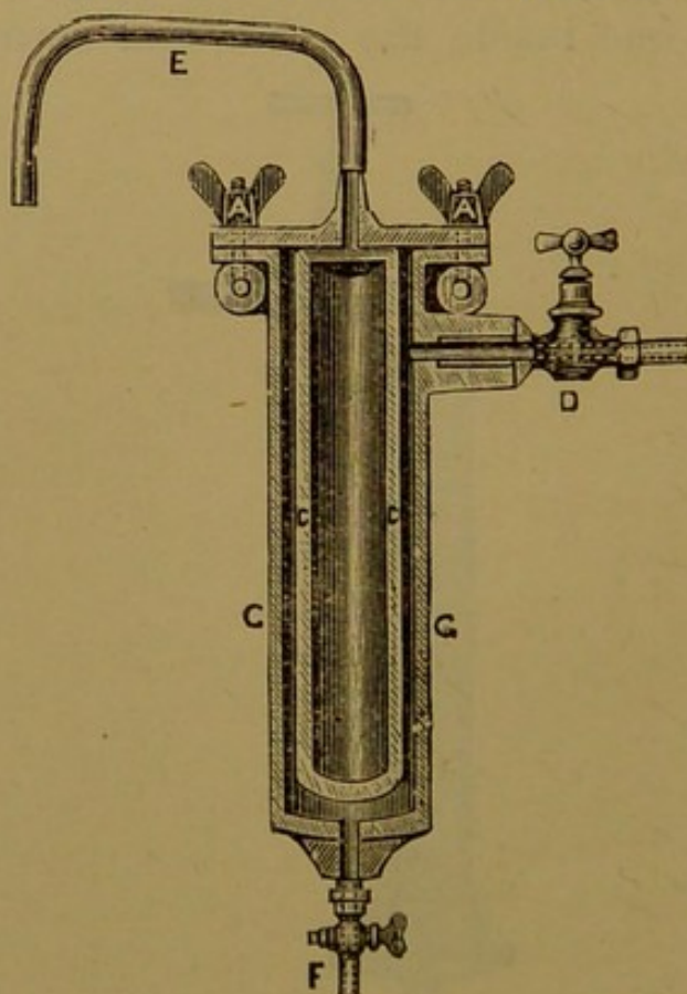
FIG. 71.—The Berkefeld tap filter.
