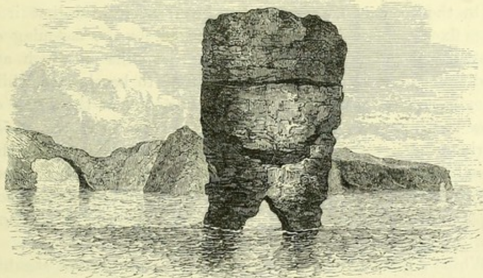
Torso Rock, near Point Deas Thomson, in the Arctic Ocean.
