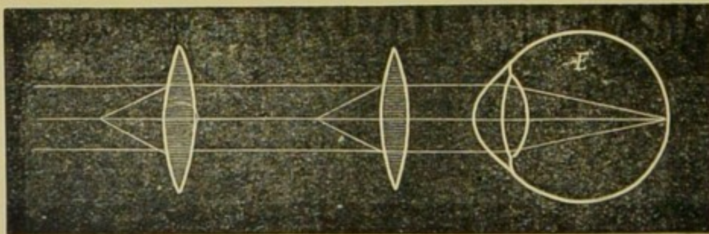
E. Emmetropic eye. Rays issuing parallel, image formed at the principal focus of the lens, no matter at what distance the lens is from the eye.
