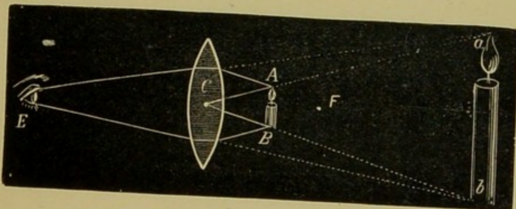
Virtual image formed by convex lens.
