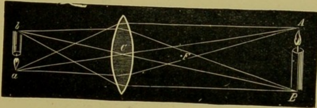
Real inverted image formed by convex lens.
