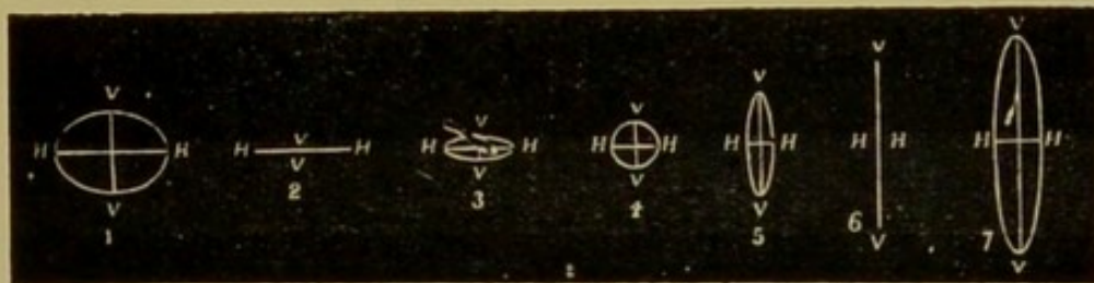
Section of cone of light at 1, 2, 3, 4, 5, 6, 7, Fig. 76.
