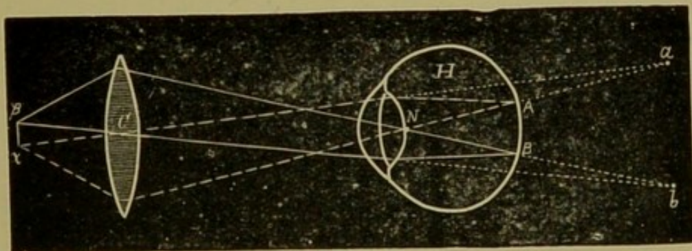
Lens at 12 cm. from the cornea.
