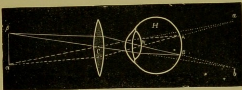
Lens at 4 cm. from the cornea.
