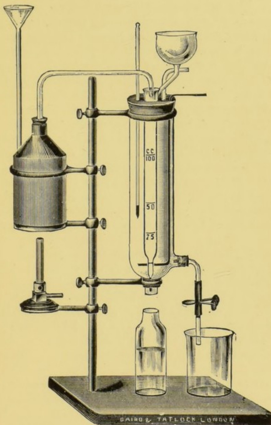
FIG. 18.—Coleman-Archbutt Viscometer.
