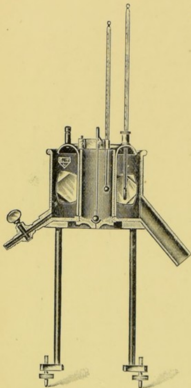
FIG. 15.—Section of the Redwood Viscometer.
