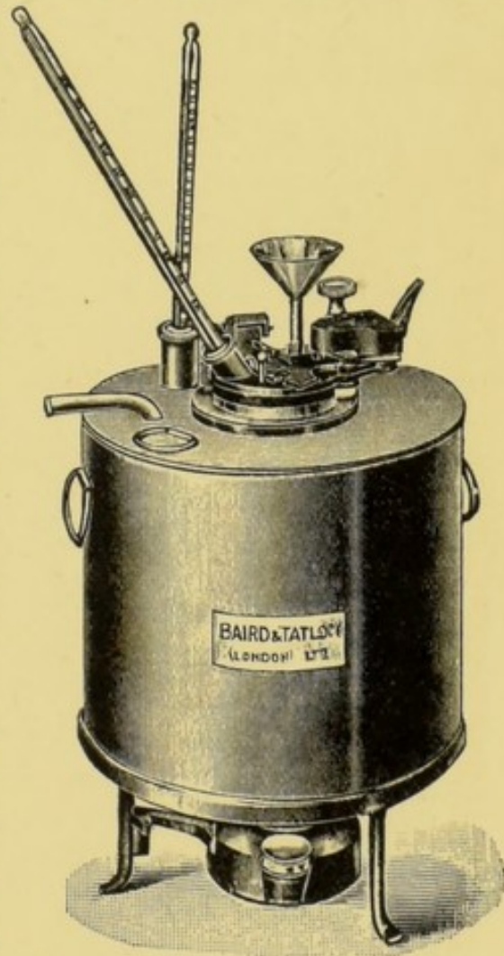
FIG. 9.—Abel-Pensky Petroleum Tester.
