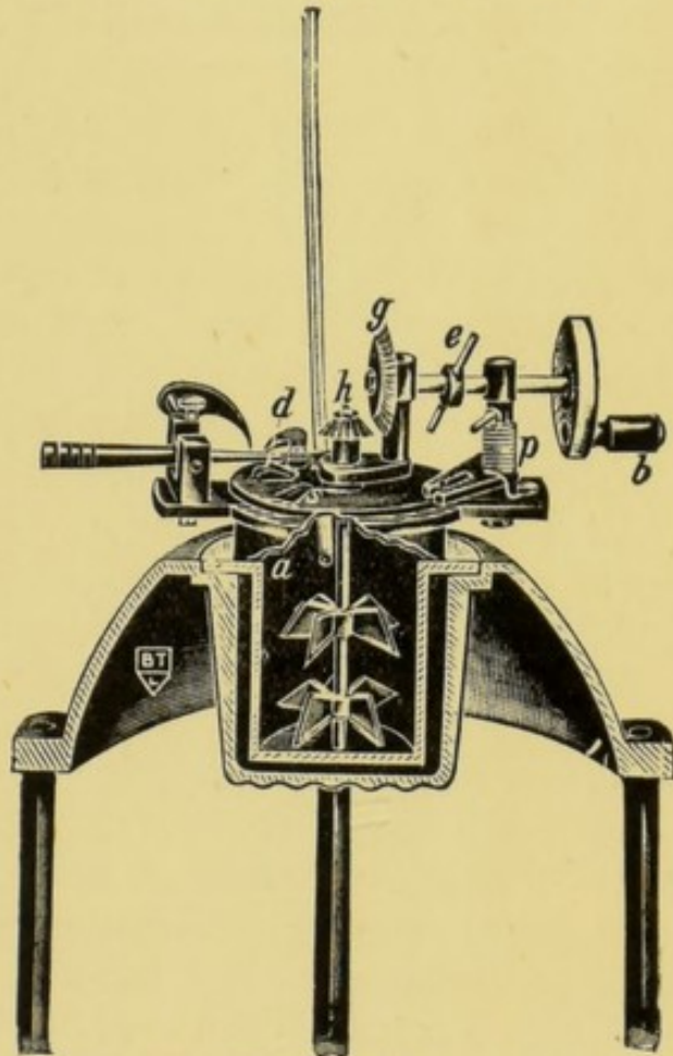
FIG. 13.—Section of Gray's Tester.
