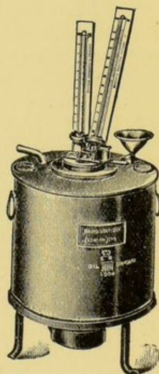
FIG. 7.—Abel Petroleum Tester.
