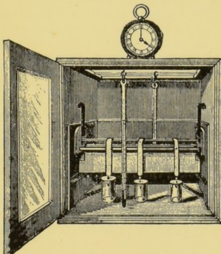
FIG. 28.—Redwood Apparatus for Capillary Test.
