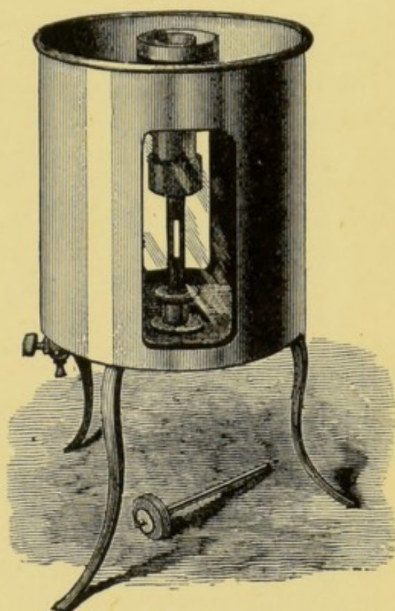
FIG. 17.—Saybolt Viscometer.
