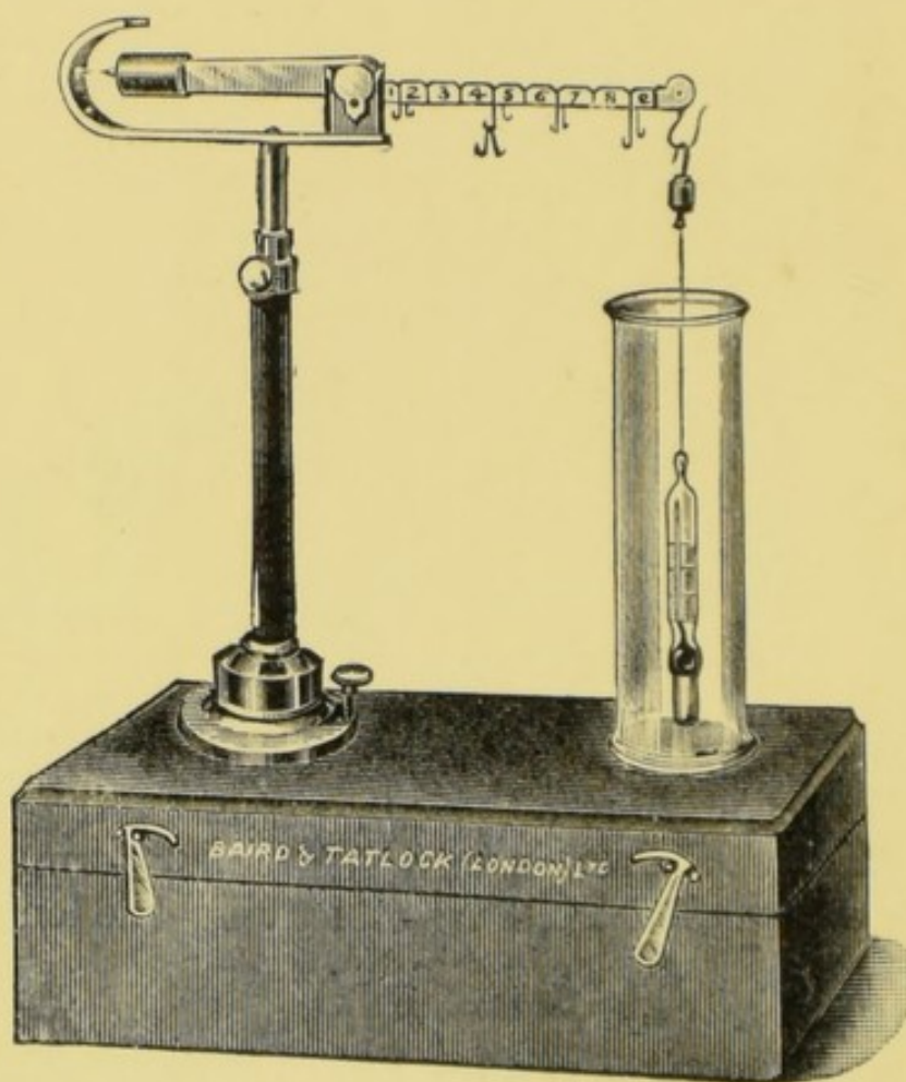
FIG. 5.—Westphal's Specific Gravity Balance.
