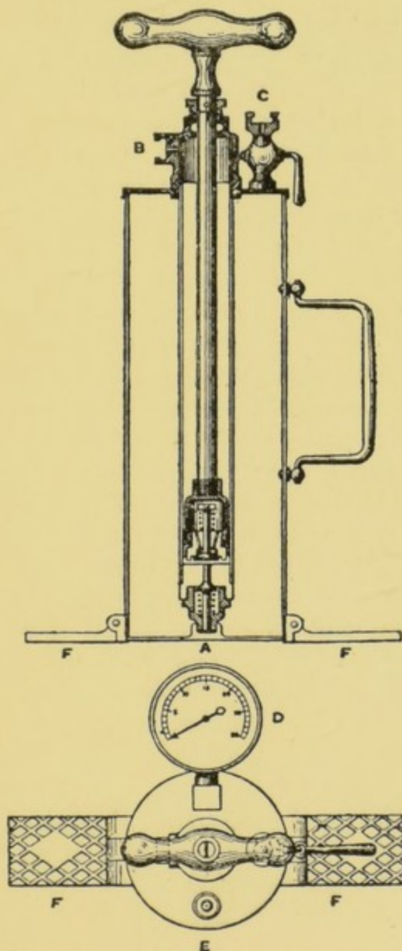
FIG. 26.—Apparatus for detecting Petroleum Vapour.
