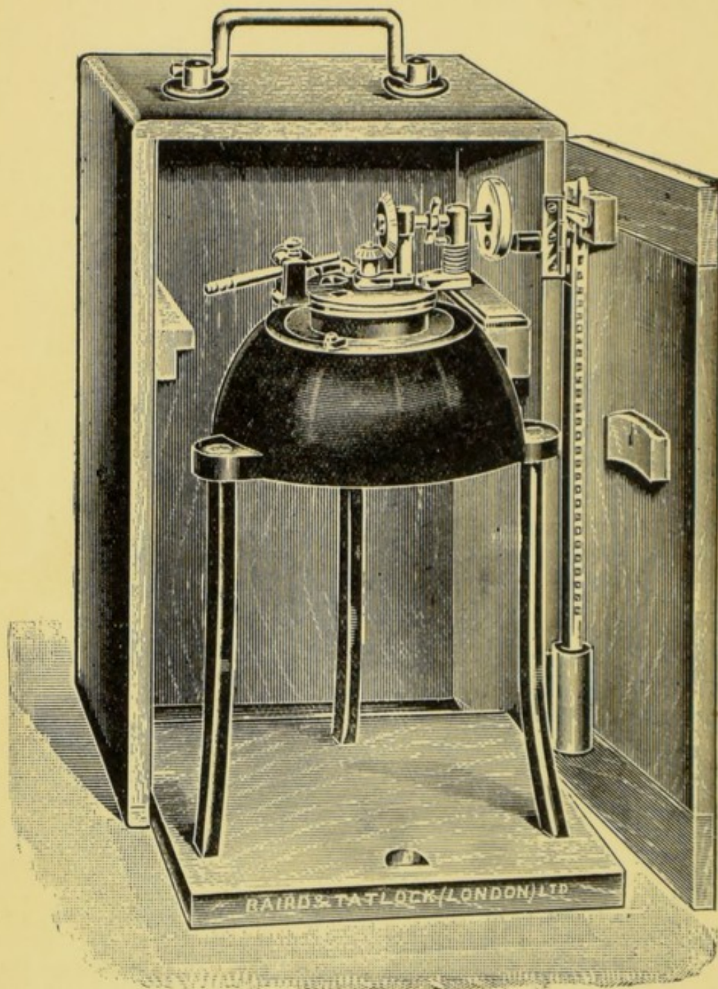
FIG. 12.—Gray's Tester.
