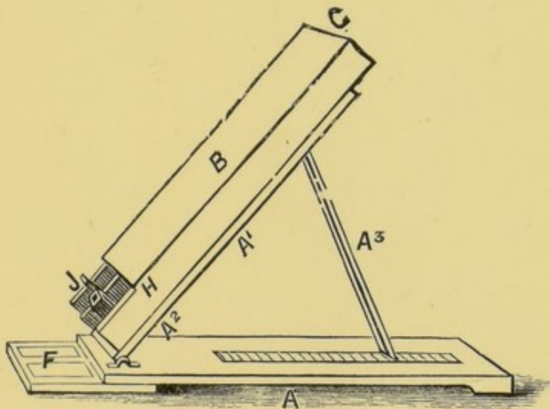
FIG. 21.—Lovibond's Tintometer.
