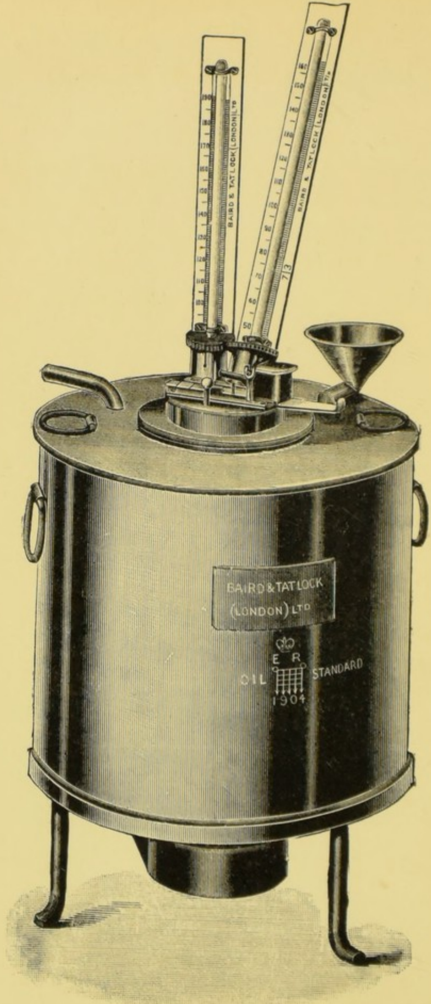
Abel Petroleum Testing Apparatus.
