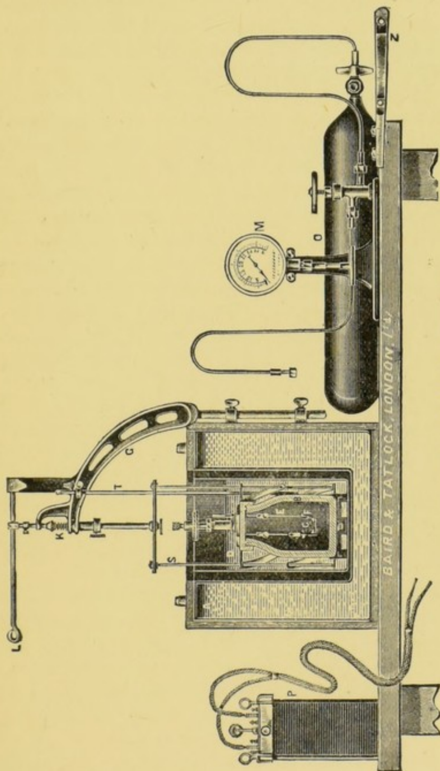
FIG. 31.—Mahler Calorimeter.
