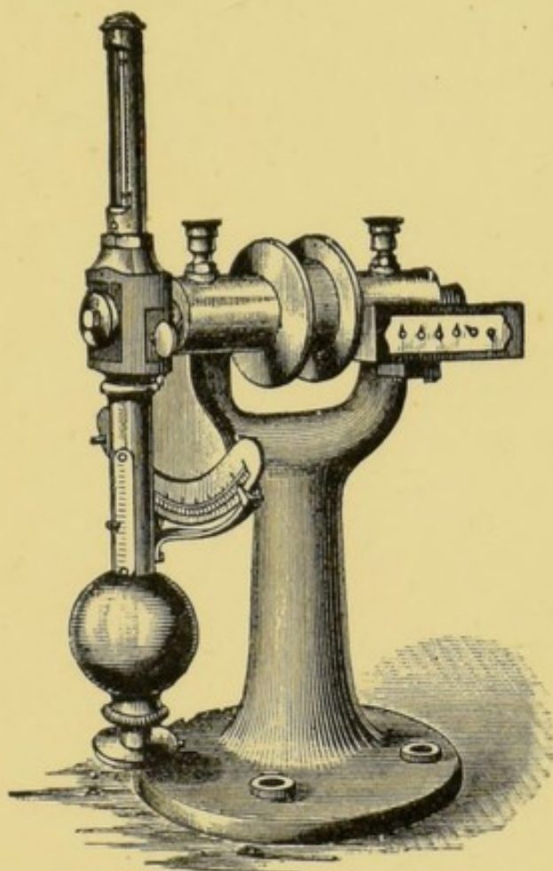
FIG. 19.—Thurston's Oil Tester.
