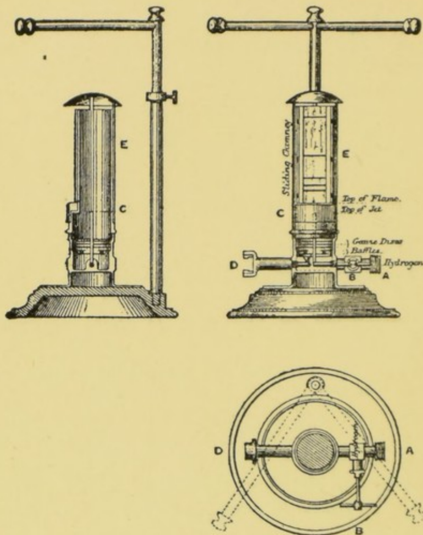
FIGS. 24 and 25.—Apparatus for detecting Petroleum Vapour.
