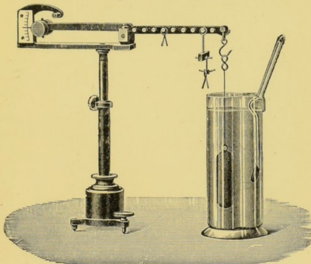
FIG. 6.—The Sartorius Specific Gravity Balance.
