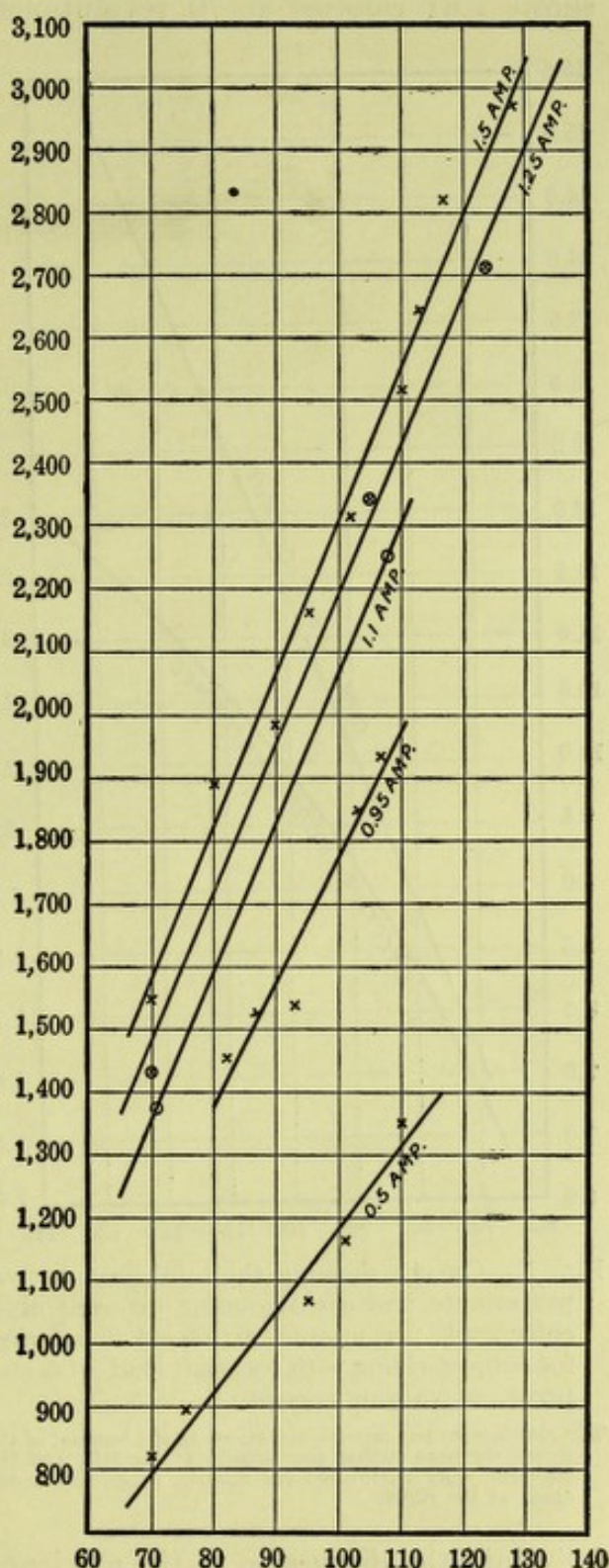
FIG. 4.—Curves showing oxygen consumption per minute with the subject riding at different speeds and with varying loads.
