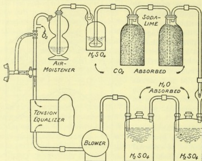
FIG. 2.—Schematic outline of the respiration apparatus.
