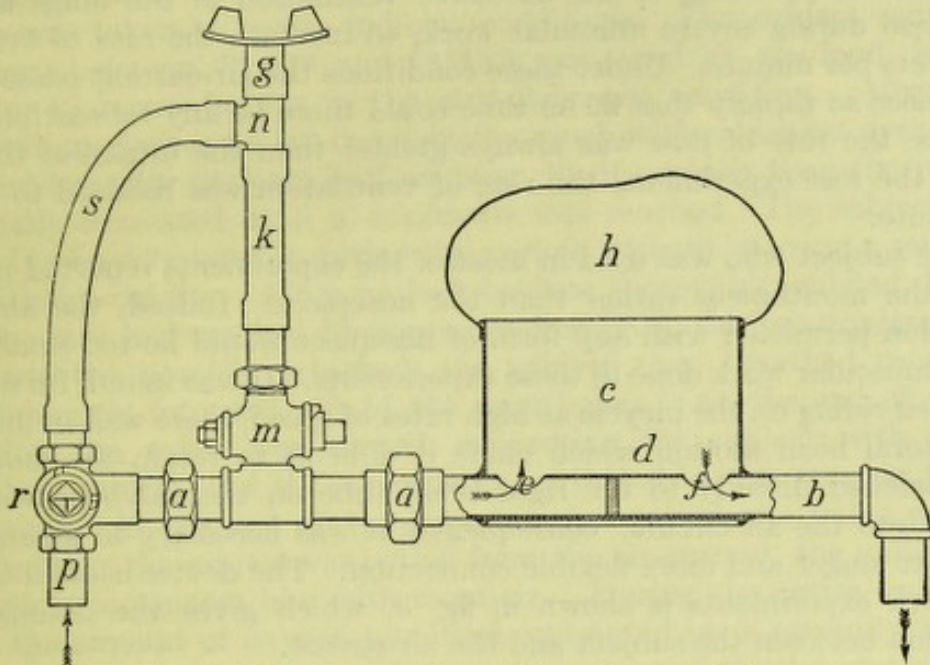
FIG. 3.—Tension-equalizer and flexible mouthpiece.
