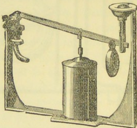
FIG. 43.—Water-closet Supply Valve with Bellows Regulator.
