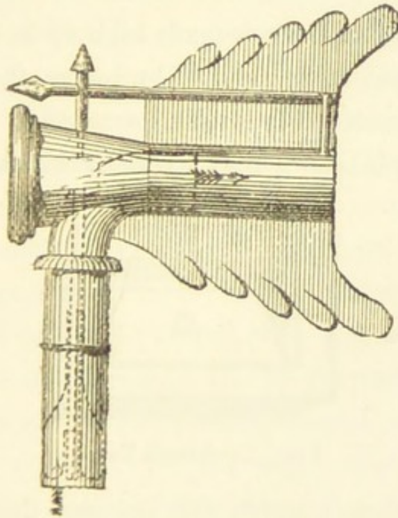
FIG. 11.—Revolving Cowl.
