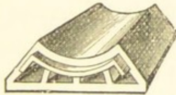
FIG. 26.—Invert Block.
