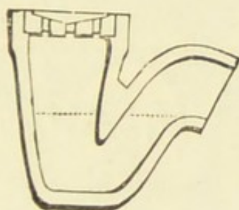
FIG. 29.—Stoneware Siphon Gully.
