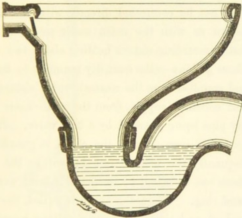
FIG 34.—Short hopper water-closet.
