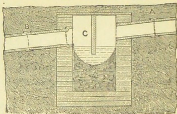
FIG. 28.—Dipstone Trap. AB. Drain. C. Dipstone.
