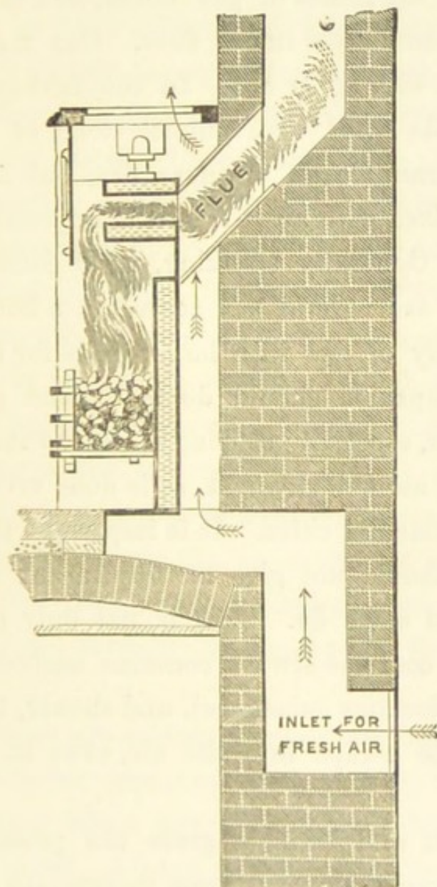
FIG. 17.—Thermhydric Grate (Section).
