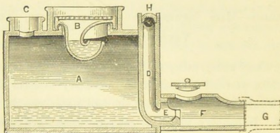
FIG. 24.—Field's Flush Tank.
