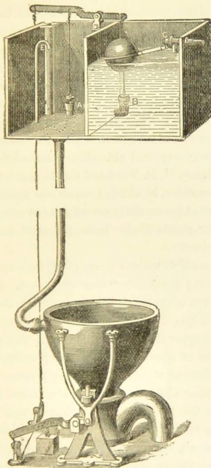
FIG. 25.—Hopper water closet with water-waste-preventing cistern and seat-action arrangement.
