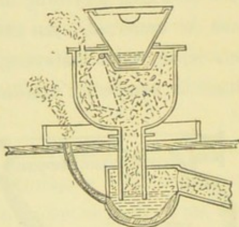
FIG. 37.—Pan Water Closet.
