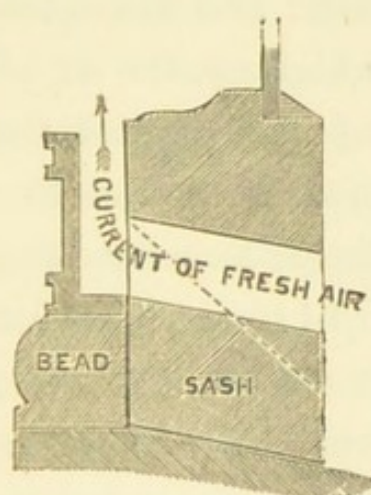
FIG. 4.—Currall Ventilator (as fixed to Window).
