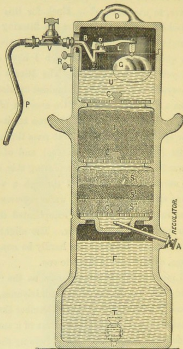
FIG. 21.—Spongy Iron Filter.
