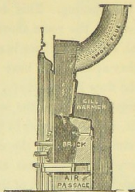
FIG. 14.—The Galton Ventilating Grate.
