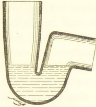
FIG. 39.—"Anti-D" Trap.
