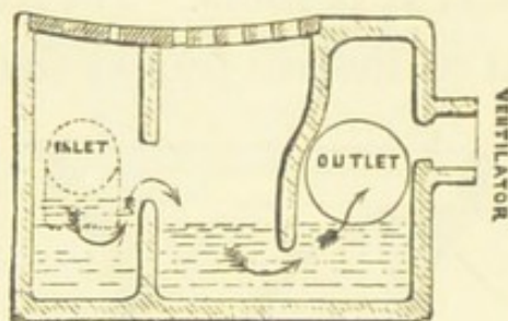
FIG 32.—Mansergh Trap.
