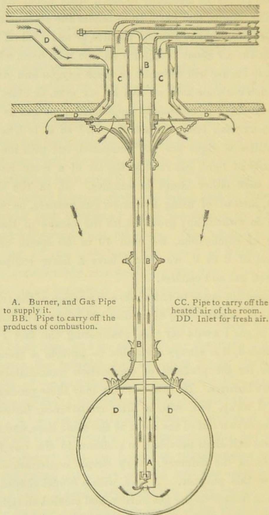
FIG. 13.—Ventilating Globe Light.
