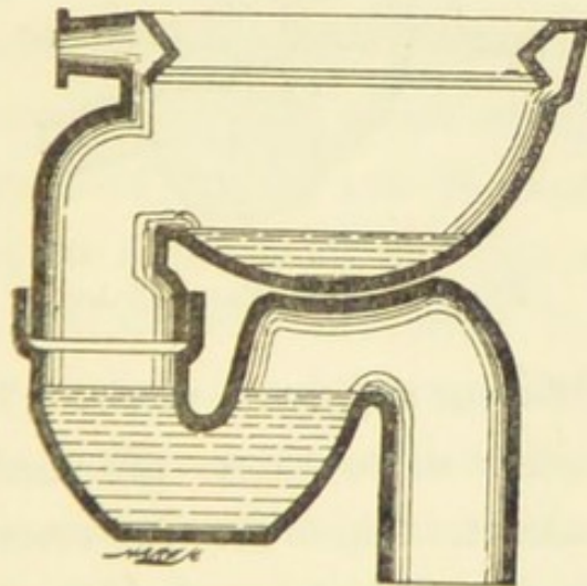
FIG. 36.—"Wash-out" Water Closet.
