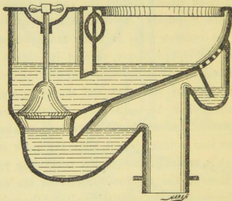
FIG. 41.—Plug Closet.
