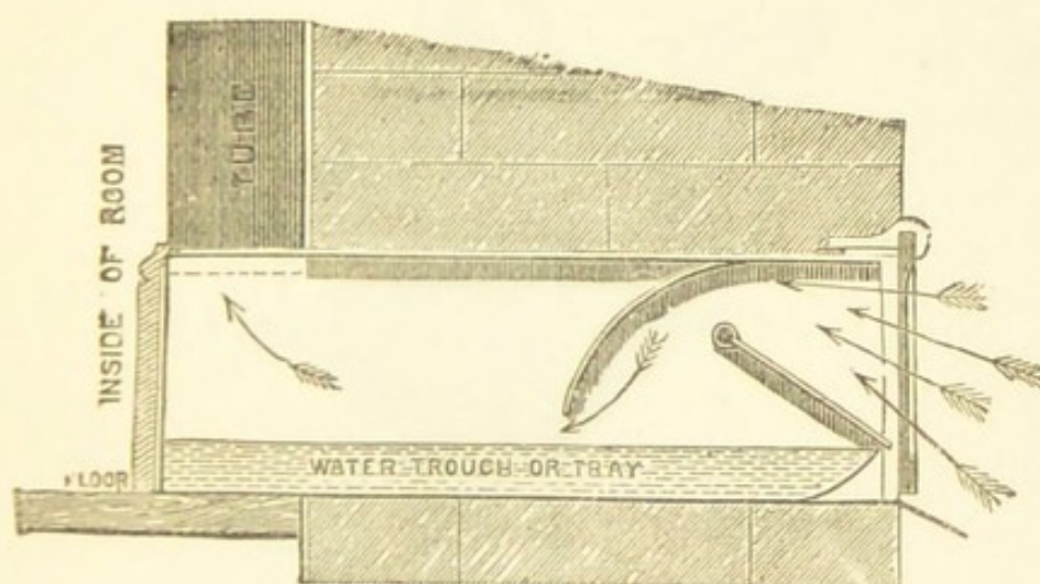
FIG. 9.—Water Tray for Vertical Tube Ventilator.
