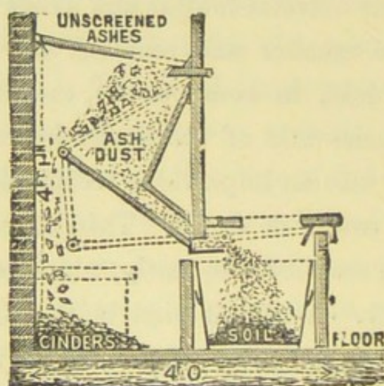
FIG. 23.—Cinder Sifting Ash Closet.
