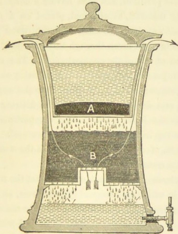
FIG. 22.—Aërating Filter.
