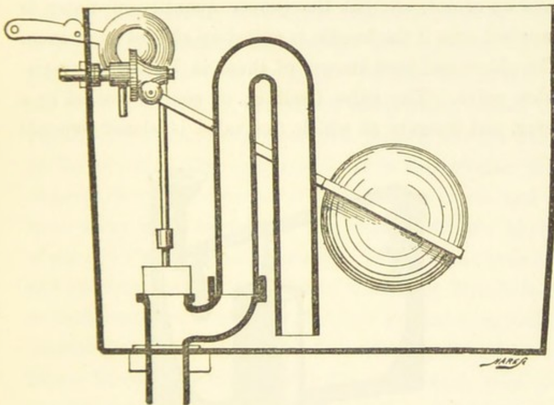
FIG. 42.—Siphon-action water-waste-preventer.
