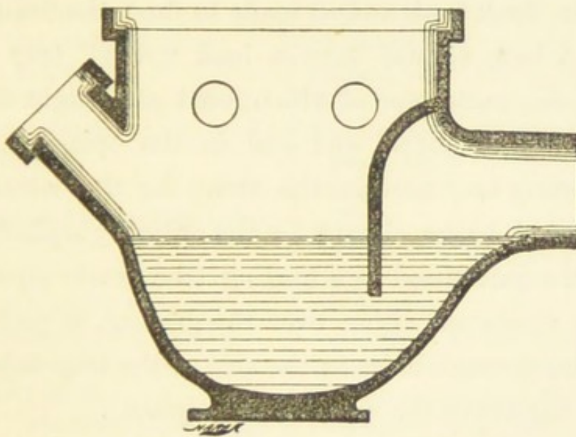
FIG. 45.—Flushing gully.
