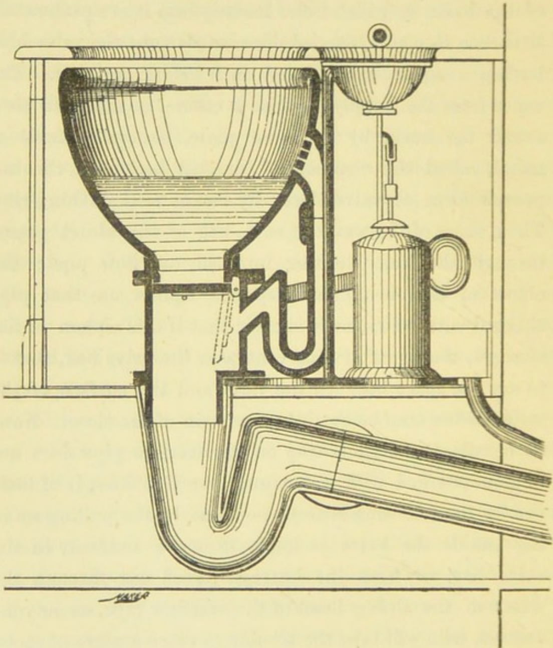
FIG. 40.—Valve Water Closet and "Anti-D" Trap.
