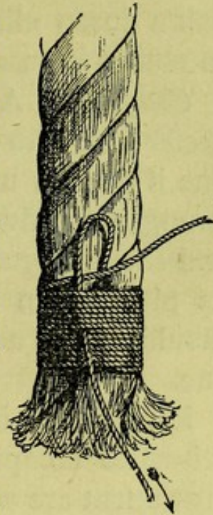
HOW TO WHIP A ROPE END.
