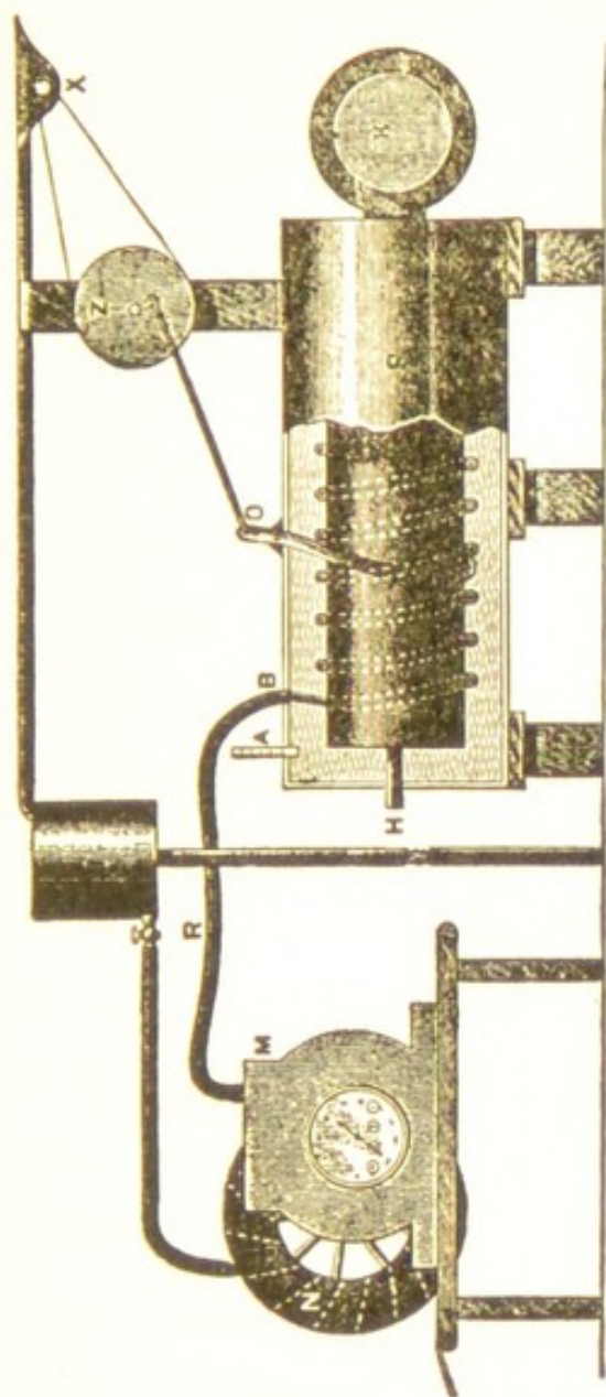
Fig. 11. Ott's Calorimeter for man.
