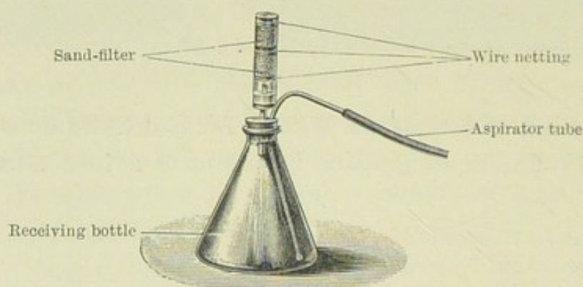
FIG. 33.—PETRI'S SAND-FILTERING APPARATUS.
