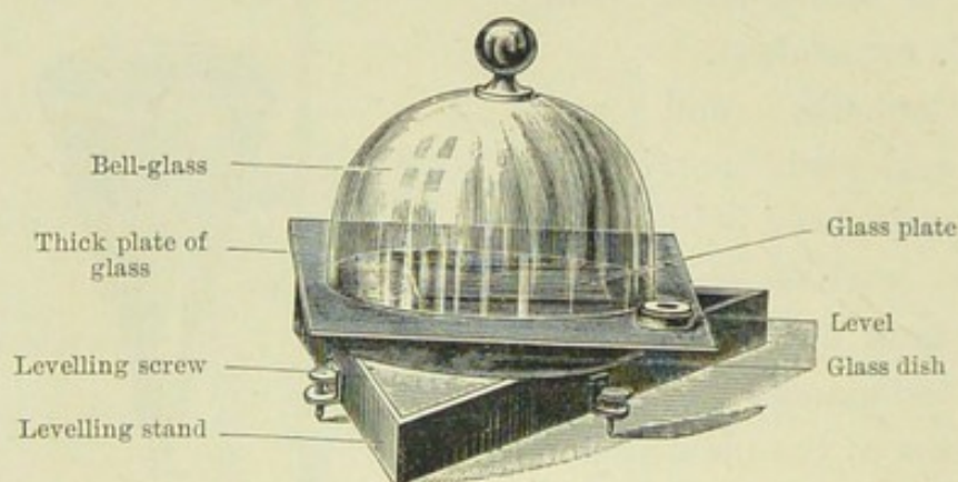
FIG. 16.—LEVELLING APPARATUS FOR MAKING PLATE-CULTIVATIONS.
