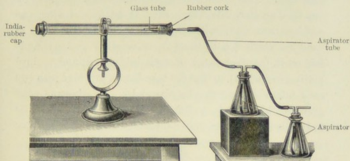
FIG. 31.—HESSE'S APPARATUS FOR EXAMINING AIR.
