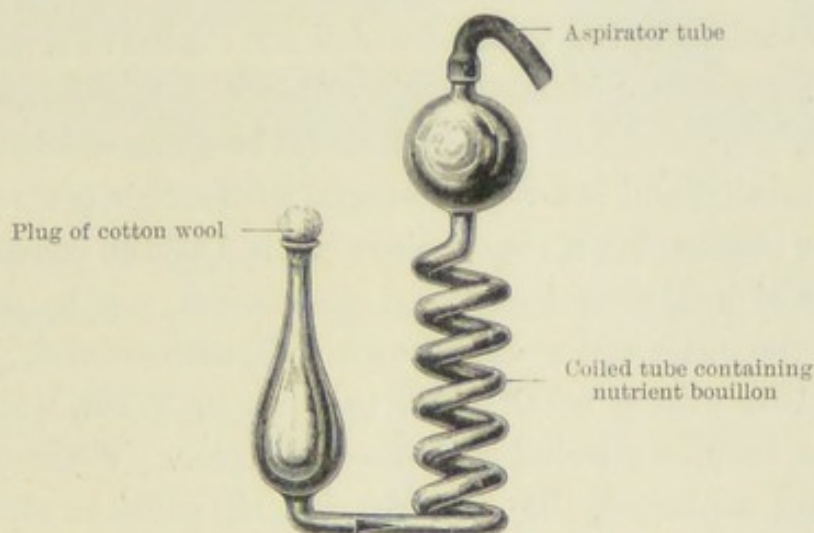
FIG. 30.—EMMERICH'S APPARATUS FOR EXAMINING AIR.
