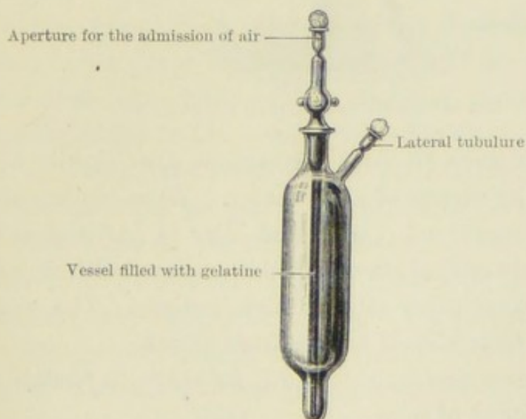
FIG. 32.—AIR-TESTING APPARATUS OF STRAUSS AND WÜRZ.
