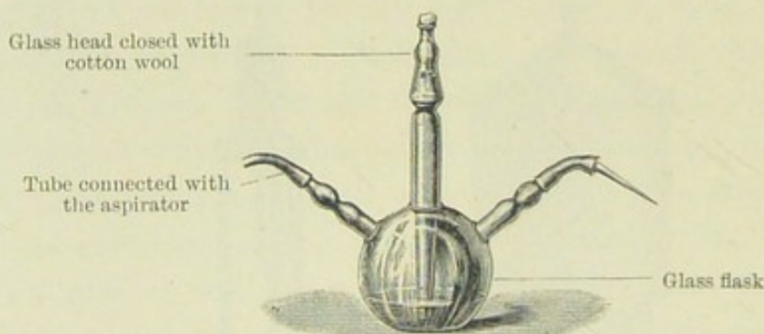
FIG. 29.—MIQUEL'S APPARATUS FOR EXAMINING AIR.
