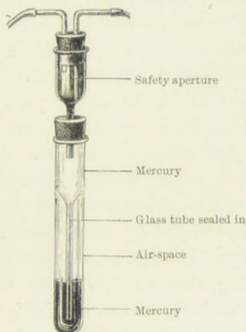
FIG. 12.—SCHENK'S THERMO-REGULATOR.
