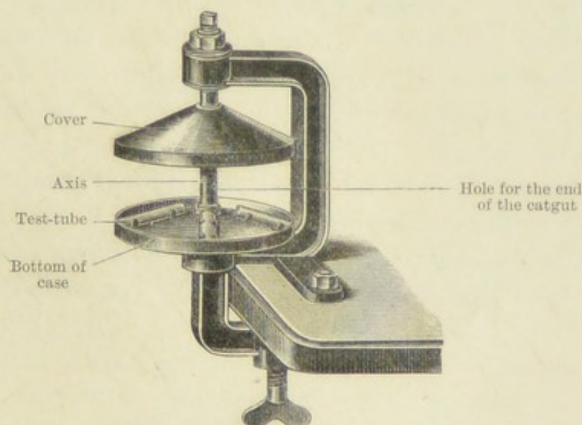
FIG. 21.—GÄRTNER'S CENTRIFUGE.
