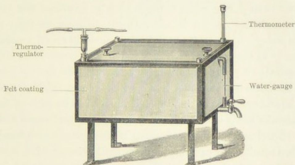
FIG. 11.—INCUBATOR.
