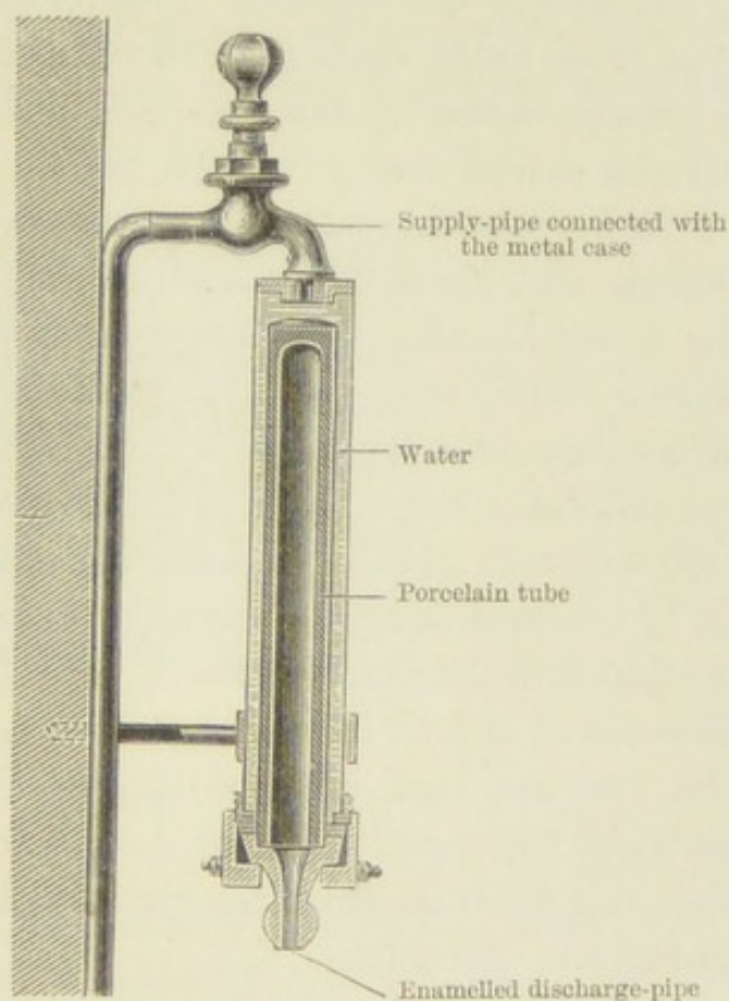
FIG. 44.—KAOLIN FILTER, ON THE CHAMBERLAND-PASTEUR SYSTEM.
