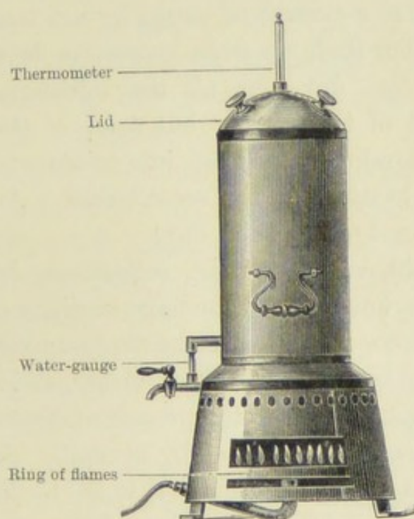
FIG. 10.—Koch's STEAM STERILISER.
