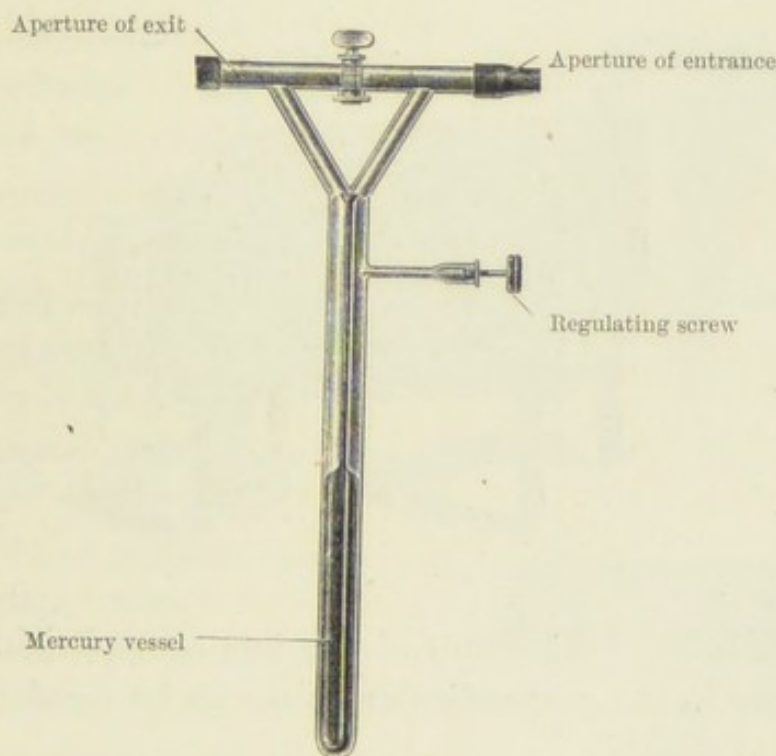
FIG. 13.—ALTMANN'S THERMO-REGULATOR.
