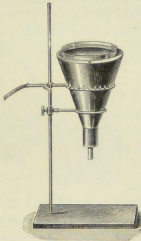
FIG. 15.—HOT-WATER FILTER (HEATED BY A RING BURNER).
