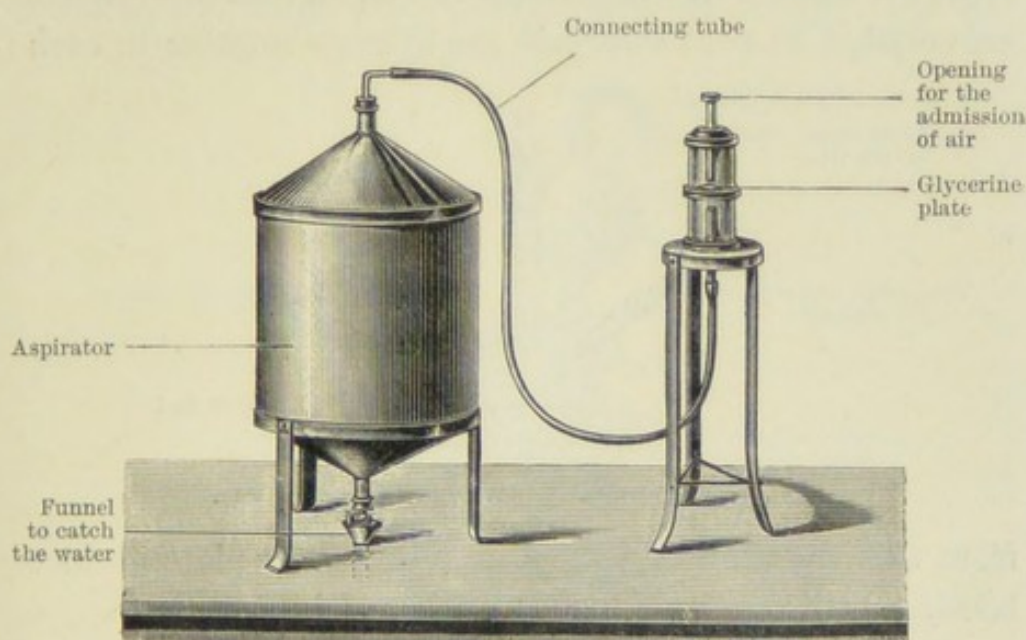
FIG. 28.—POUCHET'S AËROSCOPE.
