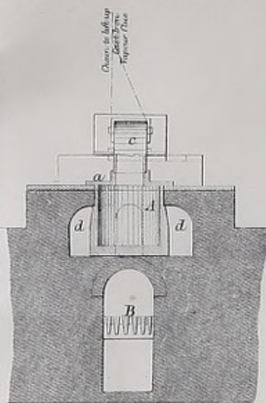
Vertical Section
