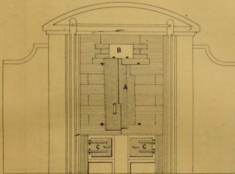
FRONT ELEVATION.
