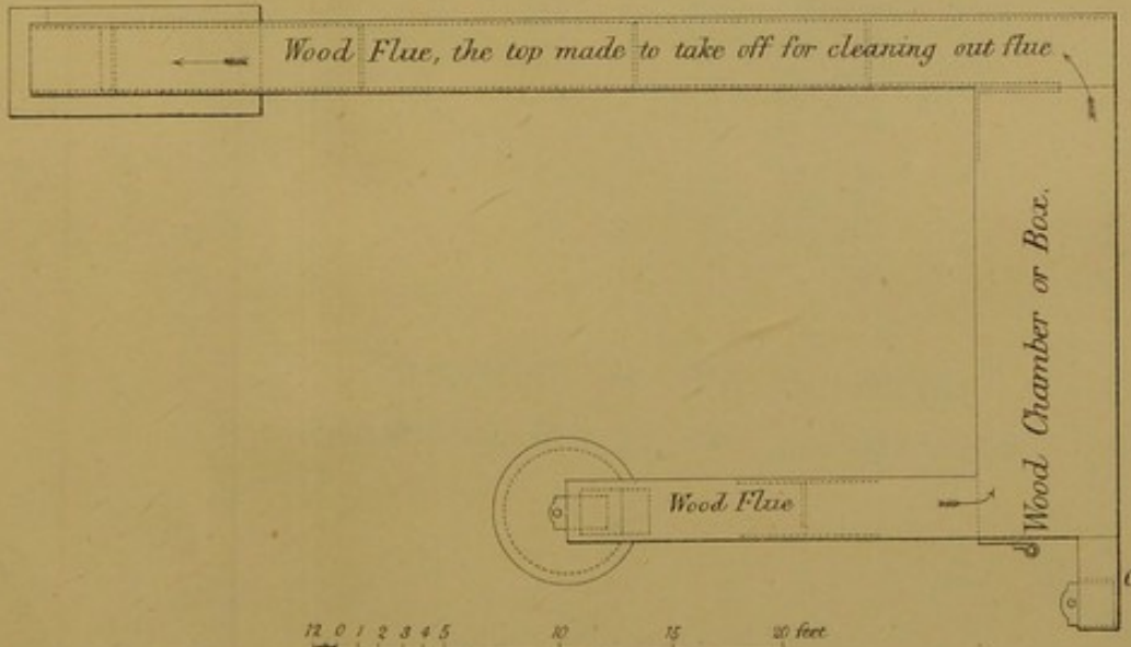
GROUND PLAN.
