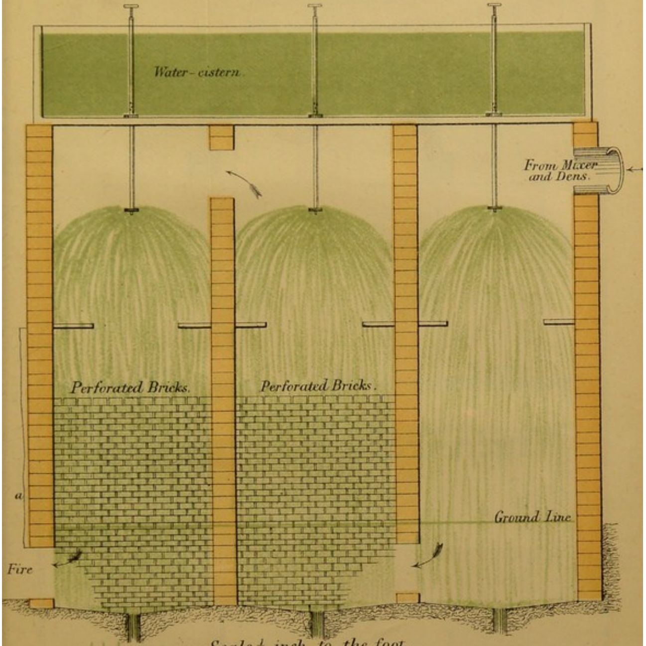
Scale \frac{1}{4} inch to the foot.
