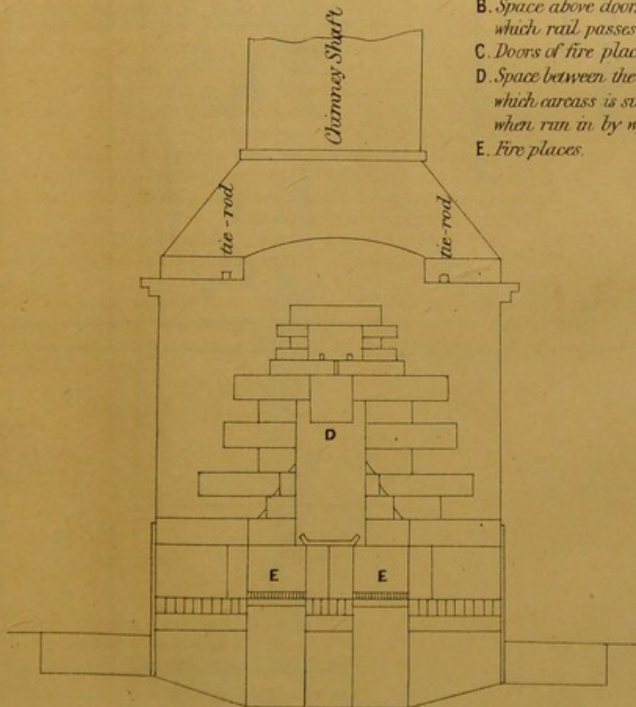
TRANSVERSE SECTION.
