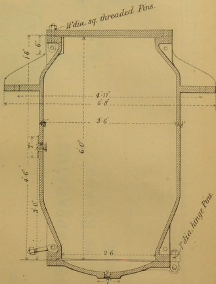
VERTICAL SECTION.
