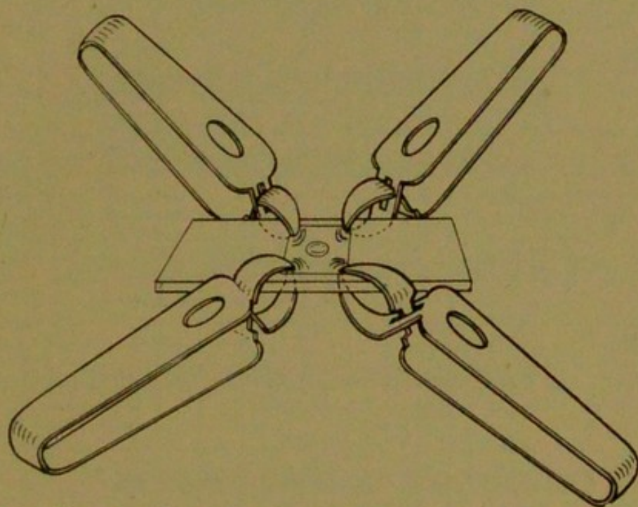
FIG. 42.—COUNTING CHAMBER WITH COVER-GLASS CLIPPED INTO POSITION.
