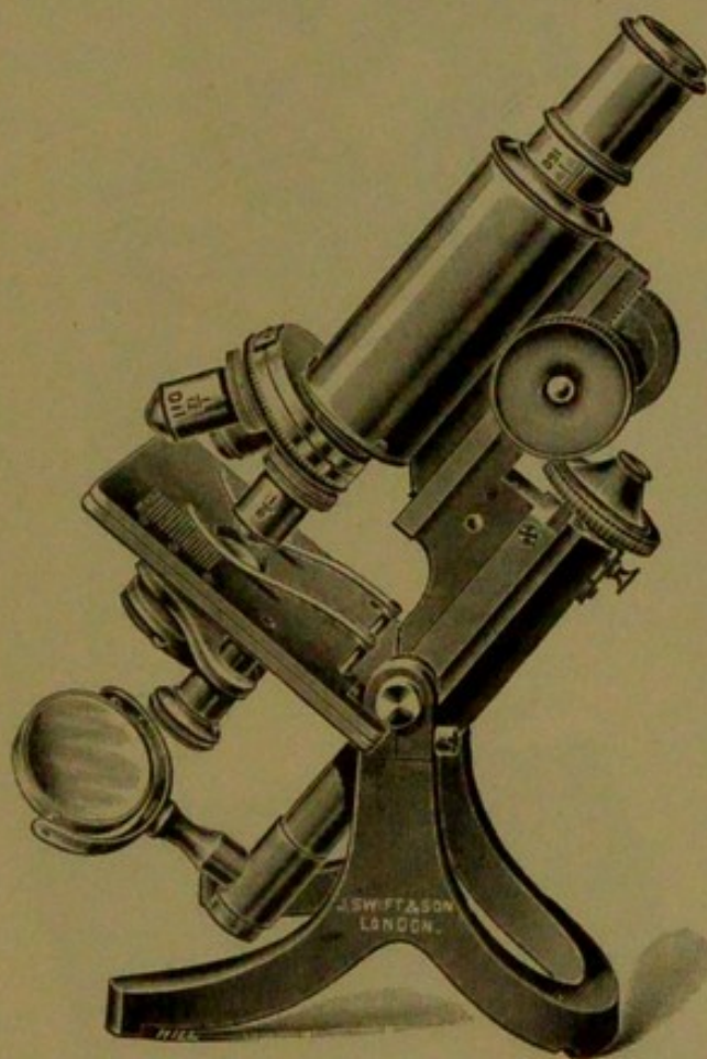
FIG. 2.—BACTERIOLOGICAL MICROSCOPE.
