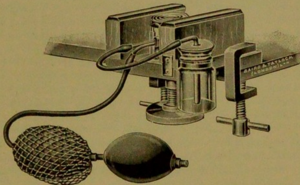
FIG. 36.—CATHCART'S MICROTOME ARRANGED FOR CUTTING FROZEN SECTIONS.
