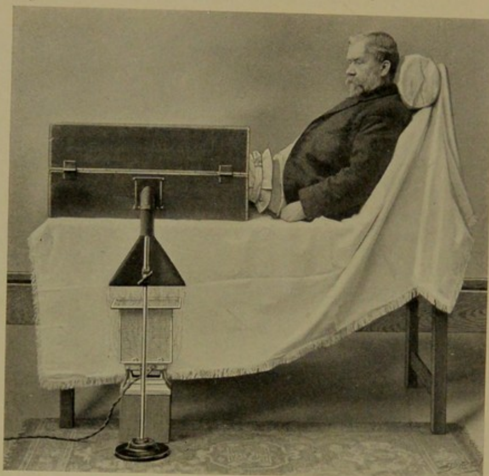
Fig. 60.—Shows the hot-air chamber for the whole leg. Here again the source of heat is an electric stove, an arrangement which simplifies matters considerably.
