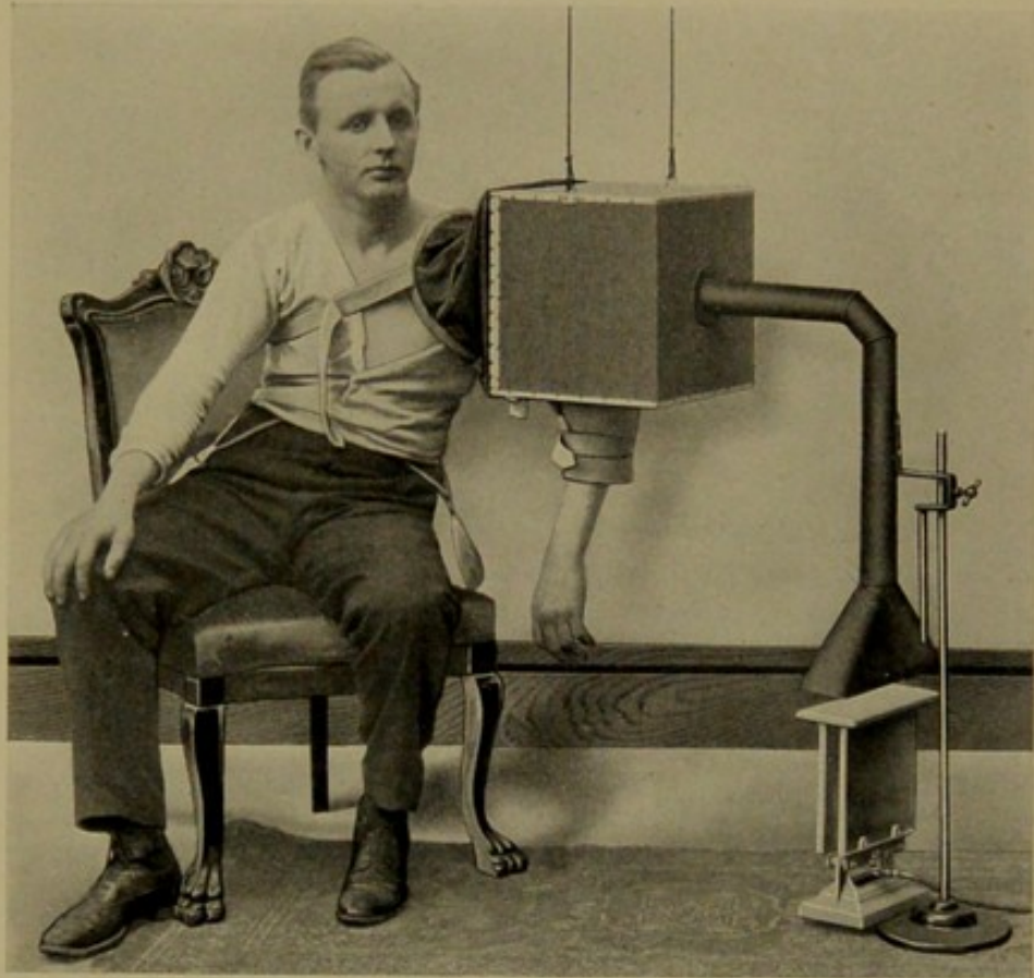
Fig. 56.—Shows the hot-air box for the shoulder; apparatus is suspended from the ceiling, an arrangement which enables the surgeon to use the same apparatus for either side. This is easily done by reversing the chair. This arrangement will be found especially useful in dispensaries, or in the offices of physicians who practise in places where institutes for hot-air treatment are not at their disposal.
