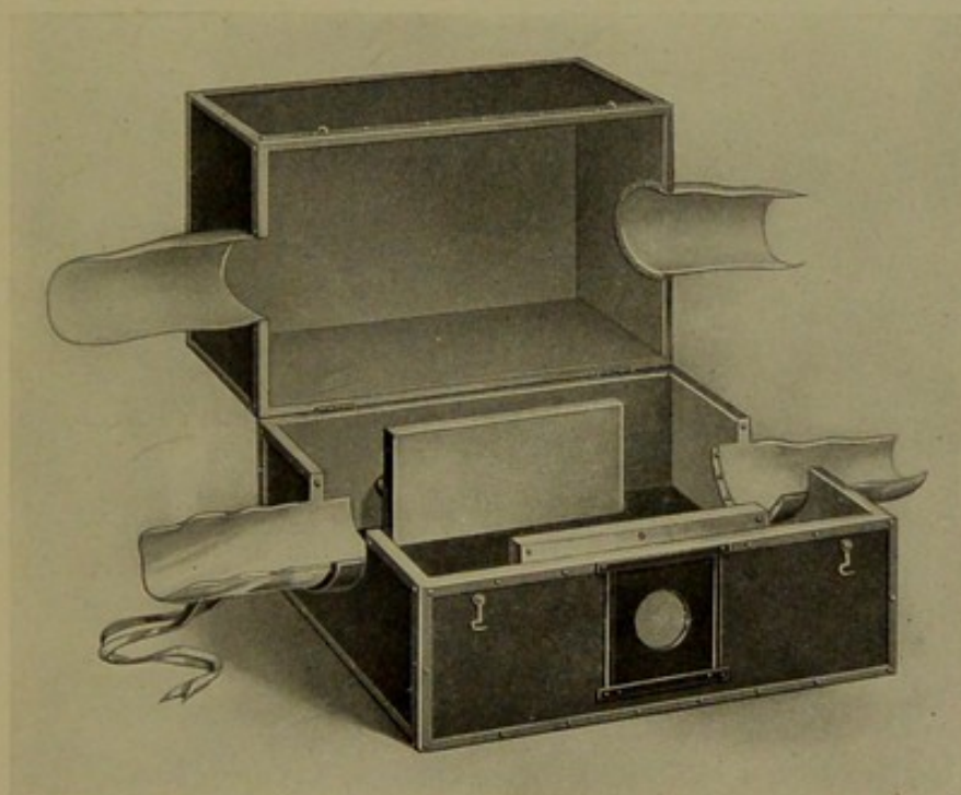
Fig. 53.—Hot-air box, open. Note the board on either side not far from the internal aspect of the opening. It takes care of a more even distribution of the hot-air current within the box.
