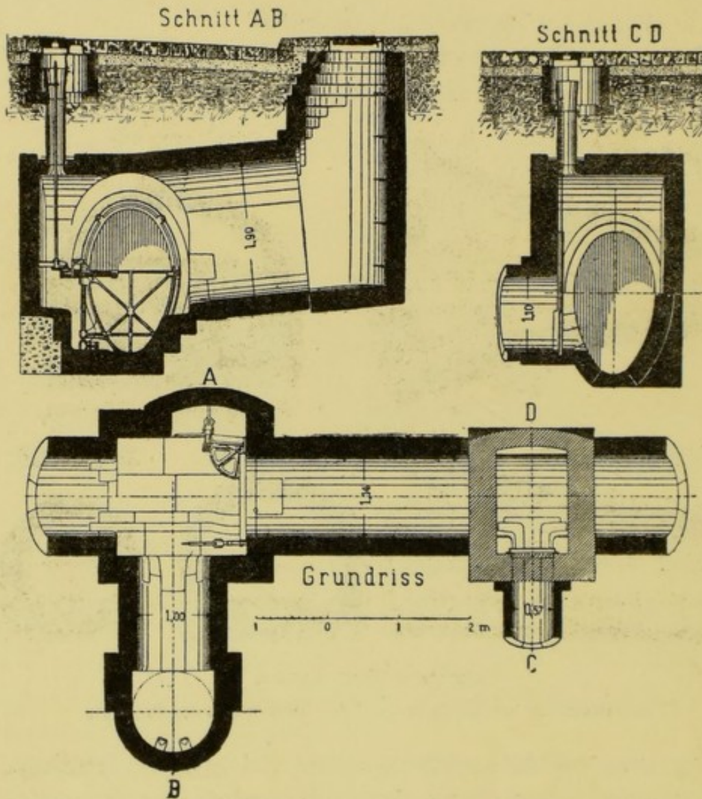
Branching-off at Right Angle and Penstock.
