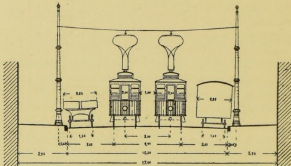
The dimensions are given in metres. One metre = 3 ft. 3 \frac{1}{2} in.
