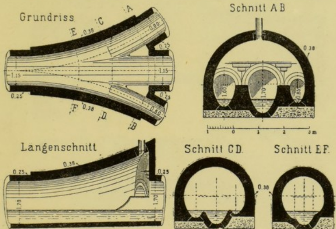
Junction of Three Sewers.
