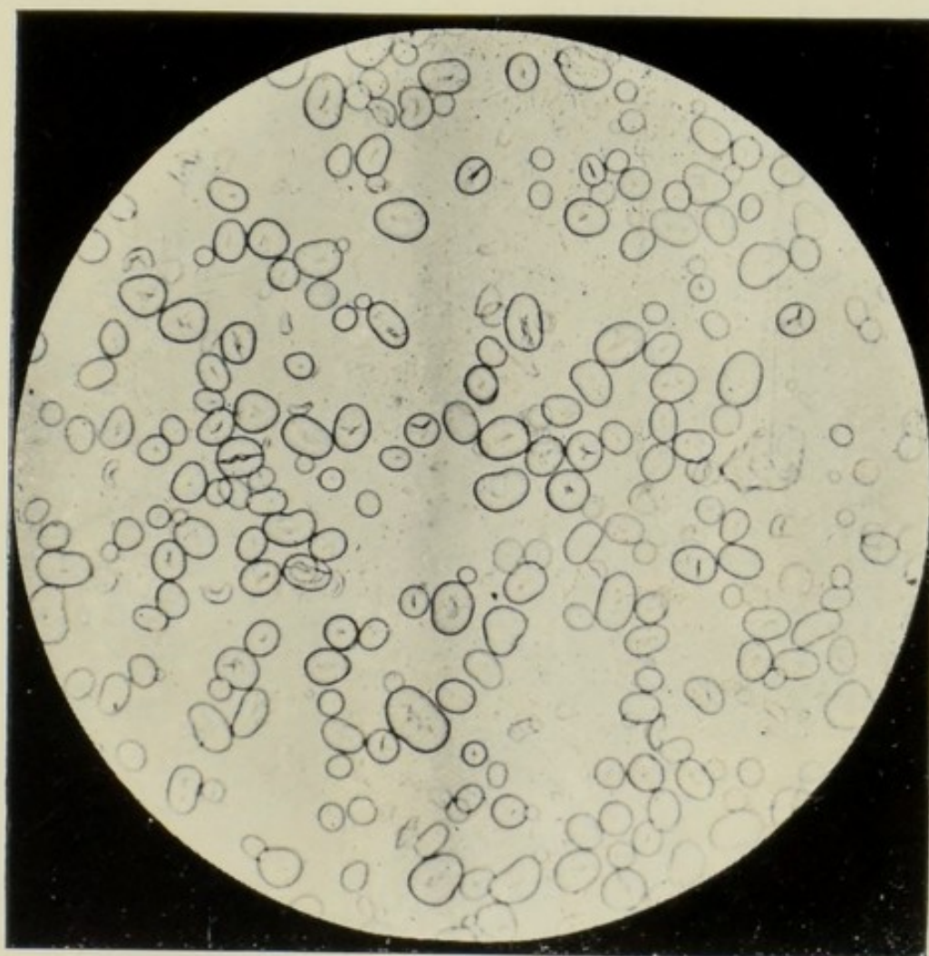
FIG. 22.—HARICOT BEAN STARCH, \times 116 .
