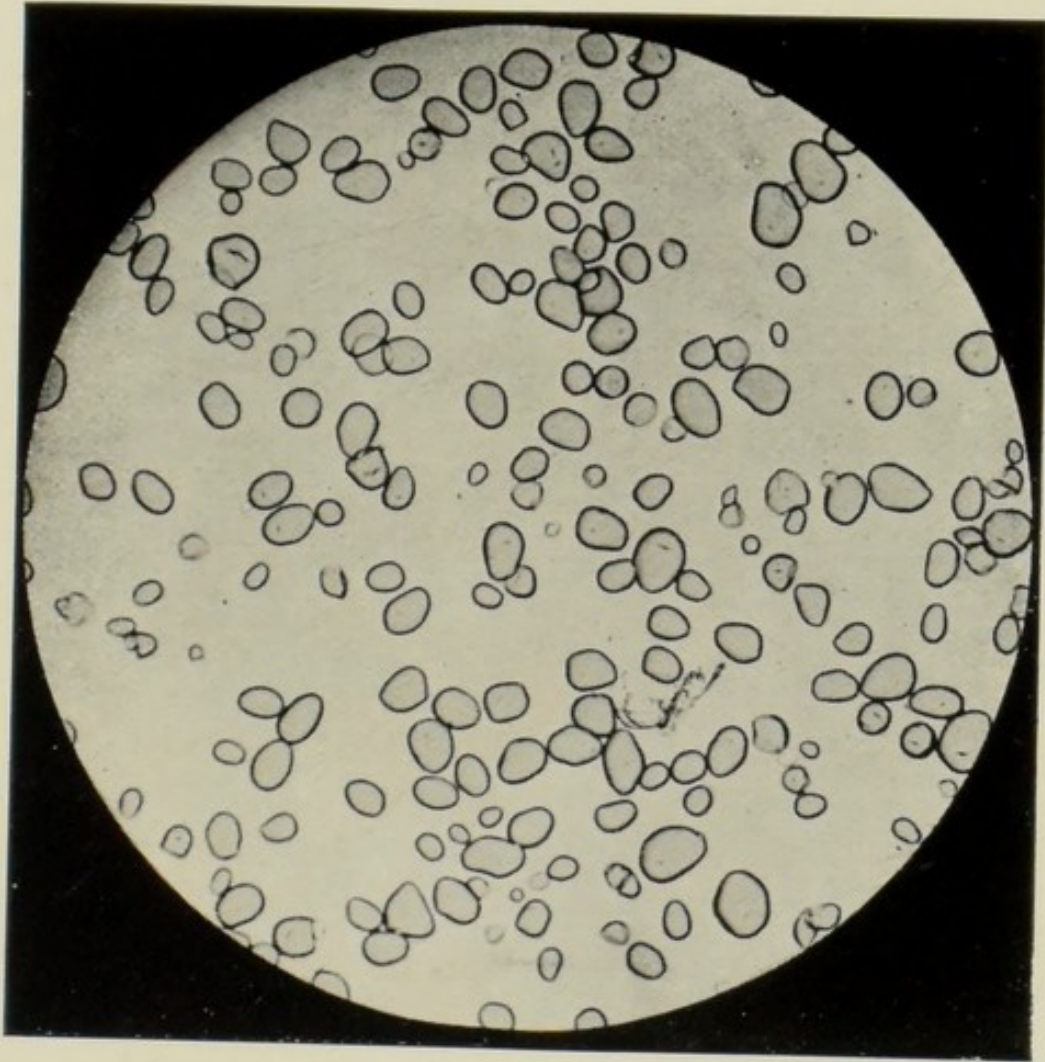
FIG. 20.—BERMUDA ARROWROOT STARCH, \times 116 .
