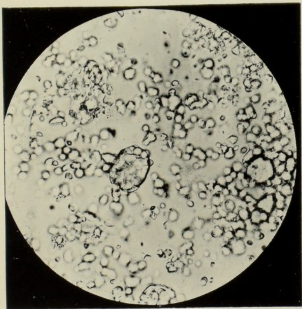
FIG. 8.—OAT STARCH, \times 380 .
