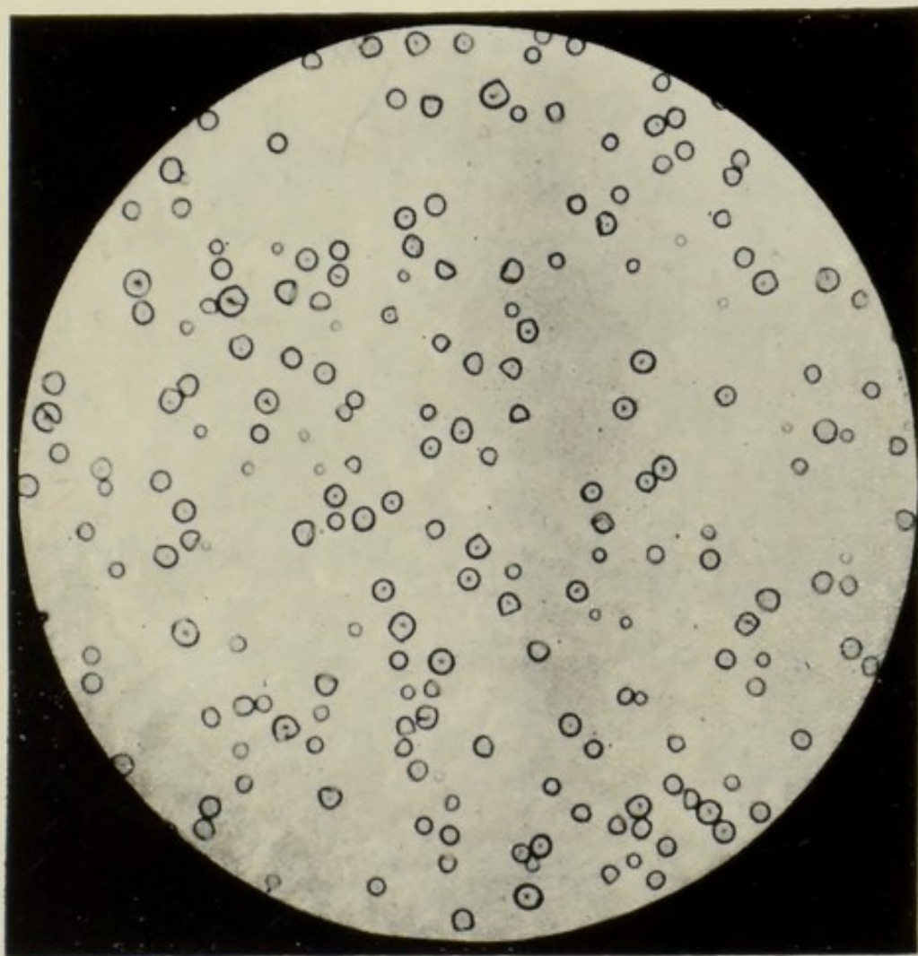
FIG. 15.—TAPIOCA STARCH, \times 116 .
