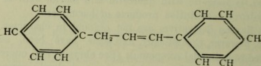
Diphenyl-1, 3-propene
