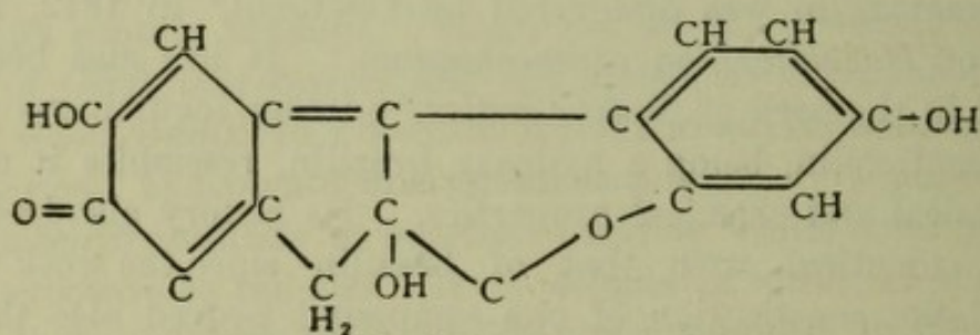
Brazilein
