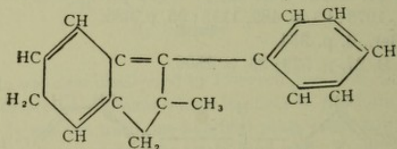
\beta -methyl- \gamma -phenyl isohydrindine
