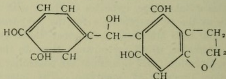
Catechin
