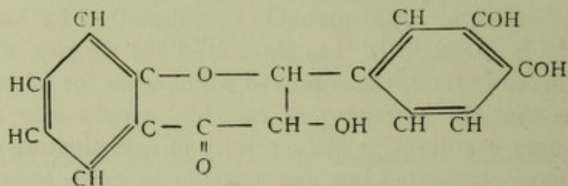
Catechin
