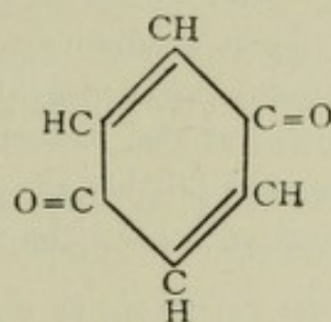
Benzo quinone
