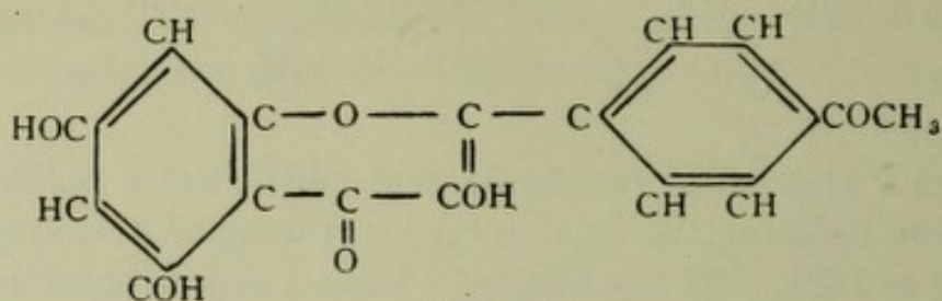
Quercetin
