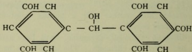
Leuco maclurin
