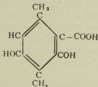
Methyl orsellinic acid
