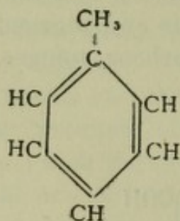
Toluene
