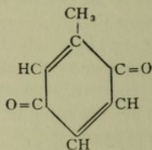
Methyl benzoquinone
