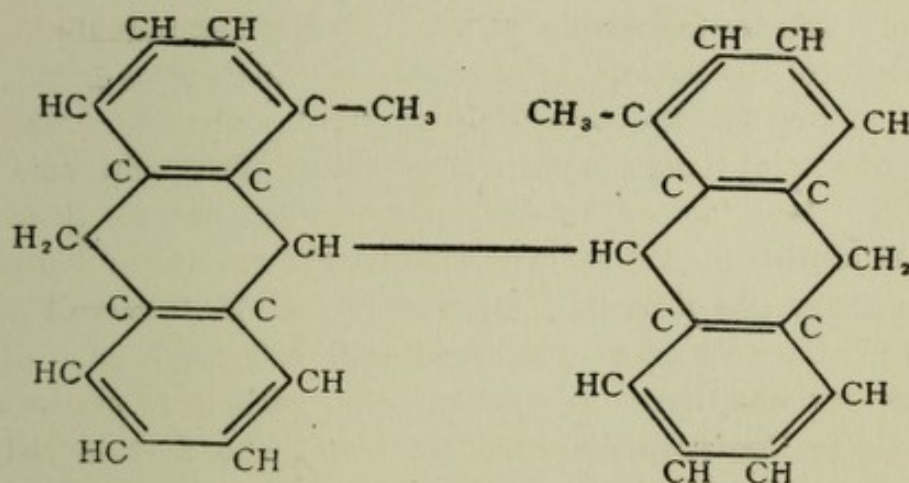
Di (methyl-dihydroanthracyl)
