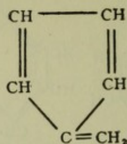
Fulvene
