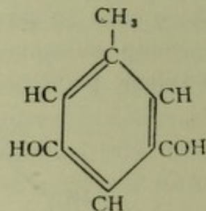
Orcinol
