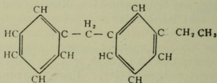
Phenyl etho phenyl methane
