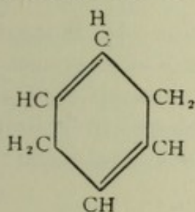
Dihydro benzene
