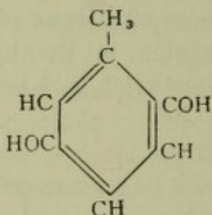
Hydrotoluquinone or Methyl hydrobenzoquinone or Methyl hydroquinone
