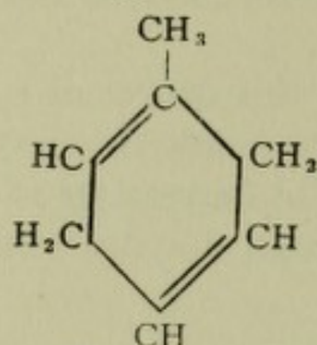
Dihydrotoluene
