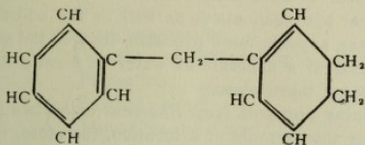
Phenyl-dihydro phenyl-methane
