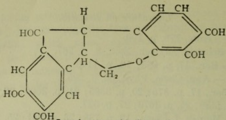
Formula suggested by Kostanecki
