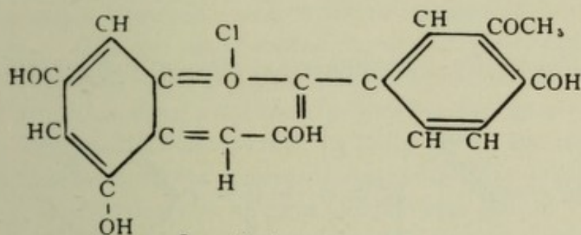
Paeonidin hydrochloride
