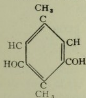
Methyl orcinol
