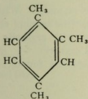
Trimethyl 1, 2, 4, benzene
