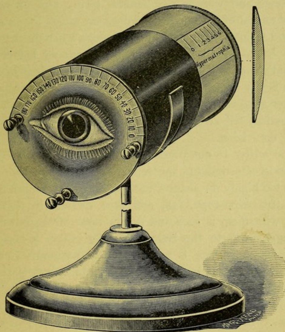
FIG. 1.—THE AUTHOR'S SCHEMATIC EYE FOR STUDYING RETINOSCOPY. (For description, see chap. vi.)
