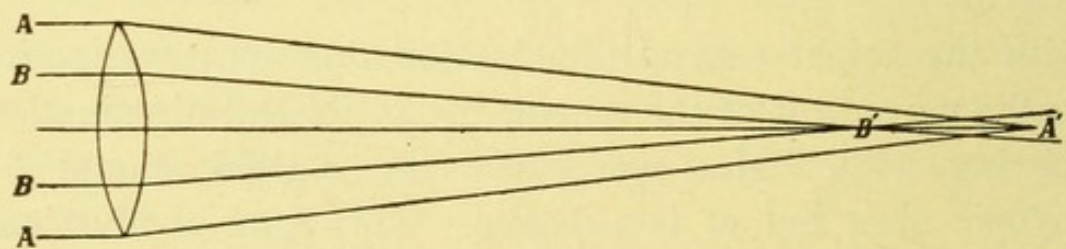
FIG. 47.—NEGATIVE ABERRATION.
