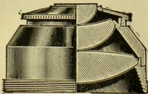
Abbe's Condenser.
