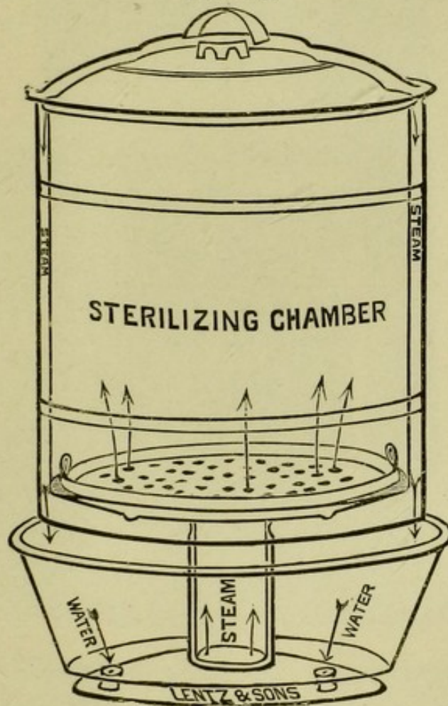
Arnold's Steam-sterilizer.
