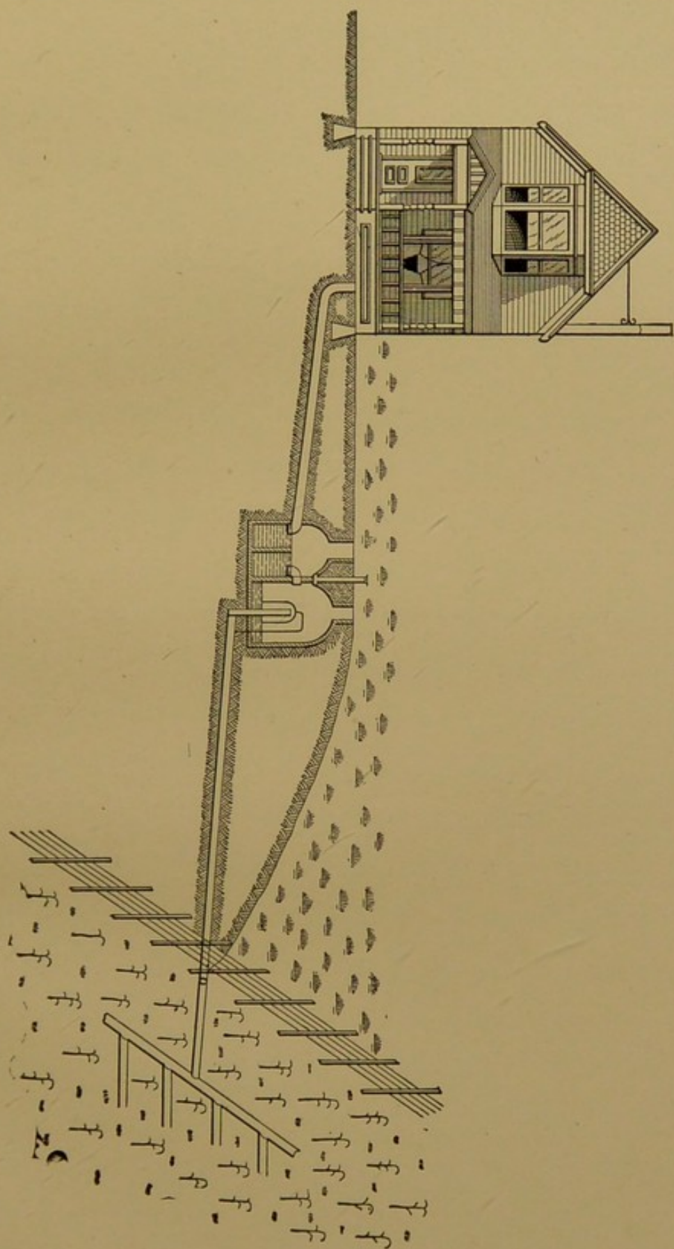
FIG. 5.—A METHOD OF SEWAGE DISPOSAL FOR AN ISOLATED HOUSE.
