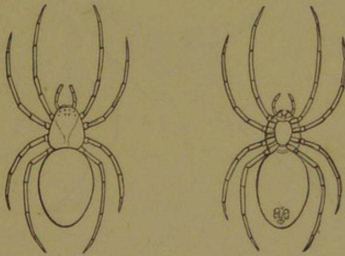
ARACHNIDE.
