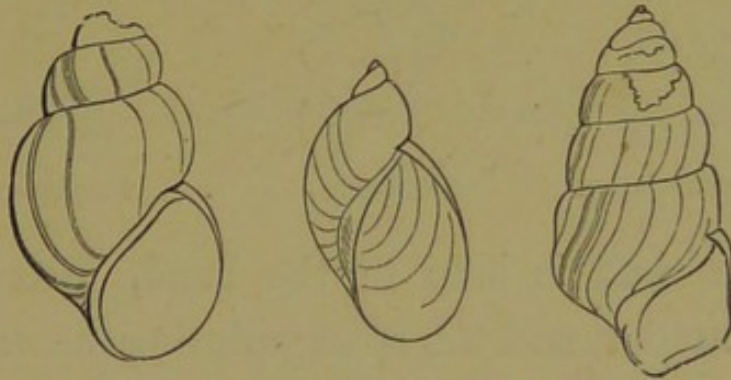
FIG. 3.—FRESH-WATER SNAIL-SHELLS.
