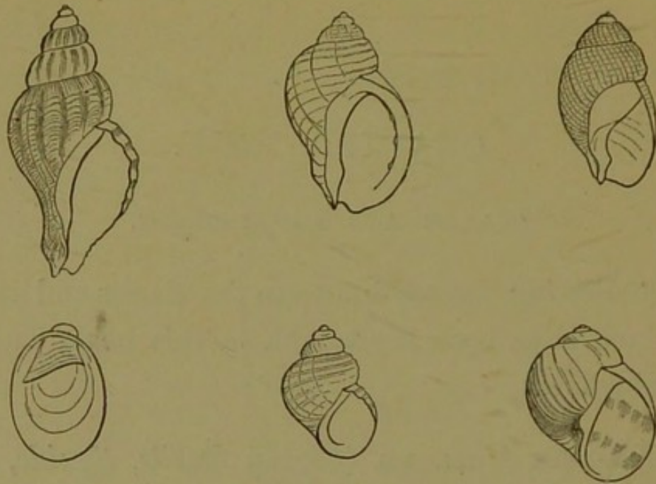
GASTEROPODS.
