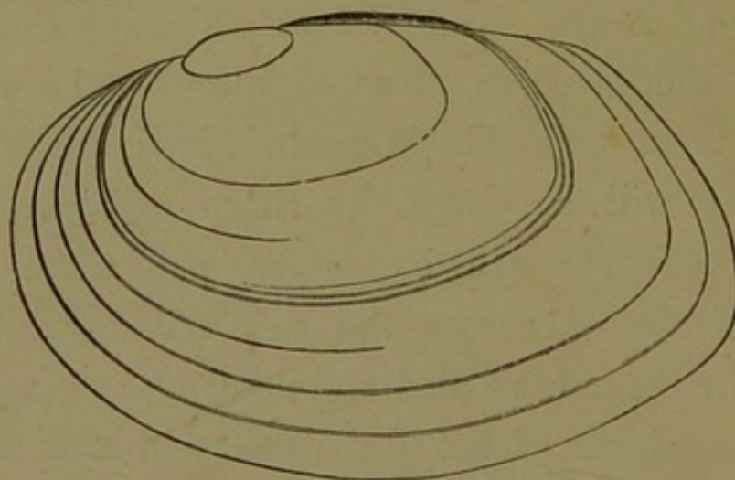
FIG. 2.—FRESH-WATER MUSSEL-SHELL.
