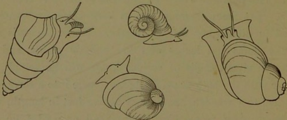
FIG. 12.—FRESH-WATER SNAILS.
