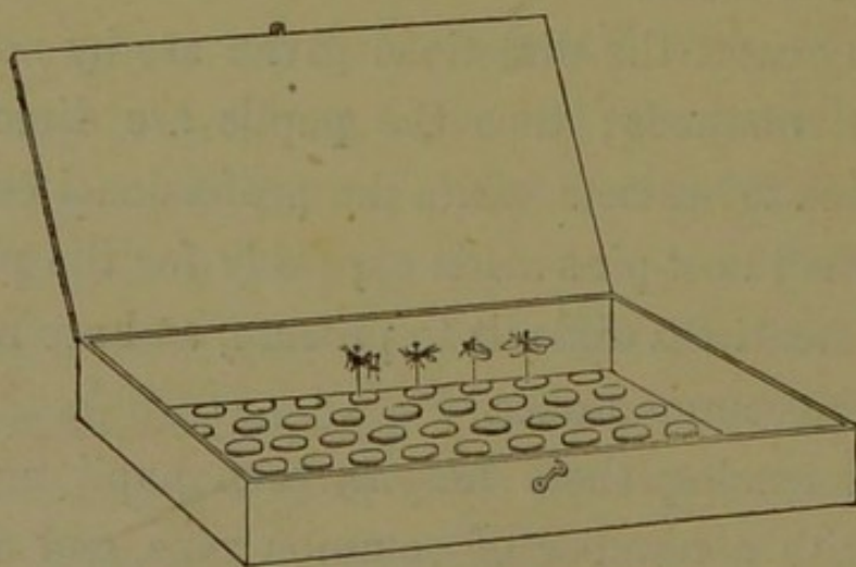
FIG. 50.—INSECT-BOX.
