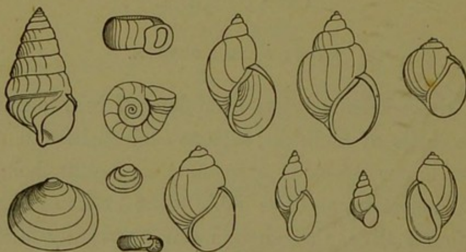
FIG. 1.—FRESH-WATER SHELLS.
