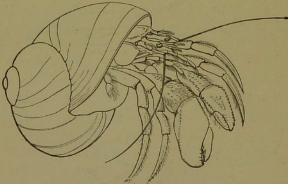
CRUSTACEANS.
