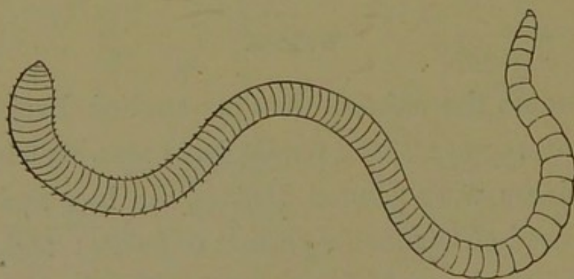
FIG. 142.—COMMON EARTHWORM.
