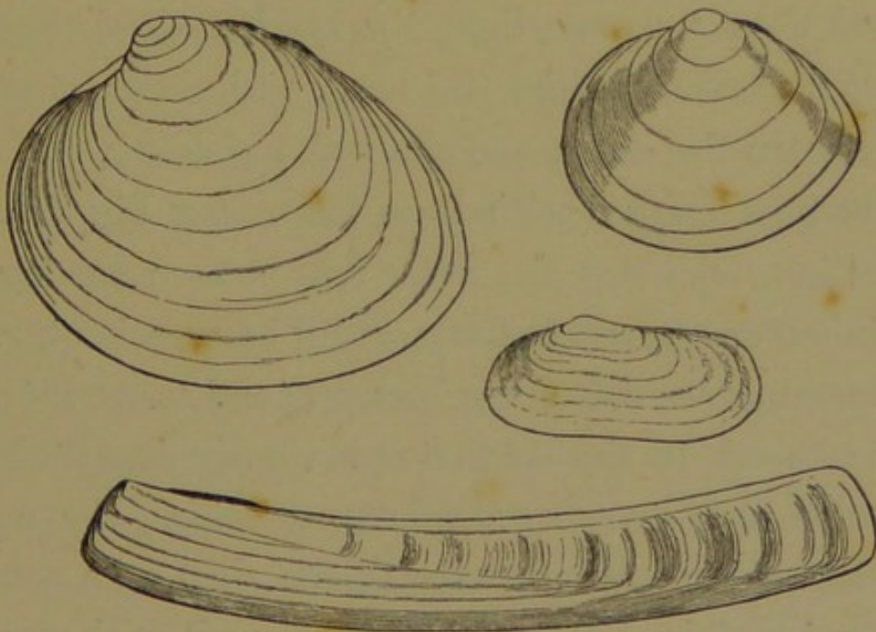
FIG. 40.—SALT-WATER BIVALVES.
