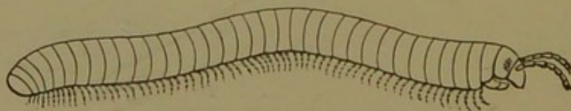
A MYRIAPOD.
