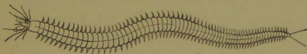
FIG. 83.—MARINE WORM.
