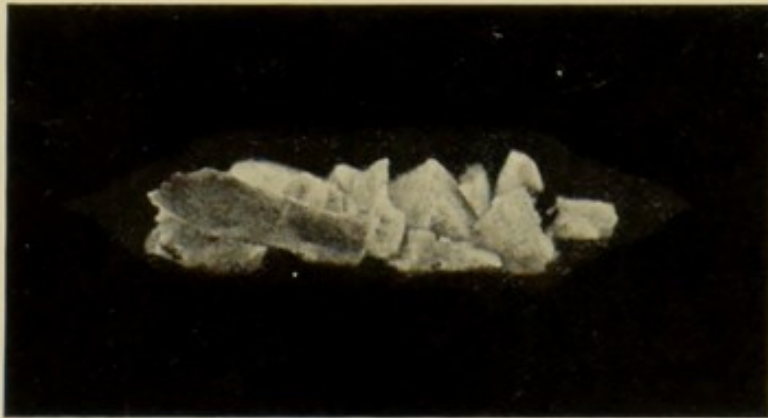
FIG. 18. The same tube photographed in the dark by its own phosphorescent light.
