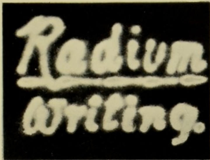
FIG. 6. Written by Radium in the Dark.
