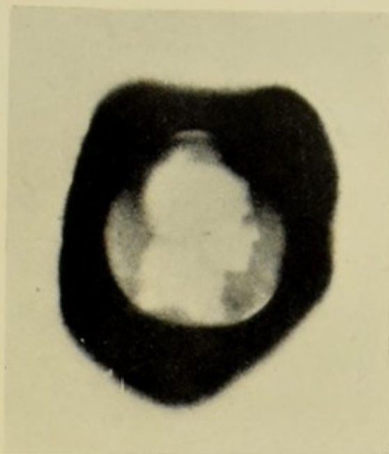
FIG. 1. Becquerel's Uranium Picture.
