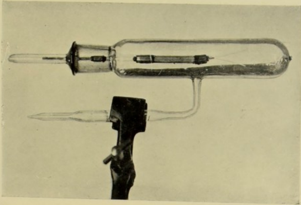
FIG. 16. Professor Strutt's "Radium Clock."
