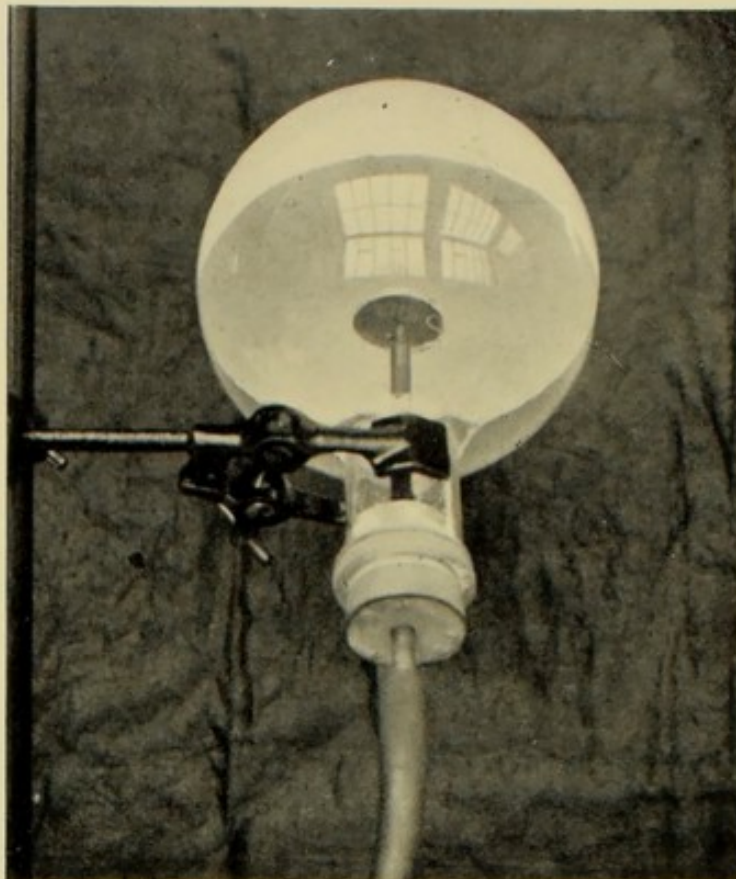
FIG. 9. Apparatus to show Absorption of \alpha -Rays by Air.
