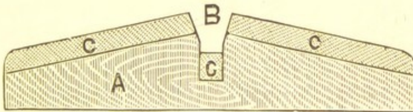
FIG. 47.—SECTION OF "SETTING" BOARD.
