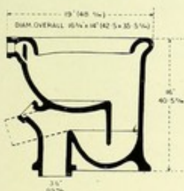
"SUPERBUS" BOXED OUTLET SECTION. Depth of Seal, about 1\frac{1}{4} in. (4.5 c/m.).
