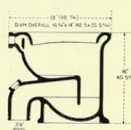
"SUPERBUS" FREE OUTLET SECTION. Depth of Seal, about 1\frac{1}{4} in. (4.5 c/m.).
