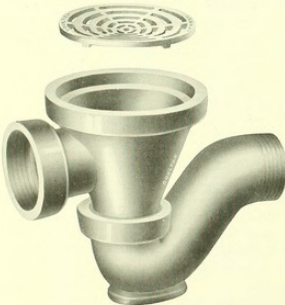
Fig. 147—REVERSIBLE GULLY. With horizontal inlet.
