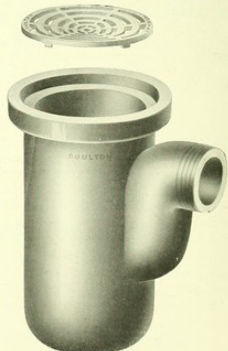
Fig. 81—YARD GULLY.
