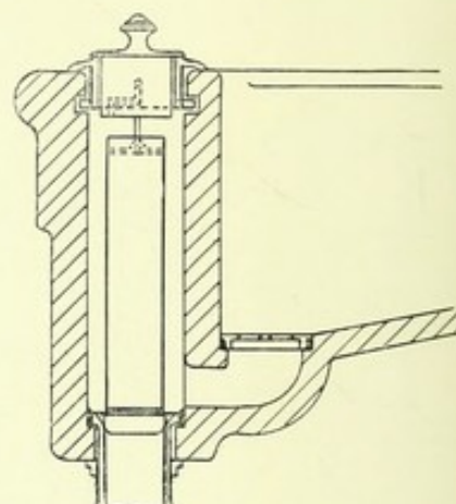
SECTION OF WASTE.
