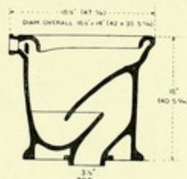
SECTION CENTRE OUTLET. Depth of Seal, about 1\frac{1}{4} in. (4.5 c/m.).
