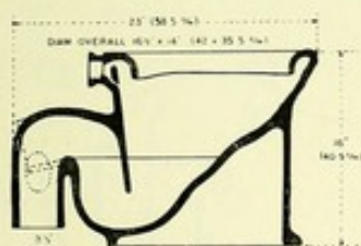
SECTION (S) AND (P) TRAP. Depth of Seal, about 1\frac{1}{4} in. (4.5 c/m.).
