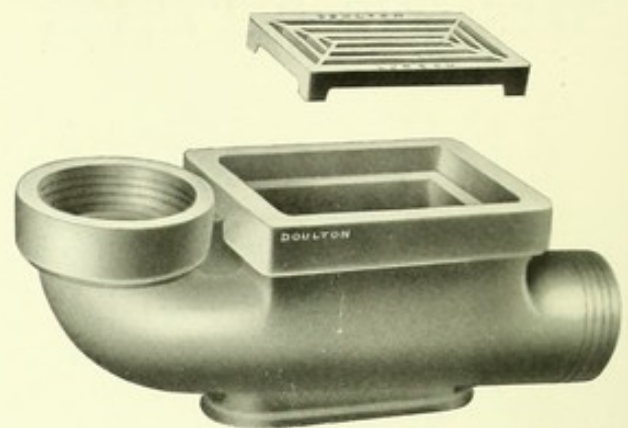
Fig. 94—RAIN-WATER SHOE. Supplied also with air-tight cover.
