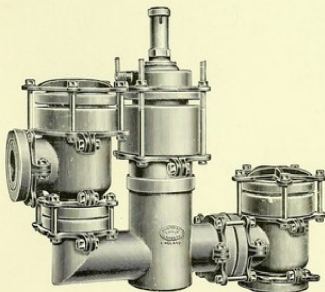
STONEWARE ACID PUMP.
