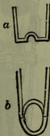
Fig. 156.—( a. ) Staple ending. ( b. ) Ring ending for Thomas's Knee-splint ( after Thomas ).
