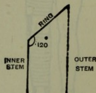
Fig. 155. — Angle of Ring on Stems.
