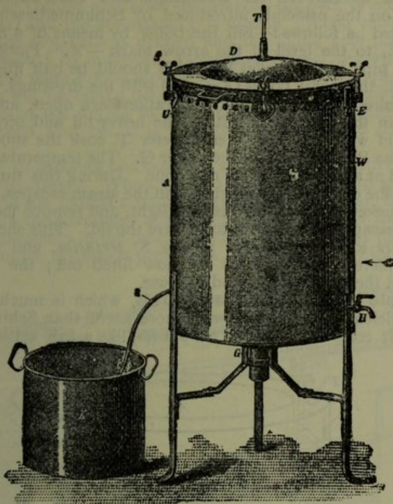
Fig. 197.—Schimmelbusch's Steam Steriliser.
