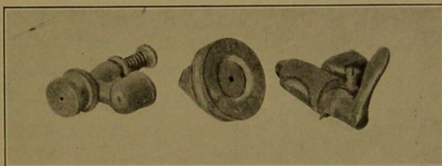
FIG. 65. —Types of nozzles. On the left, the vermores; in the center, the disk type; on the right the Bordeaux. Original.
