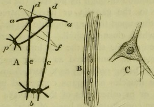
Fig. 25.—Nervous System of Mussel: A, distribution of nerves; a, a , nerves from cephalic ganglia, c , passing to mantle; b, b , branchial ganglia; d, d , nerves to anterior adductor muscle; e, e , commissural cords connecting cephalic and branchial ganglia; f , cords connecting cephalic and pedal ganglia, p . B, nerve fibre of anodon, shewing contained granules. C, ganglionic or nerve corpuscle with nucleus, and giving off branches.
